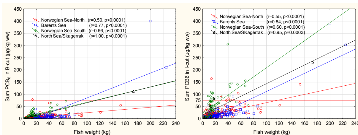
Figure 24. Correlation between concentration of sum PCB 6 in B-cut (left) and I-cut (right) and weight of Atlantic halibut from different geographical areas. The red horizontal line indicates the EU maximum level for sum PCB 6 in fish muscle.
