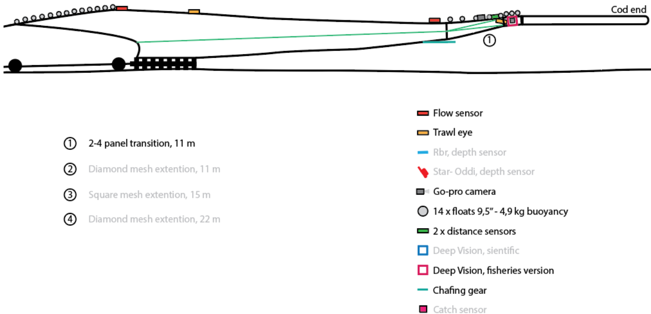
Figure 7. Selstad trawl with Deep Vision, fishery version and instrumentation. Equipment labelled in grey was not mounted to the trawl.
