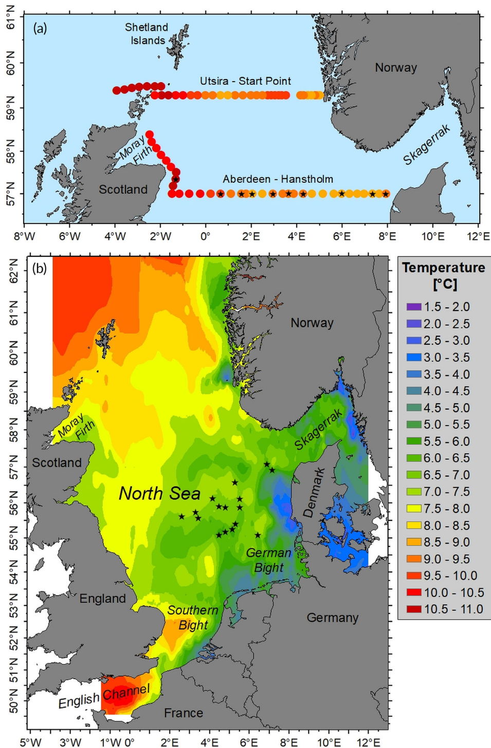
FIGURE 2 Temperature ( ^{\circ}\text{C} ) at 10 m depth in the North Sea (a) at survey stations in November/December 2016 and (b) as contours in January–March 2017. Stars show location of samples that were selected for analysis of larvae
