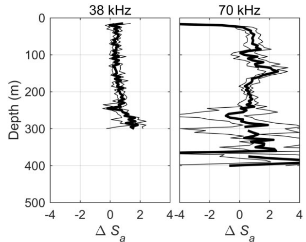
Figure 6. Variation with depth (solid thick line) of the median of the difference (EK60–EK80) in cell S_a (dB re 1 \text{ m}^2 \text{ m}^{-2} ) values for the November 2017 G.O. Sars EK60 to EK80 datasets where channel crosstalk was prevented by only operating one EK60 channel at a time. Also shown are the 25% and 75% percentiles (thin black lines) of the differences.
