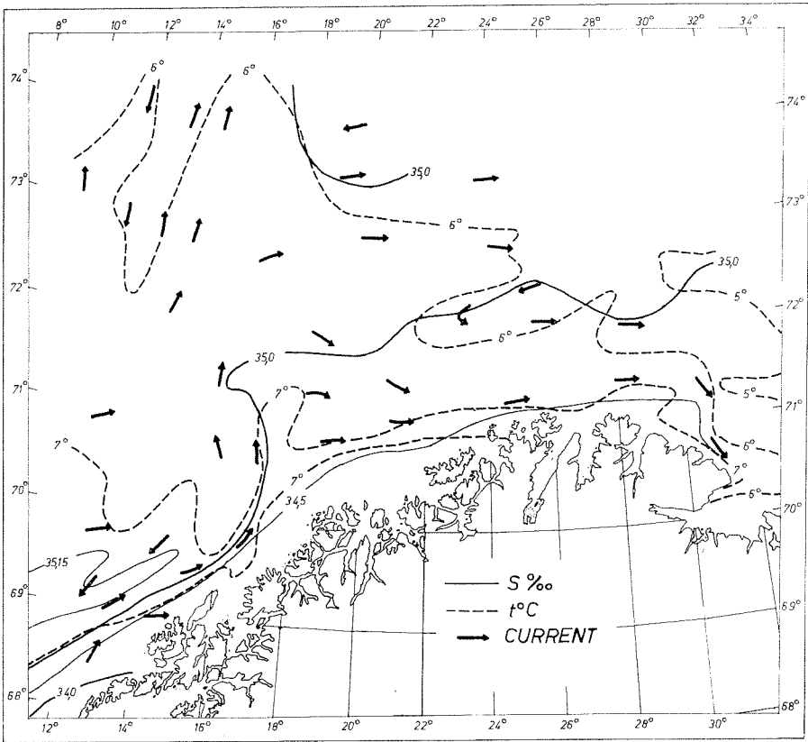
Fig. 17. Distribution of temperature and salinity at 50 m, and the main features of current system at the sea surface.
