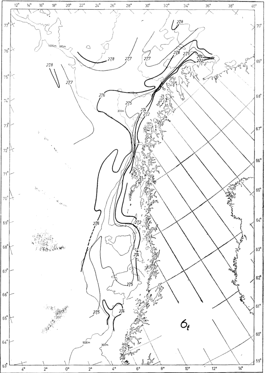
Fig. 6. C) Density at 100 m.
