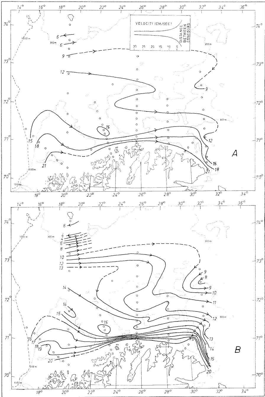
Fig. 16. A) Anomaly of dynamic height of the sea surface referred to 250 db or the bottom ( 10^3 \Delta D ). Arrows indicate direction of flow. Inset diagram shows the theoretical relation of distance between contours to the velocity. B) Volume transport between the sea surface and 250 db or the bottom of the relative current ( 10^{-1} \Delta Q ).
