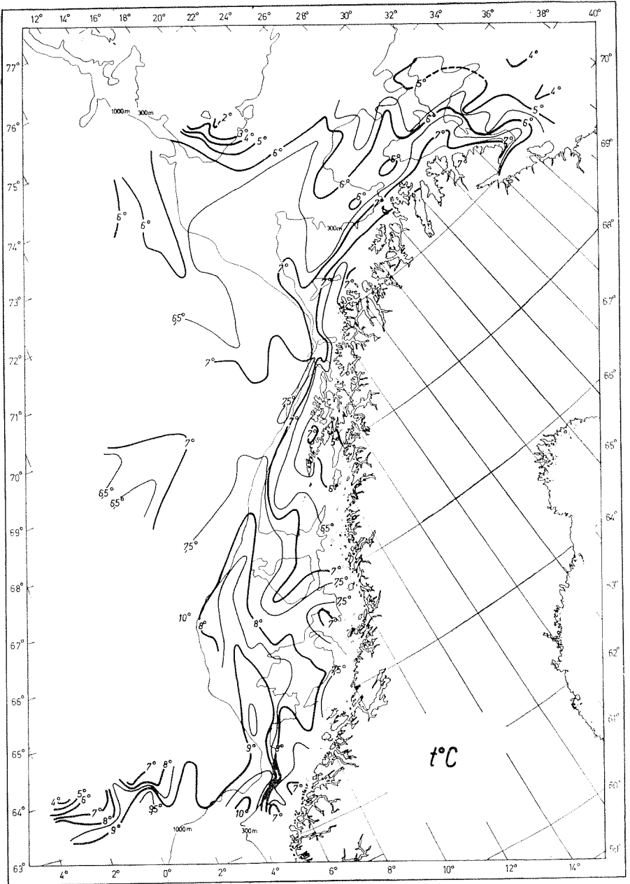
Fig. 5. A) Temperature at 50 m.
