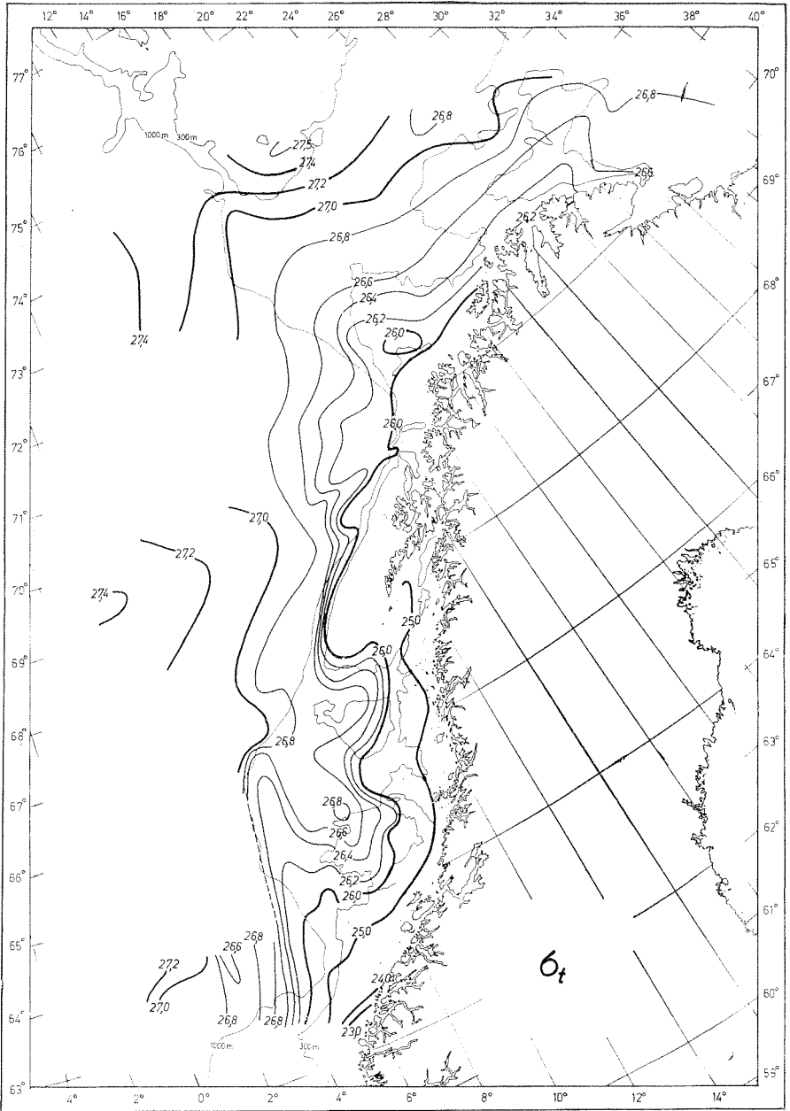
Fig. 4. C) Density at the sea surface.
