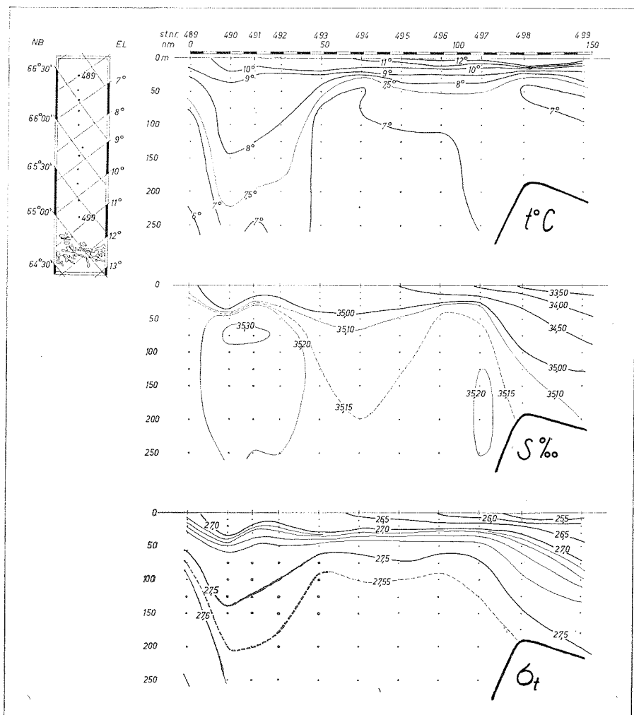
Fig. 8. Temperature, salinity and density in section across the Helgeland Plateau.
