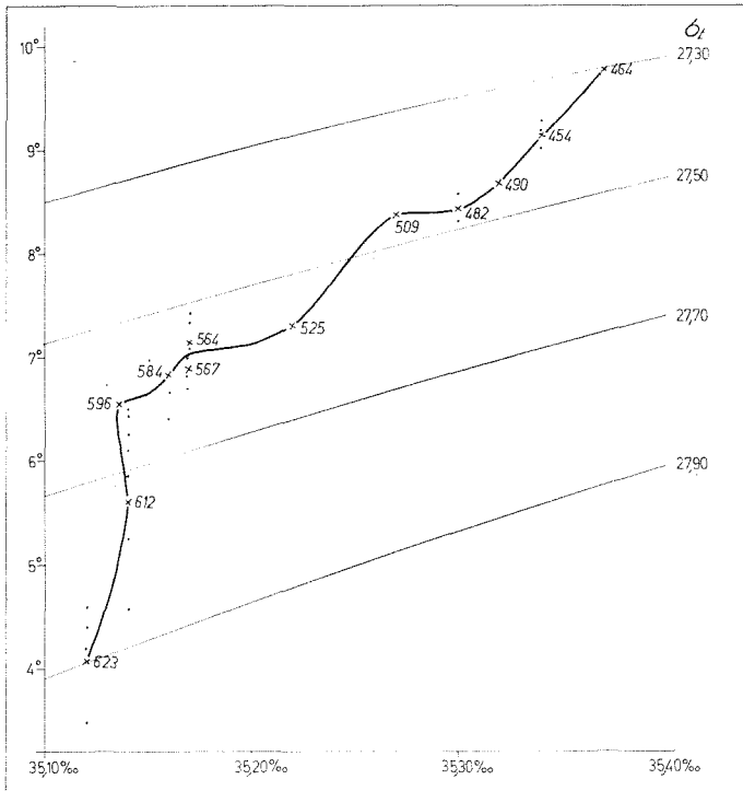
Fig. 12. t — S relation from the layer of the core of Atlantic water in the section shown in Fig. 11.
