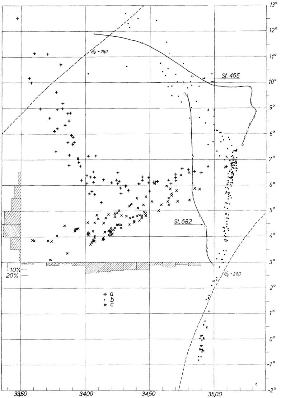
Fig. 2 a) t—S pairs of water masses inside the edge of the shelf off Lofoten and Vester-ålen. b) t—S pairs of water masses outside the edge of the same shelf. c) t—S pairs of water masses at the fixed oceanographical station off Eggum.
