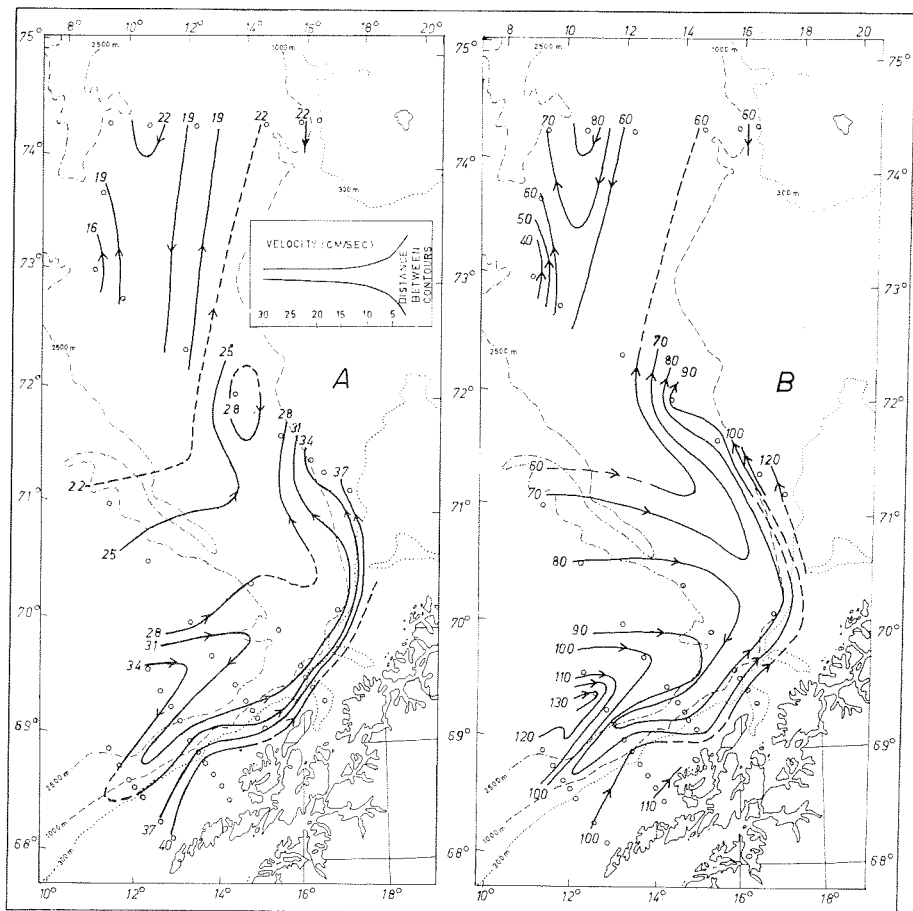
Fig. 14. A) Anomaly of dynamic height of sea surface referred to 1000 db. or bottom ( 10^2 \Delta D ). Arrows indicate direction of flow. Inset diagram shows the theoretical relation of the distance between contours to the velocity. B) Volume transport between the sea surface and 1000 m, or the bottom of the relative current ( 10^{-1} \Delta Q ).
