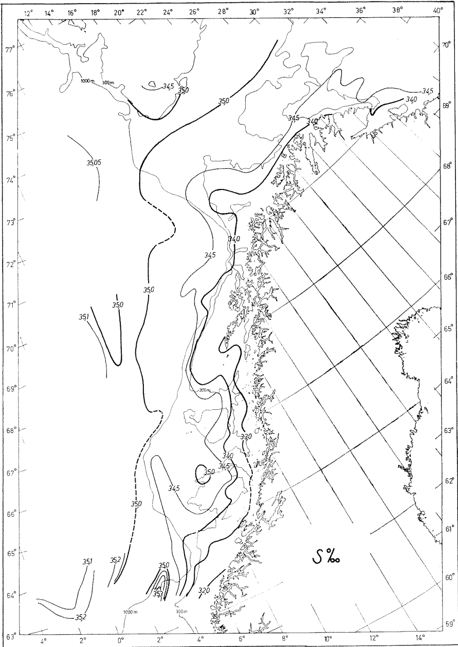
Fig. 4. B) Salinity at the sea surface.
