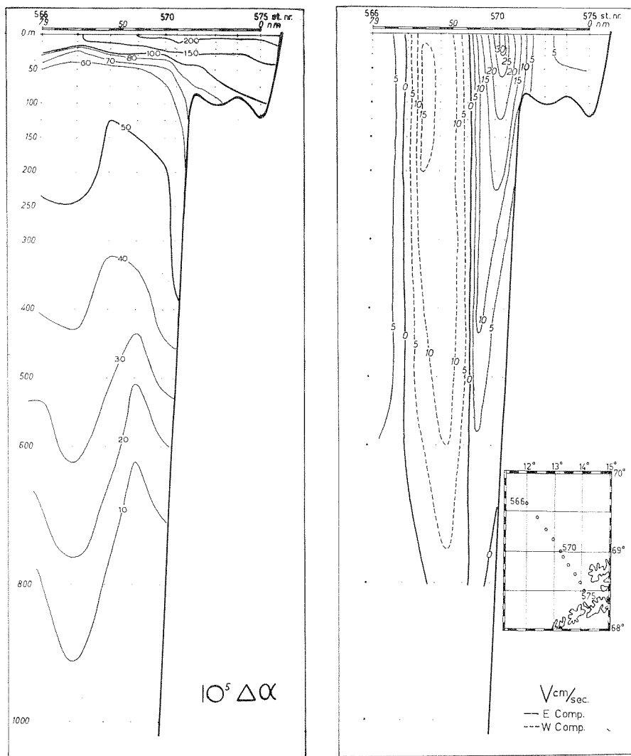
Fig. 13. Specific volume anomaly and current in the section off Vesterälven.
