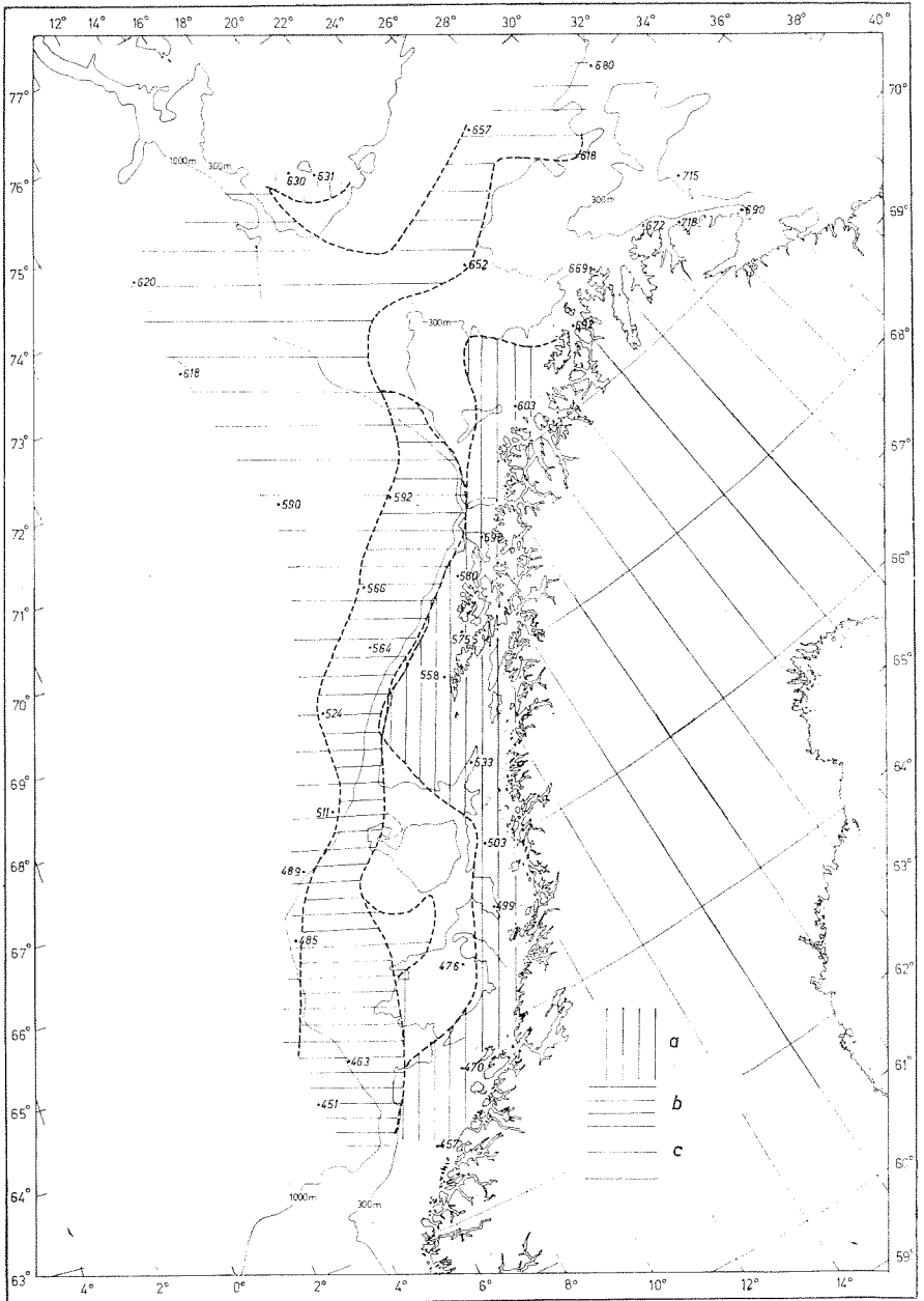
Fig. 3 a) Intermediate minimum in temperature, salinity increasing from surface to bottom or 250 m (see Fig. 2 a). b) Clearly marked intermediate maximum in salinity decreasing temperature from sea surface to the maximum depth of observation. (See Fig. 2 b). c) The same as b, the salinity maximum however being less pronounced. The first and the last station in each section are indicated by dots and a number.
