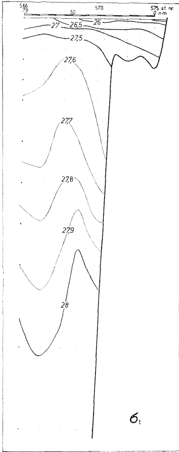
Fig. 9. C) Density in a section off Vesterålen.
