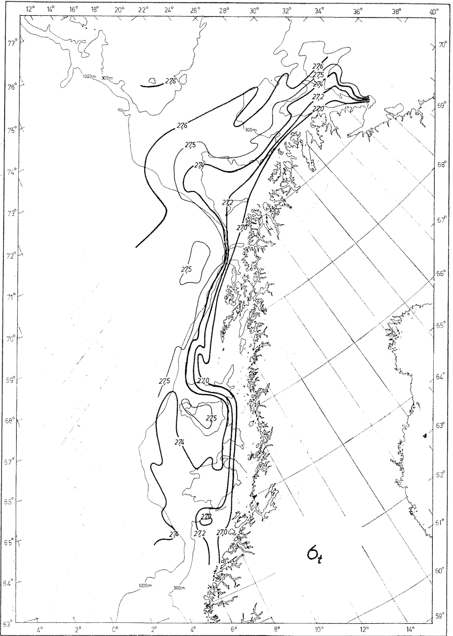
Fig. 5. C) Density at 50 m.
