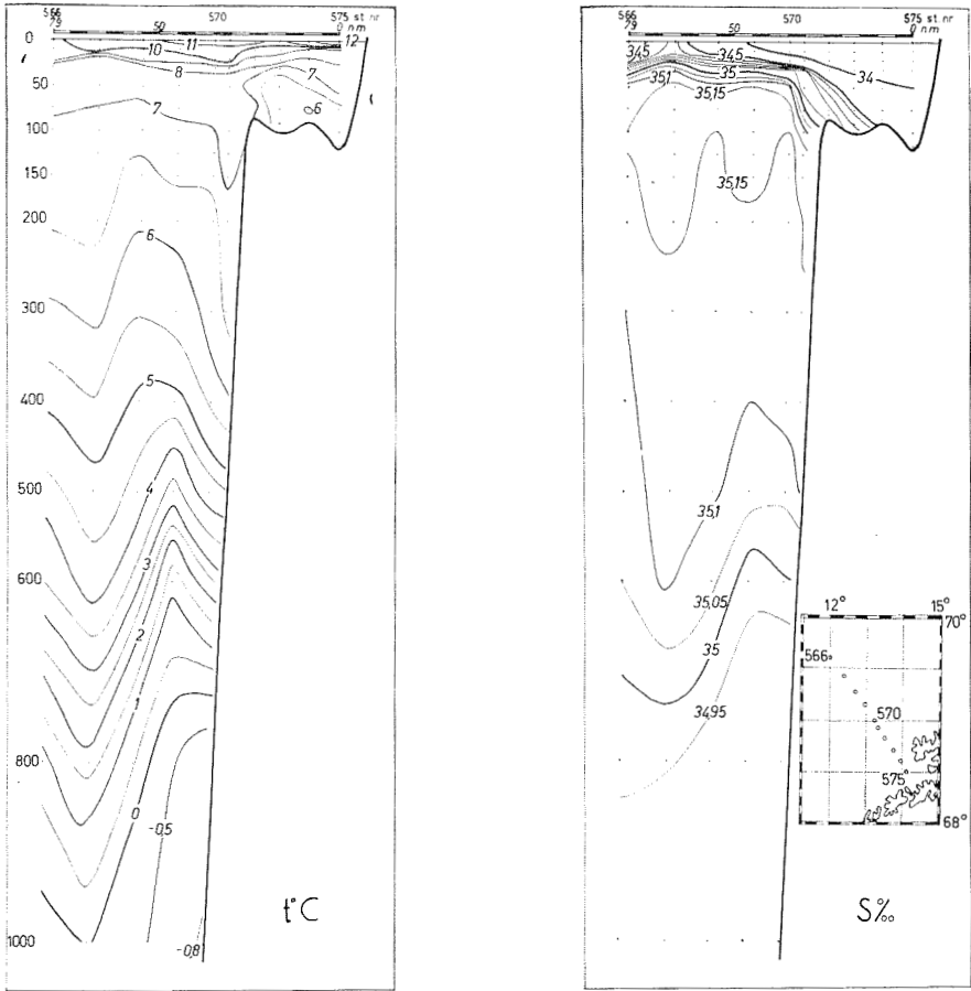
Fig. 9. A) Temperature, B) salinity in a section off Vesterålen.
