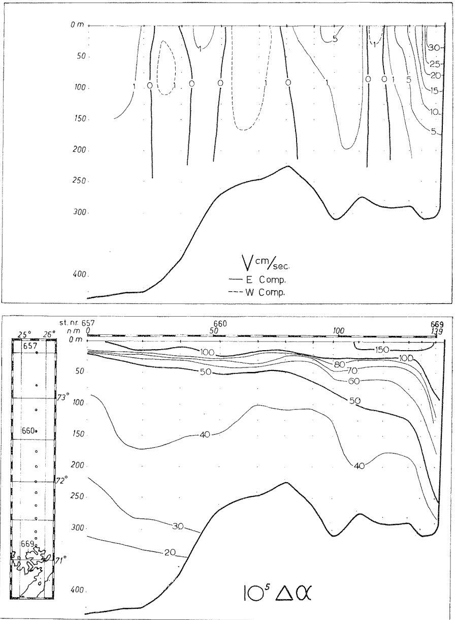
Fig. 15. Specific volume anomaly and current in the section from North Cape to the north.
