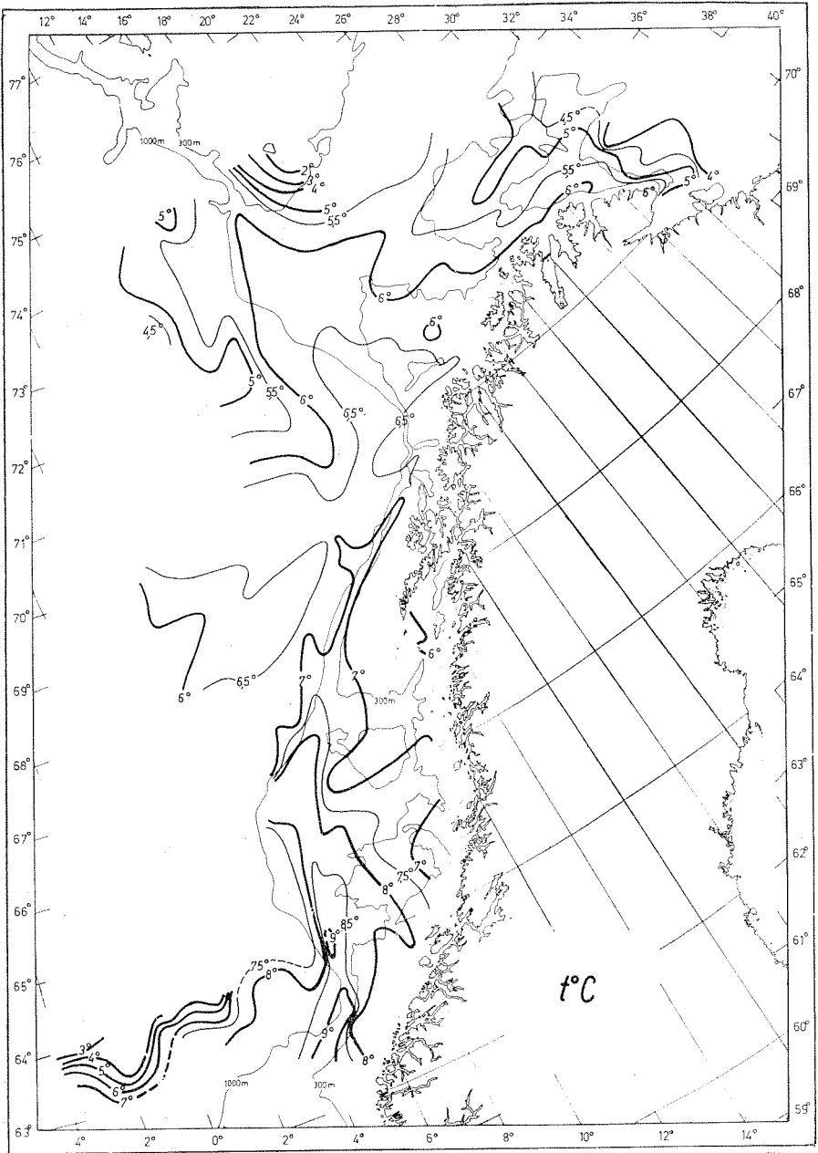
Fig. 6 A) Temperature at 100 m.
