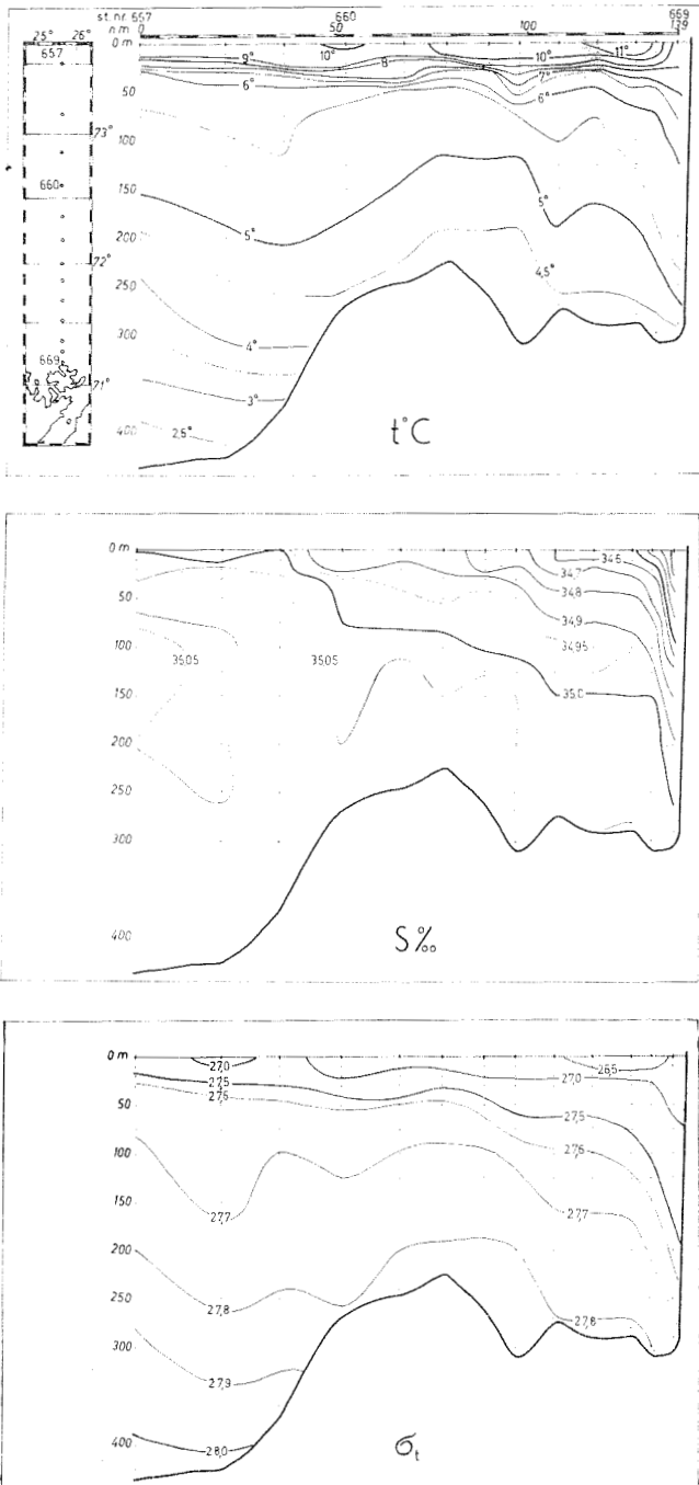
Fig. 10. Temperature, salinity and density in a section from North Cape to the north.
