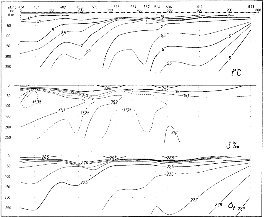
Fig. 11. Temperature, salinity and density in a section along the core of Atlantic water (maximum salinity).
