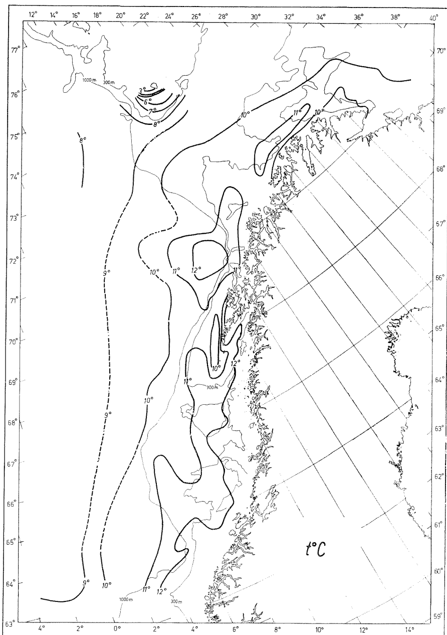
Fig. 4. A) Temperature at the sea surface.
