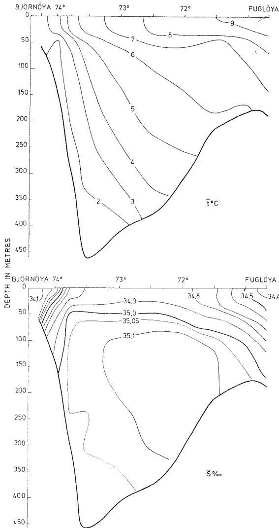
Fig. 6. Mean values of temperature, salinity and \sigma_t in the Fugløy-Bjørnøya section.
