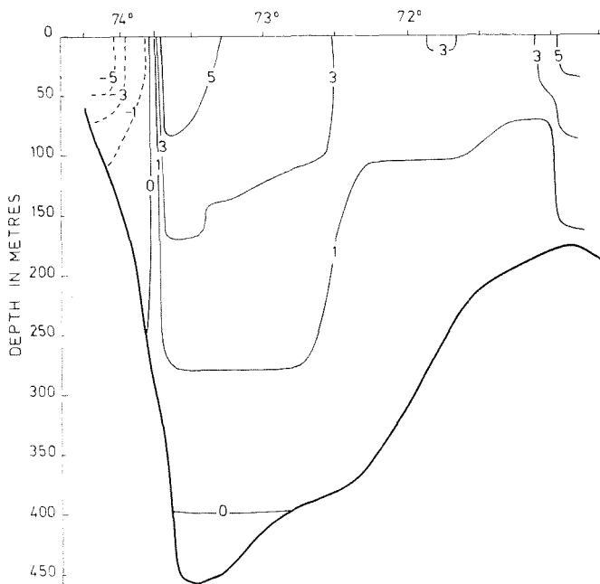
Fig. 16. Mean velocities (cm/s) computed by Helland-Hansen's formula in the Fugløya-Bjørnøya section, 1966-1977. — : Current towards east. - - -: Current towards west.
