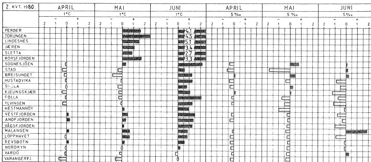
10 dagers middeltemperatur og månedsmiddel for saltholdighet langs Norskekysten i 2. kvartal 1980. [10 days mean temperature and monthly means of salinity along the Norwegian coast in 2 quarter of 1980].
