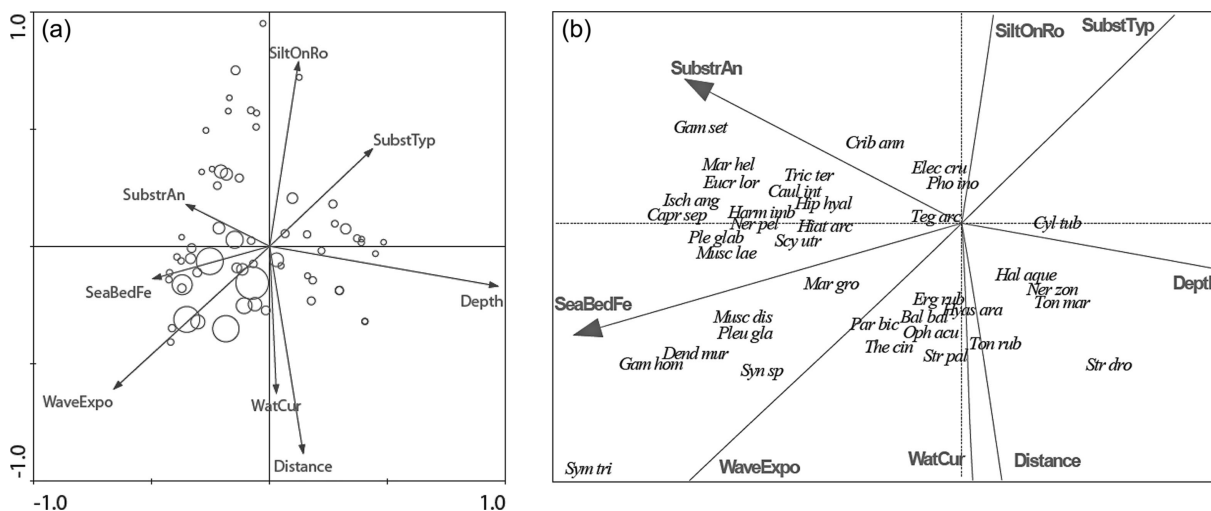
Fig. 14 Canonical correspondence analysis plots for zoobenthos on hard substrata in Kongsfjorden, Svalbard. (a) Biplot samples/factors (data on presence/absence of 403 species in samples, focus on inter-species distances, square root transformation). In (a), the size of the circles corresponds to the total biomass of each sample. Factors designations as in Table 1. (b) Biplot species/factors (data on presence/absence of 403 species in samples, focus on inter-species distances, square root transformation). The biplot is zoomed to show 38 species, which are the most widely distributed in studied habitats and (or) with the greatest abundance/biomass in samples. Species are abbreviated as follows: Balanus balanus Bal bal; Caprella septentrionalis Capr sep; Cauloramphus intermedius Caul int; Cribriolina annulata Crib ann; Cylindroporella tubulosa Cyl tub; Dendrobeania murrayana Dend mur; Electra crustulenta arctica Elec cru; Erginus rubella Erg rub; Eucratea loricata Eucr lor; Gammarellus homari Gam hom; Gammarus setosus Gam set; Haliclona aqueductus Hal aque; Harmothoe imbricata Harm imb; Hiatella arctica Hiat arc; Hippothoa hyalina Hip hyal; Hyas araneus Hyas ara; Ischyrocerus anguipes Isch ang; Margarites groenlandica var. groenlandica Mar gro; Margarites helicina Mar hel; Musculus discors Musc dis; Musculus laevigatus Musc lae; Nereis pelagica Ner pel; Nereis zonata Ner zon; Ophiopholis aculeata Oph acu; Parapleustes bicuspis Par bic; Pholoe inornata Pho ino; Pleusymtes glabroides Ple glab; Pleusymtes glaber Pleu gla; Scypha utriculus Scy utr; Strongylocentrotus droebachiensis Str dro; Strongylocentrotus pallidus Str pal; Symplectoscyphus tricuspoidatus var. acuminatus Sym tri; Synoicum sp. Syn sp; Tegella arctica Teg arc; Thelepus cinninnatus The cin; Tonicella marmorea Ton mar; Tonicella rubra Ton rub; Tricellaria ternata Tric ter.
