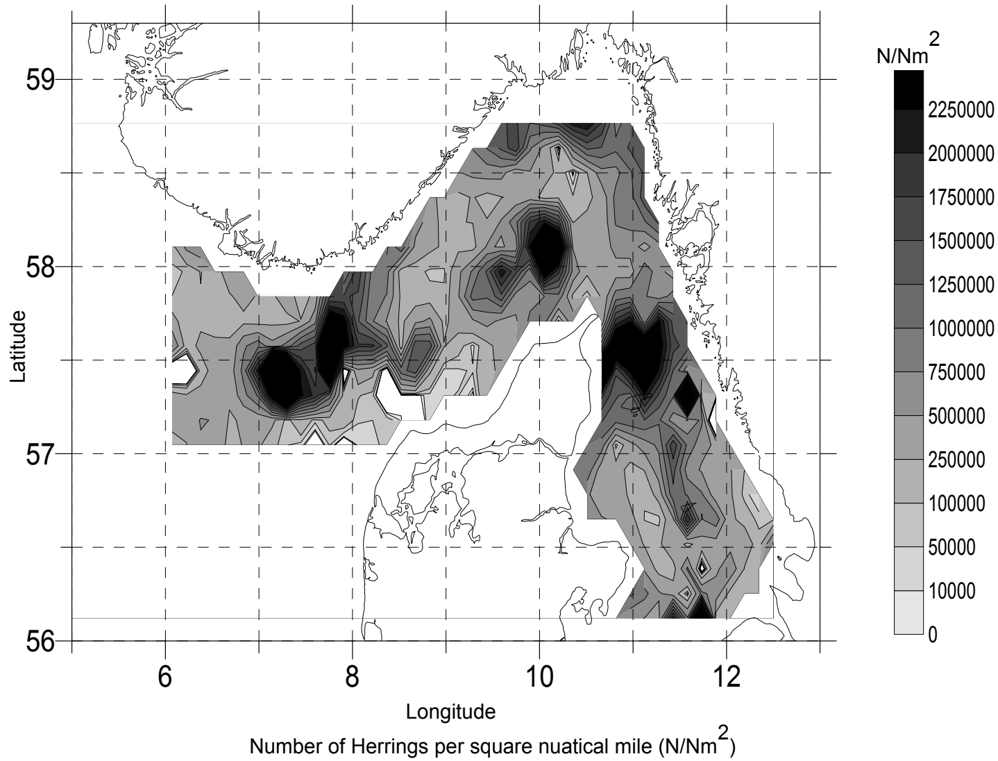
Figure IIB.5. Map of the eastern North Sea, Skagerrak and Kattegat showing contoured density of herring from the July 2002 Danish acoustic survey.
