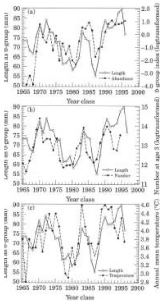
Figure 2. Temporal development in length of 0-group cod in comparison with (a) abundance as 0-group, (b) abundance at age 3, and (c) annual mean temperature in the Kola section.
