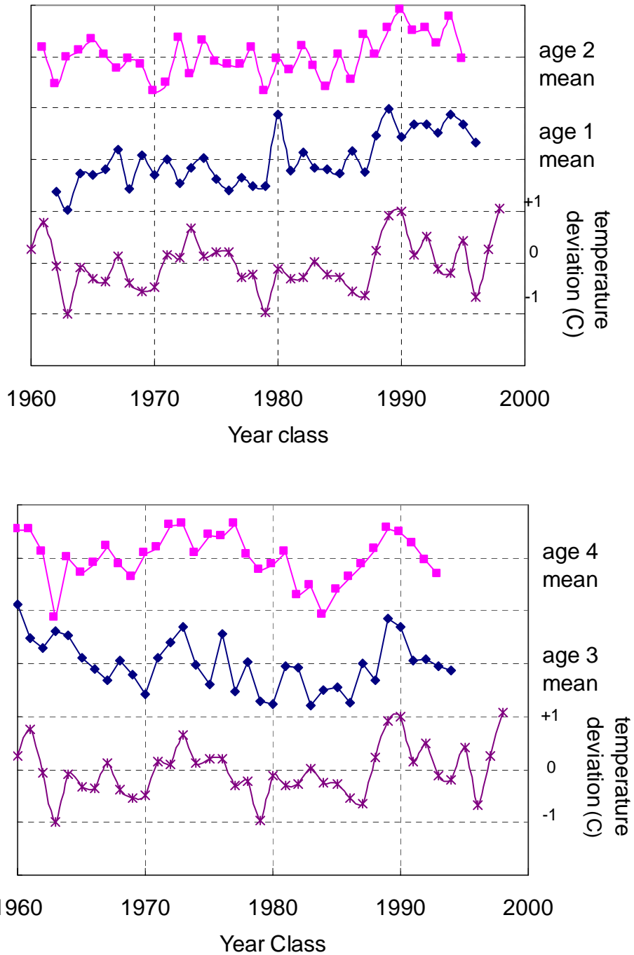
Figure 1. Deviations from the mean weight at age and mean bottom temperature for North Sea cod. The top panel shows ages 1 and 2; the bottom panel shows ages 3 and 4. The horizontal dashed lines correspond to 20% deviations from the mean weight.
