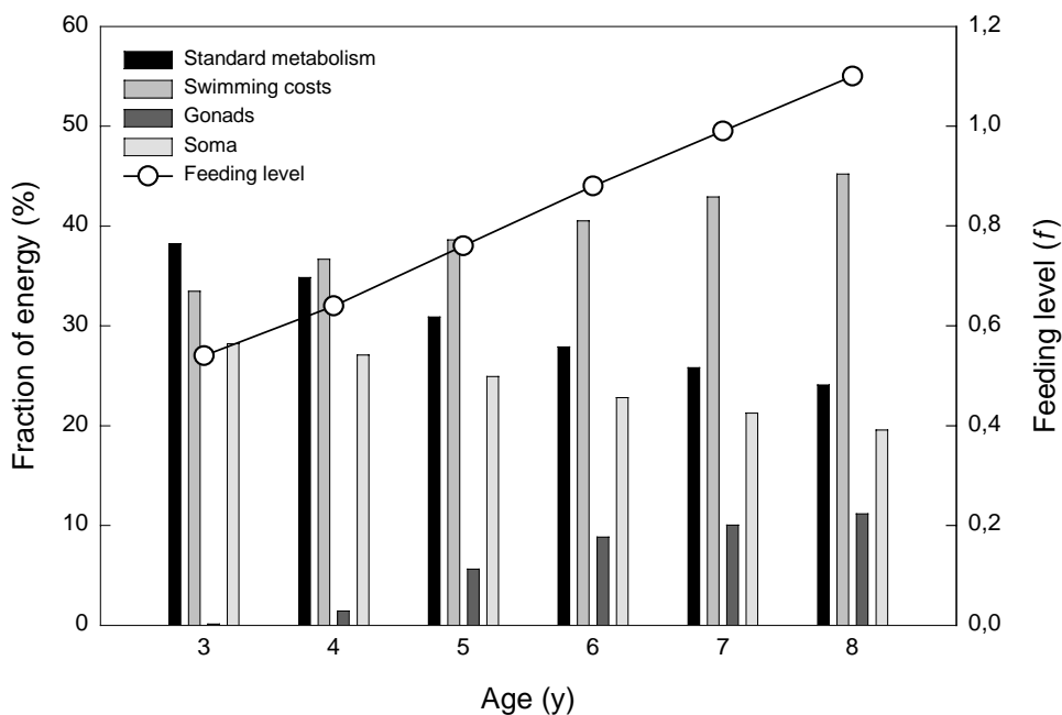
Figure 2. Feeding level and allocation of net energy in North Sea saithe by age class.
