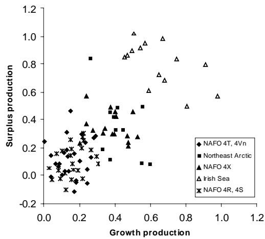
Fig. 5. Surplus production in year t+1 and growth production of survivors from year t to year t+1 on a per capita basis for 5 different cod stocks
