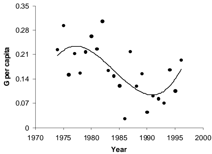
Fig. 1. Growth production on a per capita basis of cod 3 years old and older in the northern Gulf of St. Lawrence for the period 1974 -1996
