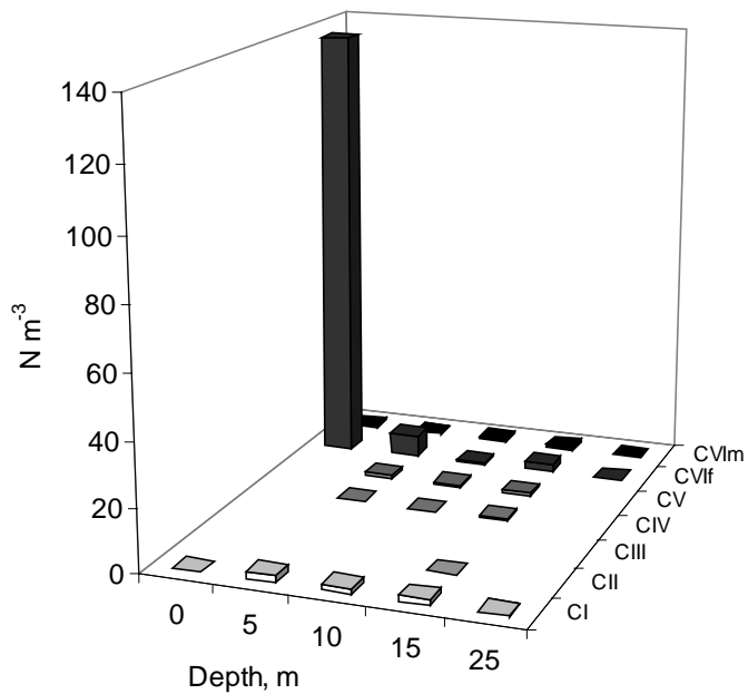
Figure 1. Depth distribution of C. finmarchicus copepodites sampled by Clarke-Bumpus closing nets at Henningsvær, Lofoten Islands 24 March 2000, at noon in bright sunshine (Skreslet and Olsen, unpubl.)
