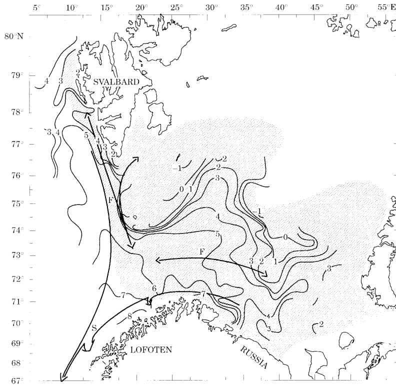
Figure 1. The Barents Sea with the area of distribution of Arcto-norwegian cod and isotherms (°C) at 100m depth. Feeding areas (hatched), seasonal feeding migrations (F) and spawning migrations are indicated (see Mehl, 1991). Temperature distribution is for August 1995 (ICES, 1996). This map is taken from Ottersen et al. (1998).
