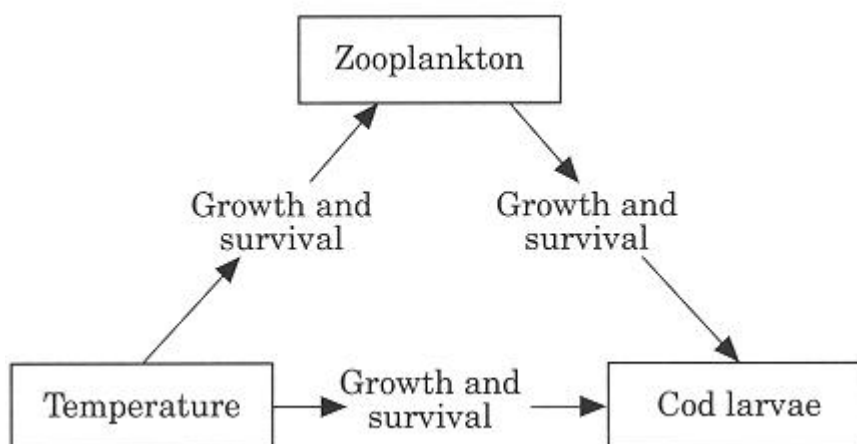
Figure 3. Mechanisms linking temperature to growth and survival
