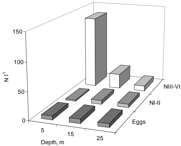
Figure. 2. Average concentration of C. finmarchicus eggs and nauplii collected in 3x2 liter water samples at Henningsvær, Lofoten Islands 14 April 2000, at noon in bright sunshine (Skreslet and Olsen, unpublished).
