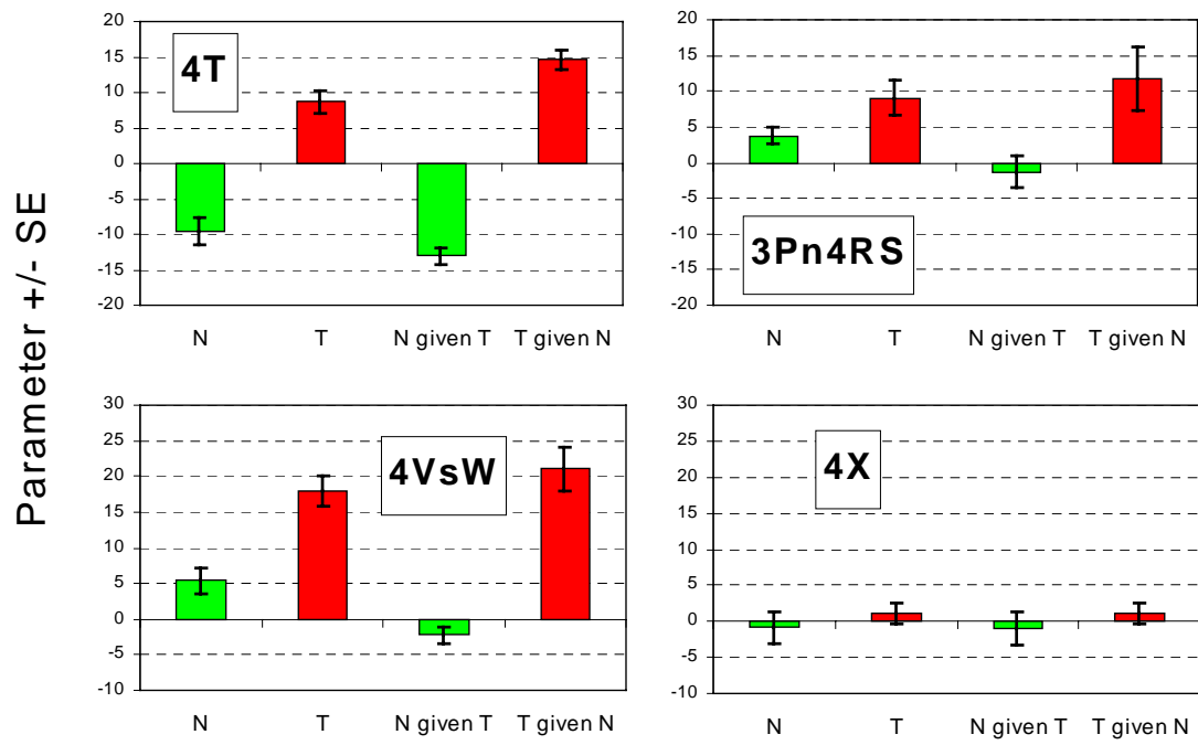
Figure 2. Effects of density (N) and environmental temperature (T) on length-at-age of cod in the Gulf of St. Lawrence (4T, 3Pn4RS) and on the Scotian Shelf (4VsW, 4X).
