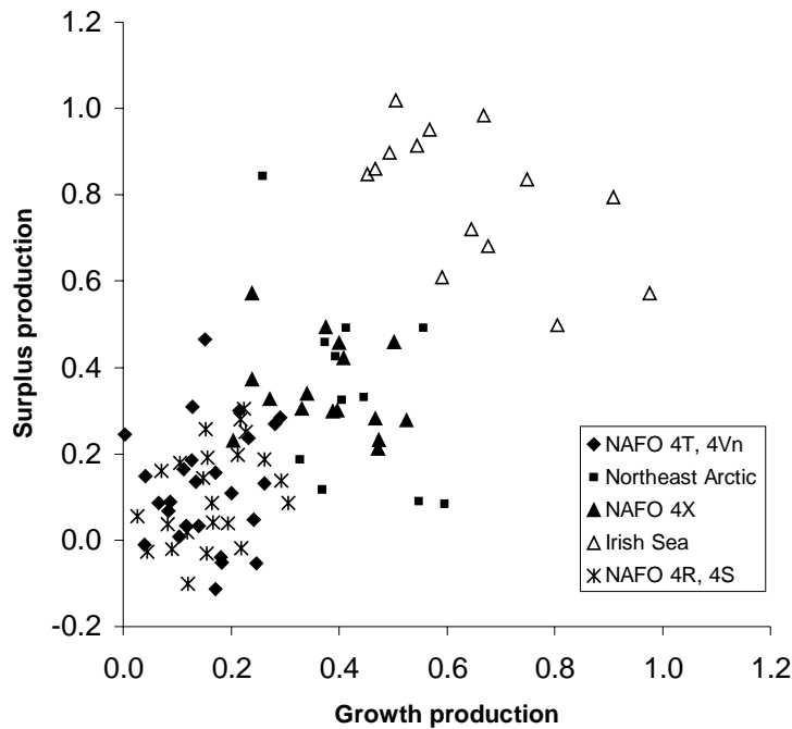
Figure 6.1. Surplus production in year t+1 and growth production of survivors from year t to year t+1 on a per capita basis for 5 different cod stocks.
