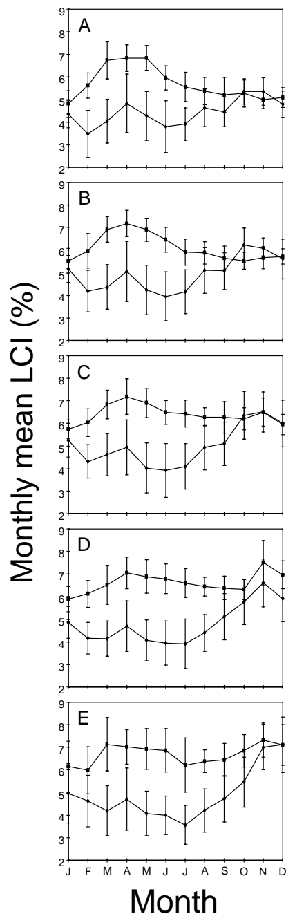
Monthly mean LCI (%) of Northeast Arctic cod for years when capelin stock biomass was less than 1 mill. tonnes(diamonds) and years when capelin stock biomass was greater than 1 mill. tonnes (squares). The 95 % confidence limits are shown.(a) 41-50 cm cod, (b) 51-60 cm cod, (c) 61-70 cm cod, (d) 71-80 cm cod, and (e) 81-90 cm cod.
