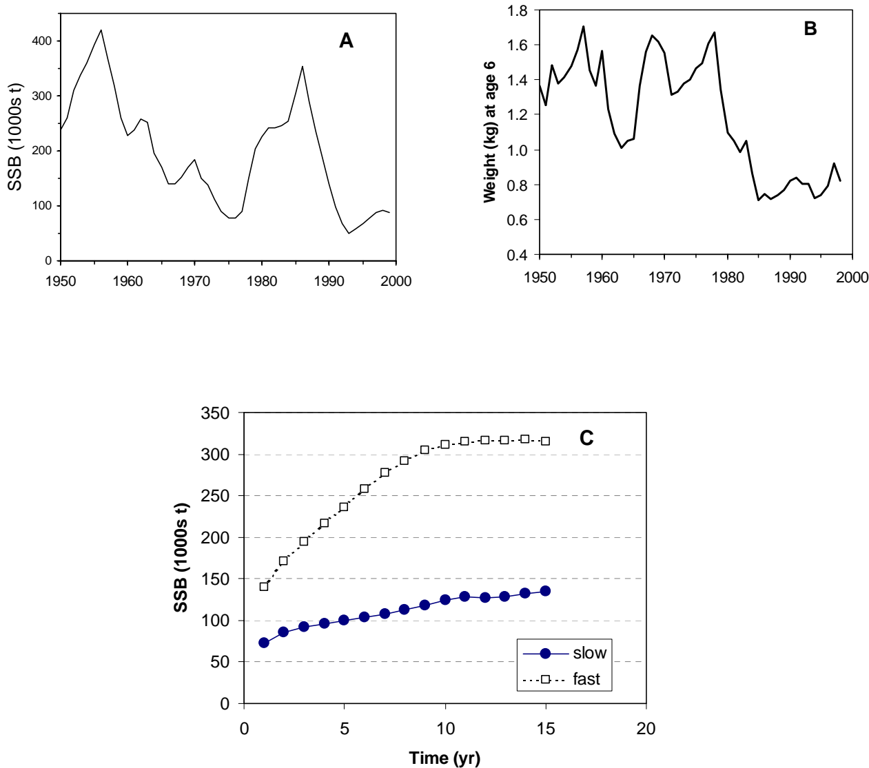
Figure 6.3. Effect of variation in growth on biomass of southern Gulf of St. Lawrence cod. A. Spawning stock biomass (SSB). B. Weight at age 6. C. Simulated recovery from stock collapse assuming either the fast growth rates of the mid 1970s or the slow growth of the early 1990s.
