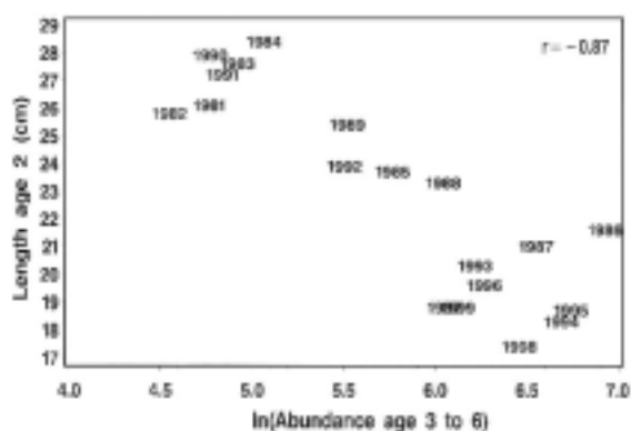
Figure 3. Abundance of agegroups 3 to 6 vs length at age 2 for Arcto-norwegian cod from 1978 until 1999. The Pearson correlation ( r ) is shown.
