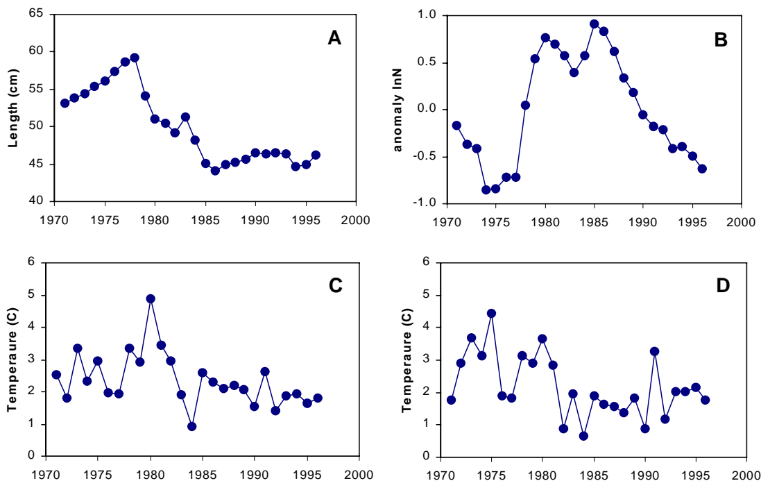
Figure 1. Examples of variation in length-at-age, abundance and temperature conditions for southern Gulf of St. Lawrence cod. A. Length at age 6 yr; B. Abundance index for ages 5-7 yr; C. Environmental temperature index; D. Average ambient temperature of 6-yr-old cod in September.
