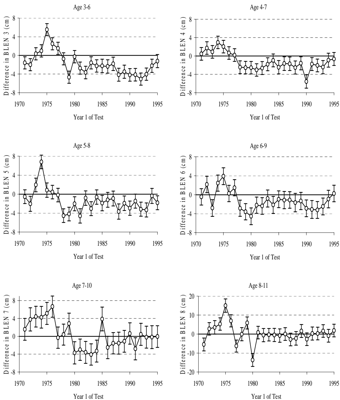
Figure 3: Within year class differences in mean backcalculated lengths at a common age but from fish caught 3 years apart. The label on each panel gives the ages of capture. The differences are calculated as the mean of the older fish less the mean of the younger fish. All panels have a common x-axis which is the year in which the younger age group was caught. Backcalculations assumed a biological intercept of 0.44 mm otolith radius and 2.44 cm fish length.
