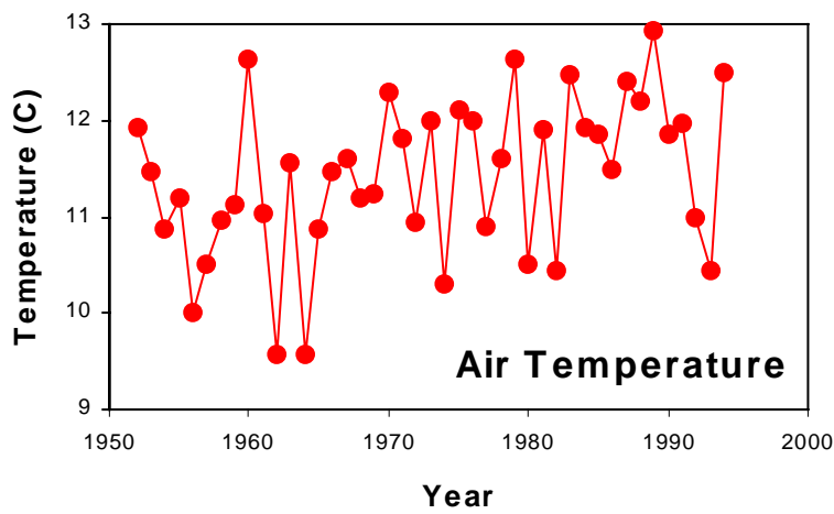
Figure 2. Temperature conditions in the southern Gulf of St. Lawrence. CIL = mean CIL minimum temperatures extrapolated to July 15 (from Gilbert and Pettigrew 1997); Air Temperature = mean monthly air temperatures (May, June, July) at the Magdalen Islands.
