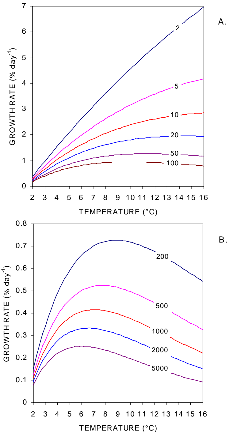
Figure 2 Growth rate of cod as a function of temperature for fish weight from 2-100 g (A) and 200-5000 g (B).
