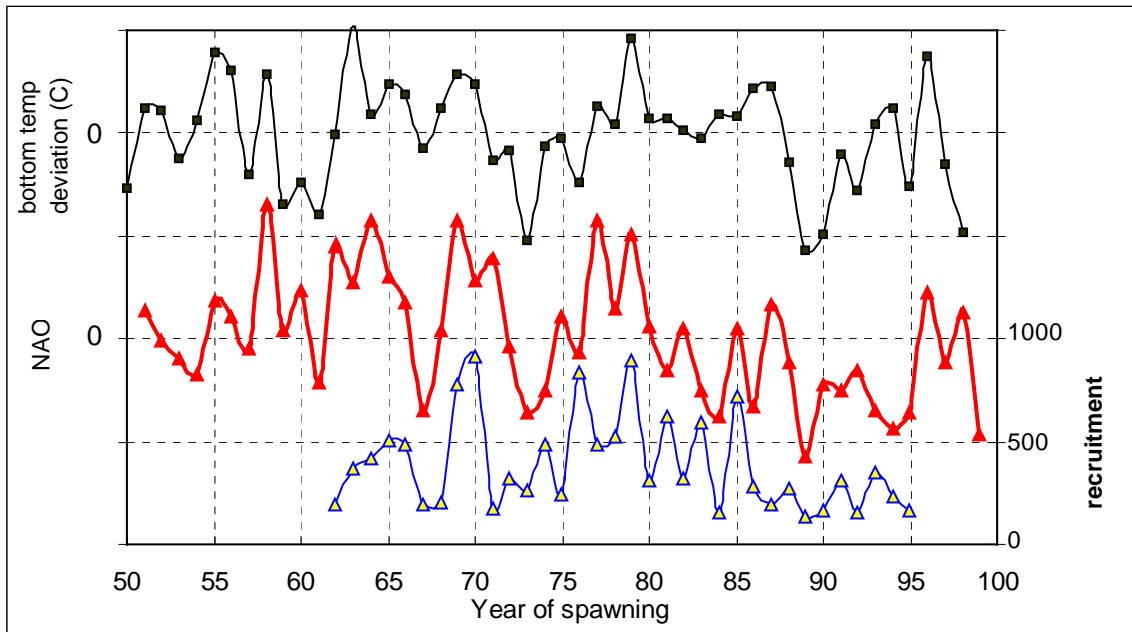
Figure 3. Cod recruitment plotted with deviations in mean bottom temperature and the North Atlantic Oscillation (NAO) index. The dashed lines represent one unit on both the temperature and NAO scales. Both temperature and NAO scales are inverted to facilitate visualisation.
