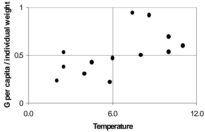
Fig. 4. Size-specific growth production on a per capita basis and cod environment temperature for 3-year-old fish in several stocks
