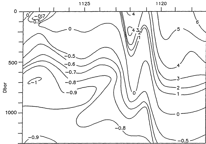
Fig. 3. Potential temperature, salinity and \sigma_\theta in the section across the Arctic Front in November 1993.
