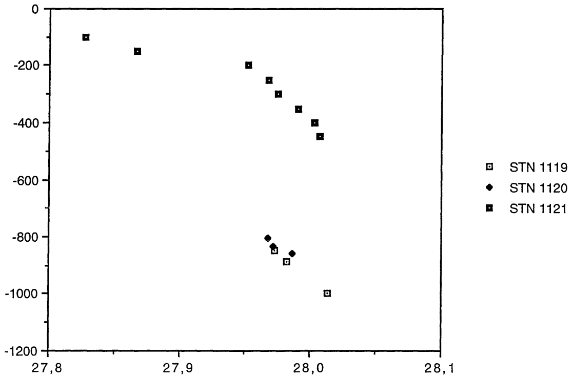
Fig. 4. Potential densities, \sigma_{\theta} , from the frontal tongue with salinities less than 34.88 in Fig. 3, plotted against pressure.
