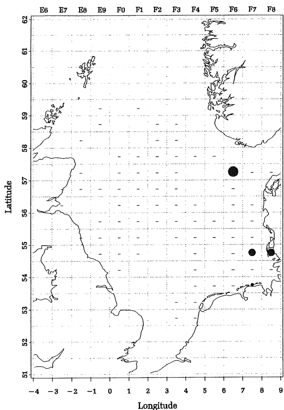
C) PREDATOR=Cod 1981 QUARTER=3
