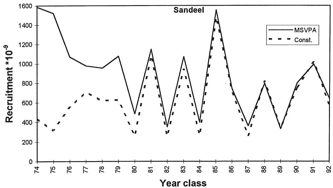
Figure 10.3.2. Recruitment estimates from SXSA using MSVPA or constant natural mortalities.
