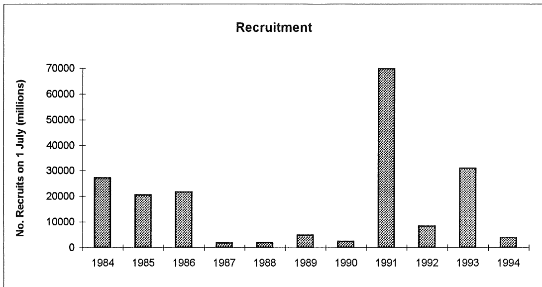
Sandeel at Shetland. Recruitment and Spawning Stock.
