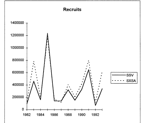
Sandeel, Southern North sea.
