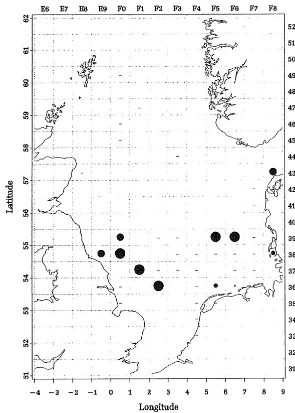
D) PREDATOR=Cod 1981 QUARTER=4
