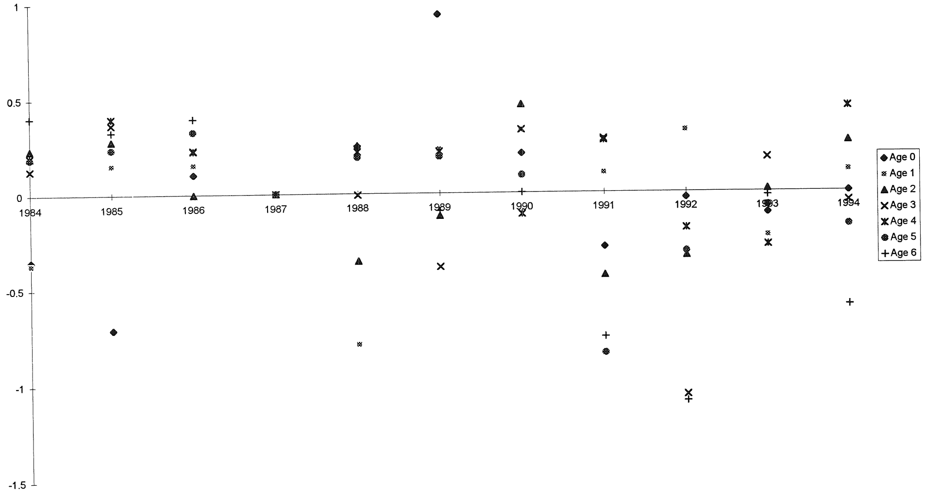
Figure 8.4.1 Sandeels at Shetland, Log RV residuals
