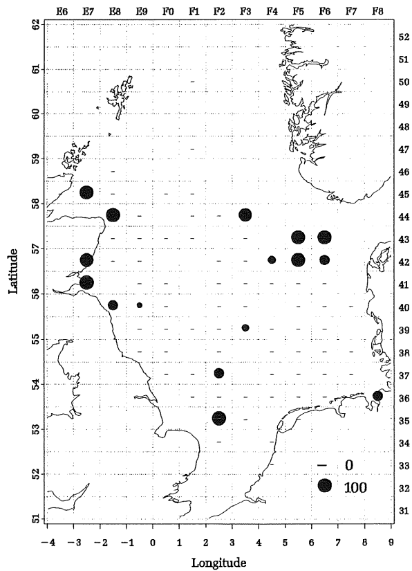
T) PREDATOR=Whiting 1987 QUARTER=3
