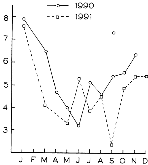
Figure 3. Volume transport through the repeat section. Units in Sverdrup, 10^6 \text{ m}^3/\text{sec} .
