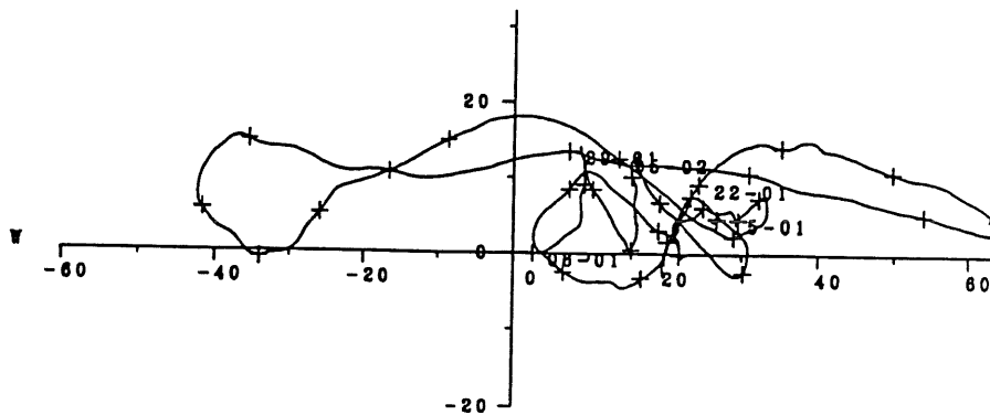
Figure 5. Progressive vector diagram of the current at 186 and 286 m depth at 63^{\circ} 00' N , 03^{\circ} 49' E during the period 8 January - 11 February 1991.
