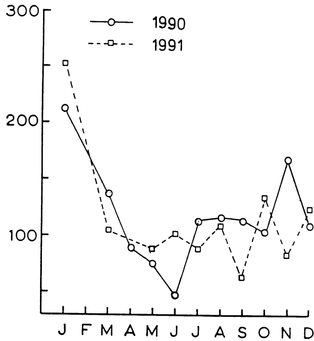
Figure 4. Heat transport through the repeat section. \text{W} \cdot 10^{12} .
