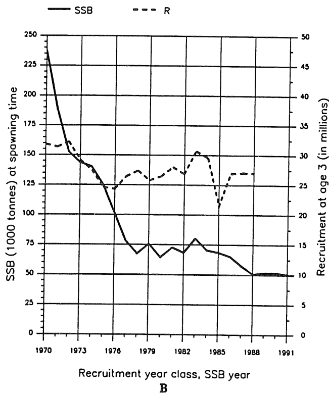
Trends in spawning stock biomass (SSB) and recruitment (R)
