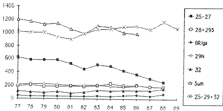
Spawning stock biomass (000) t. Single ass. versus total ass.
