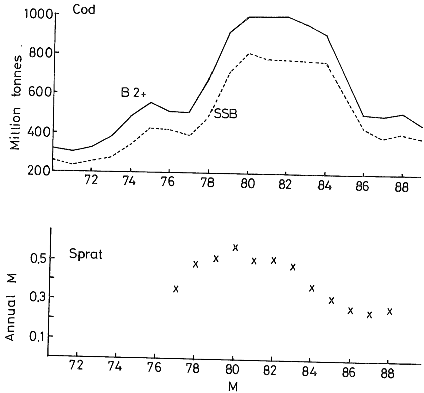
Figure 4.5.1 Natural mortality used for assessment of sprat in Sub-divisions 22-32 (average for ages 1-3) and cod biomass for ages 2+ and spawning stock biomass in Sub-divisions 22-32.
