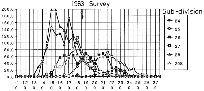
Figure 3.1.3 Herring age group 2. Length frequency distribution by sub-division and from acoustic surveys.
