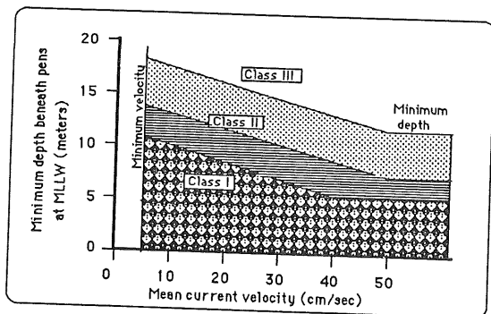
Figure 2 : Minimum depth and current guidelines for salmon net-pen siting in Washington State: Class I = production \leq 9 t/yr; Class II = 9-45 t/yr; Class III = > 45 t/yr.
