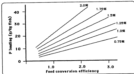
Figure 6 : Estimated phosphorus loading per kg fish produced in relation to phosphorus content of feed and feed conversion efficiency (modified after Mäkinen, 1985).
