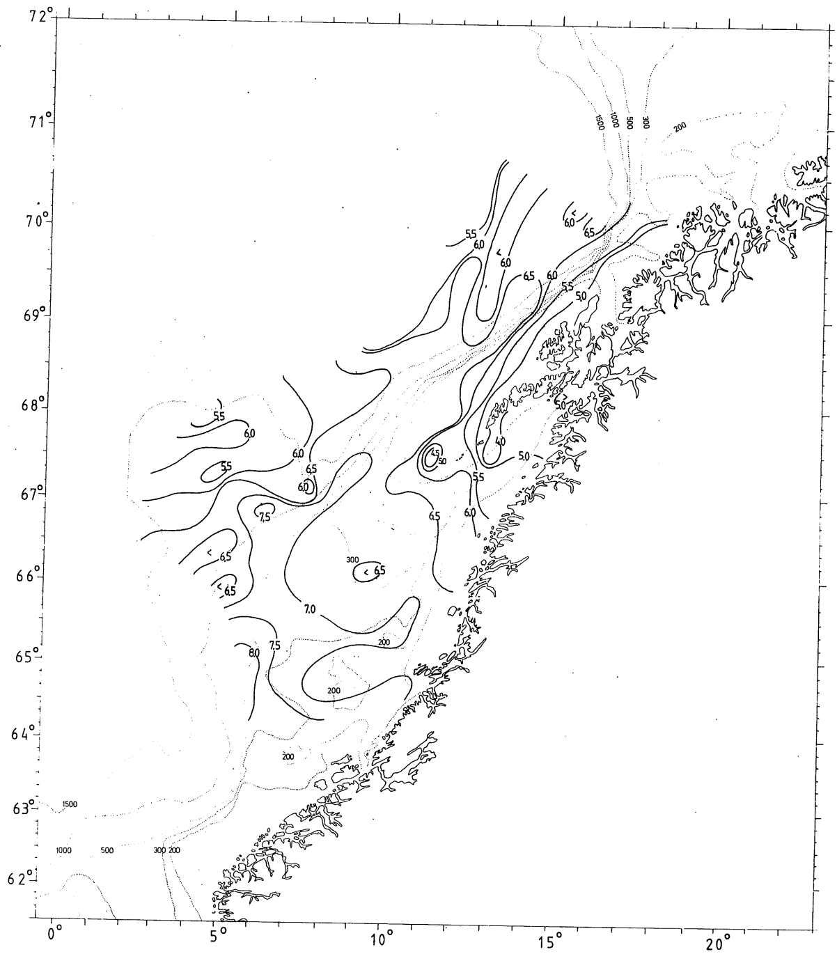
Figure 6. Distribution of temperature ( ^{\circ}\text{C} ) in 100 meter depth or at the bottom where the bottom depth was less than 100 meter.
