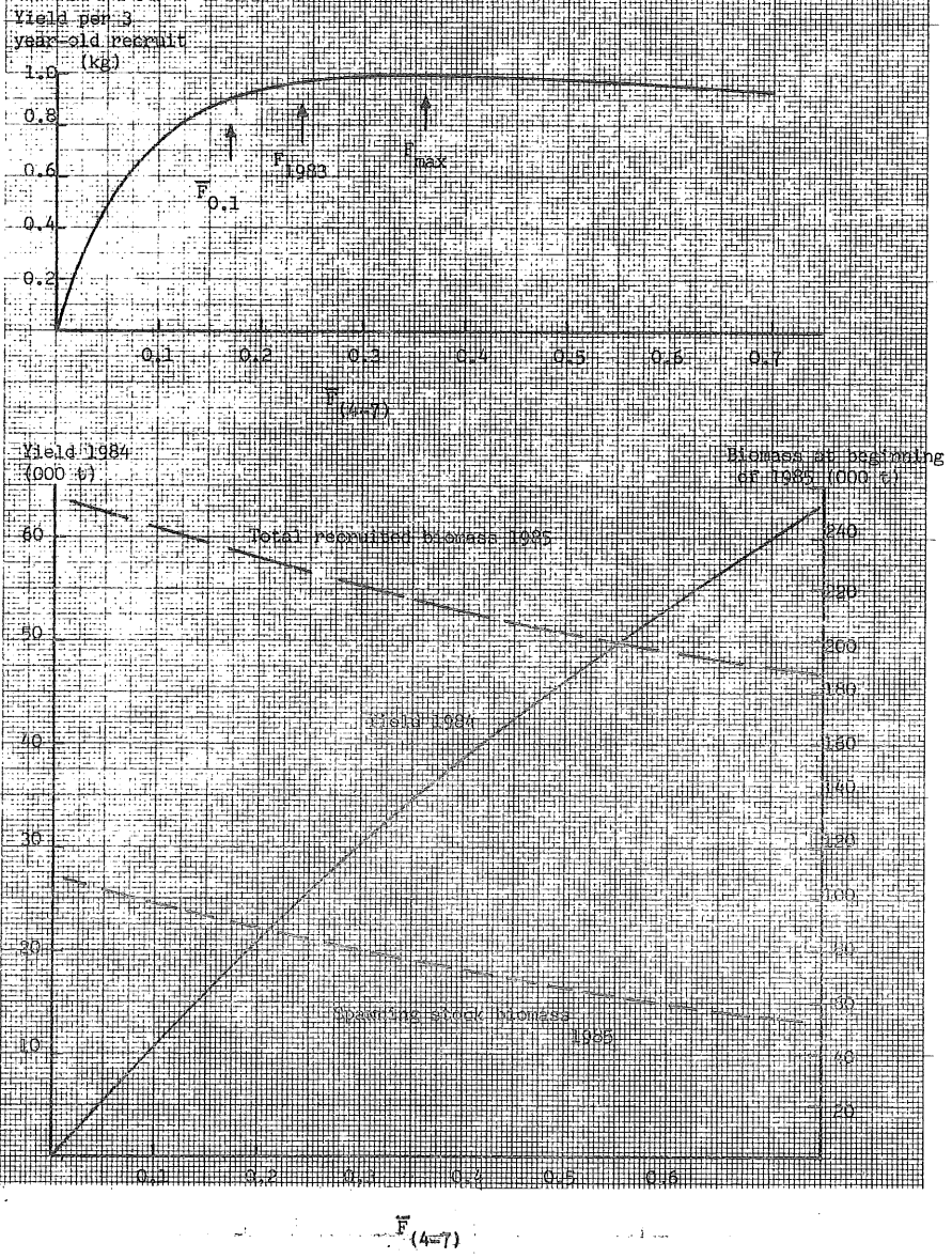
Figure 17. North-east Arctic Haddock, Y/A, yield 1984, total recruited biomass (age 3+) and spawning stock biomass at beginning of 1985 for different levels of fishing mortality in 1984.
