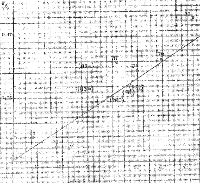
Figure 5 North-East Arctic COD. Fishing mortality generated by Norwegian trawlers in Division IIa on 6 years old versus effort by the same fleet (in Norwegian units) in this area. The upper value for 1983 is the one implied by using the estimate from the acoustic survey in 1983.
