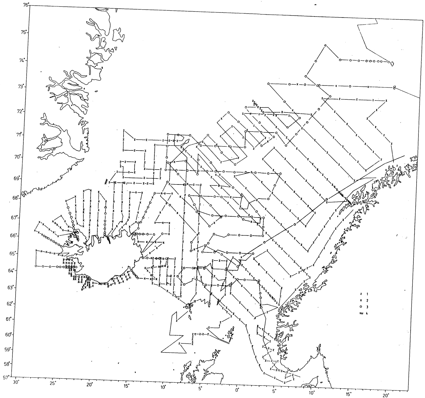
Fig. 2. Cruise tracks and hydrographical stations, August 1983. 1) CTD-sonde, 2) BT and XBT, 3) Water bottles with reversing thermometer, 4) Ice-border.
