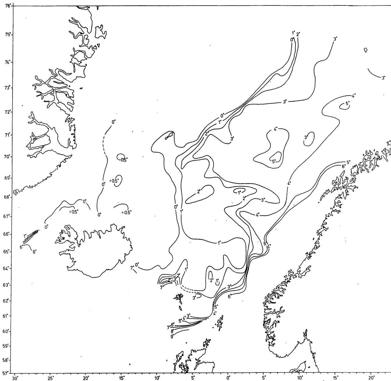
Fig. 5. Temperature ( t^{\circ}\text{C} ) at 400 m depth, August 1983.
