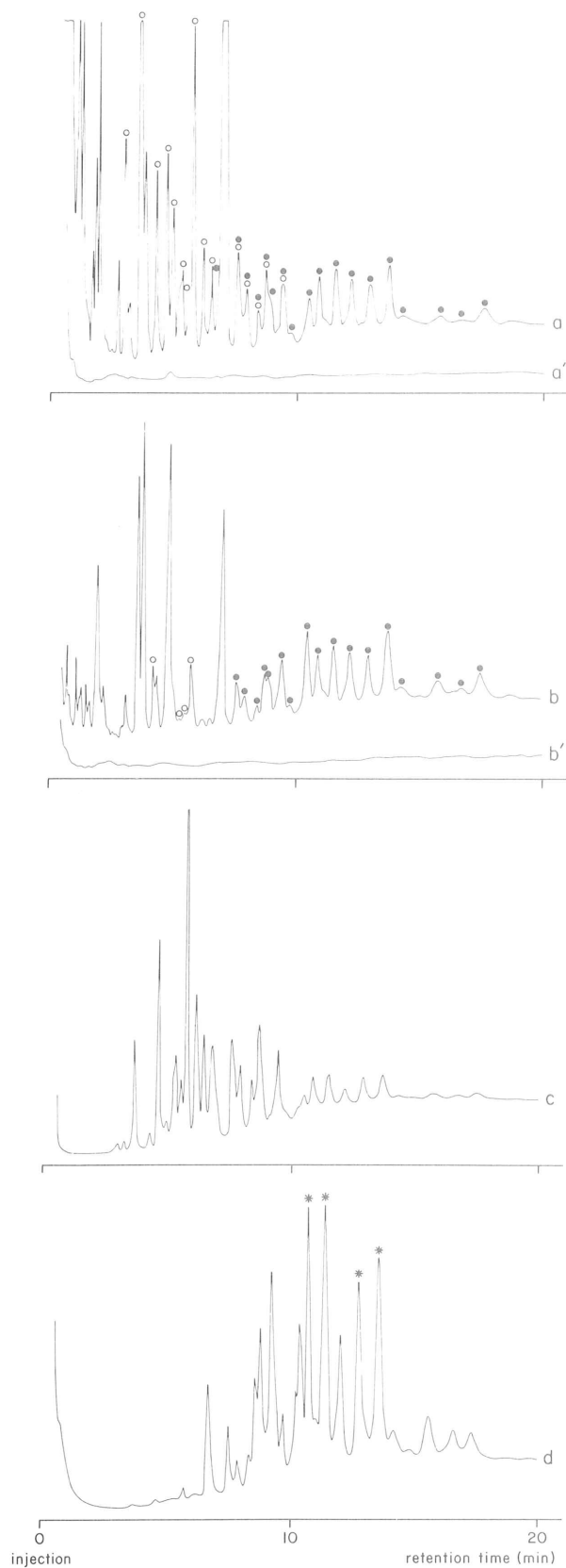
Fig. 1. Chromatograms of the first fractions of extracts of water (a) from the central part of the Southern Bight and (b) from the Danish Wadden Sea. The peaks corresponding to peaks in Clophen A30 (c) are indicated by symbol O and those in Aroclor 1254 (d) by symbol ●. Peaks used for quantitation in terms of Clophen A 50 are indicated by * . Chromatograms of blanks obtained by extracting water that had already been extracted twice are given in a' and b'. Sample volume 120 litres. Temperature programmed conditions 160°C to 215°C, 4°C min. -1 . Column 1.5% SP2250, 1.95% SP2401 on 100-120 mesh Supelcon AWDMCS, 1.8m x 0.64 cm O.D. After Duinker & Hillebrand, 1979b.
