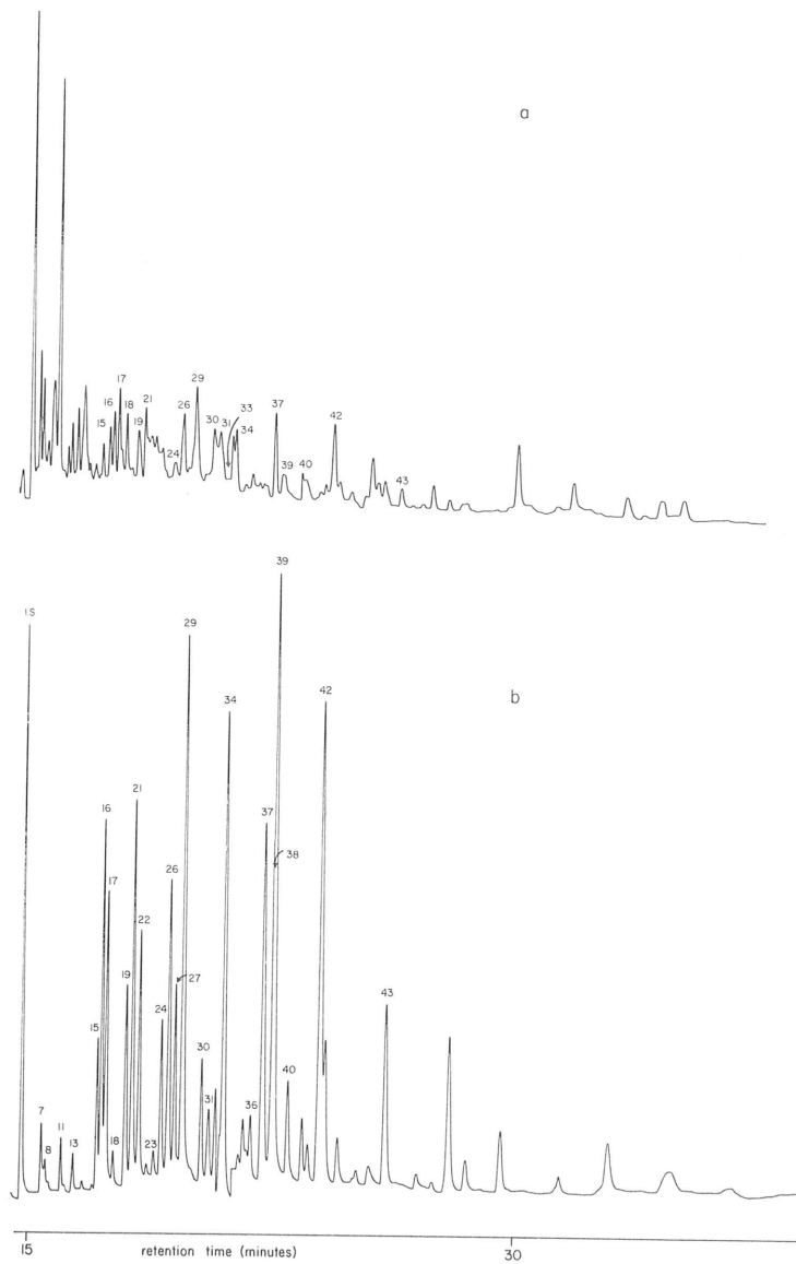
Fig. 2. Temperature programmed capillary column ECD-gaschromatogram of (50 m SE-54) a: seawater extract (see text) and b: Aroclor 1254. I.S. = internal standard. 100-230^{\circ}\text{C} , 8^{\circ}\text{C. min}^{-1} .
