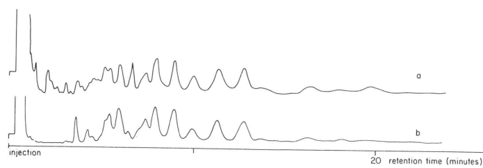
Fig. 3. Isothermal packed column chromatograms of same open ocean sample as in Fig. 2 (a) and Aroclor 1254 (b); column and conditions as in Fig. 1.
