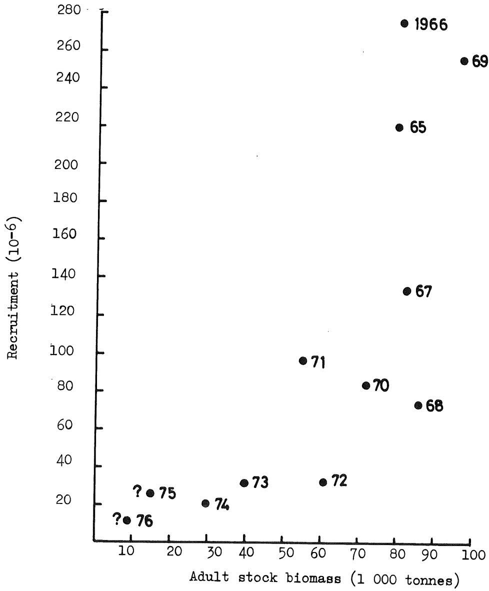
Fig. 3.2 Celtic Sea Herring. Adult Stock biomass (at 1 April) against Recruitment numbers (1 ringers two years later)
