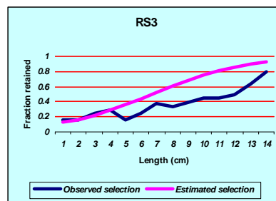
Figure 11. Selection curve by Rigid Sorting.
