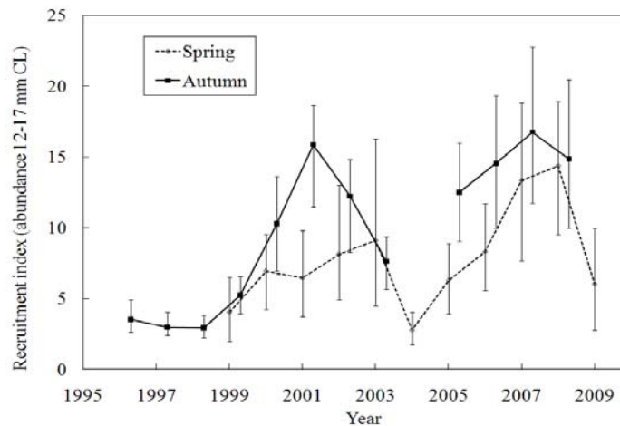
Fig. 2.8. Shrimp in Div. 3LNO: Recruitment indices derived from abundances of male shrimp with 12 – 17 mm carapace lengths from Canadian spring and autumn bottom trawl survey (1996–2009) data.
