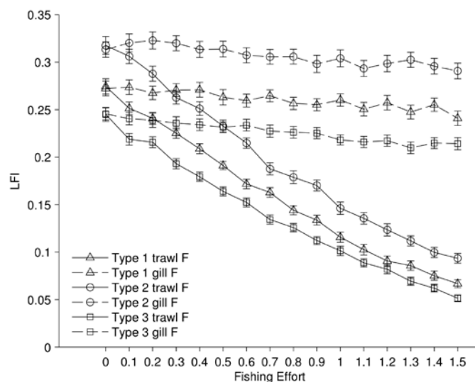
Figure 3.4.2.1. For the FCSR, LFI against fishing effort E for trawl fishing and gillnet fishing, and three fish community types. For each point, the standard deviation over 100 simulations with 100 random parameter sets is shown as a vertical bar. Types 1 to 3 communities differ by the distribution of species over sizes.
