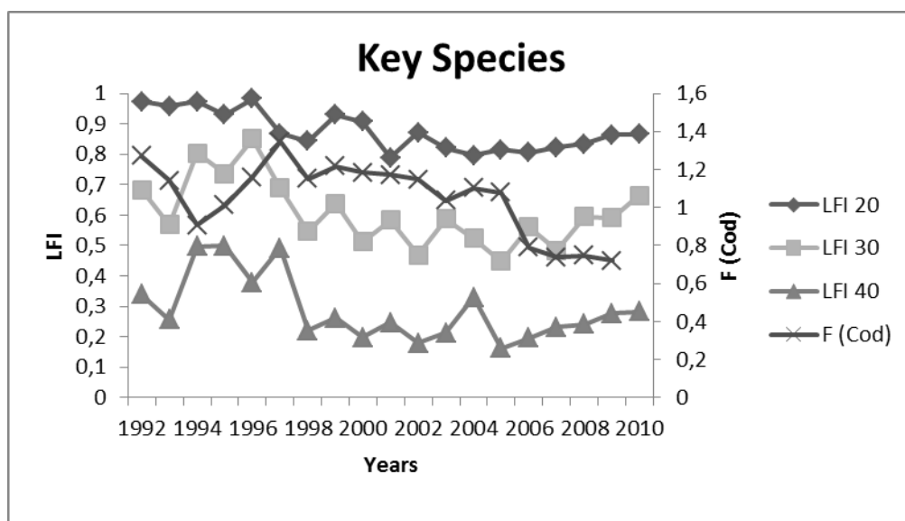
Figure 3.2.1.3. Estimated „Large Fish Indicator“ for P. flesus , L. limanda , G. morhua , M. merlangus , and the four key species together in Subdivision 21, 22, 23, 24 (ICES, Dattras, HLNoATLngt).
