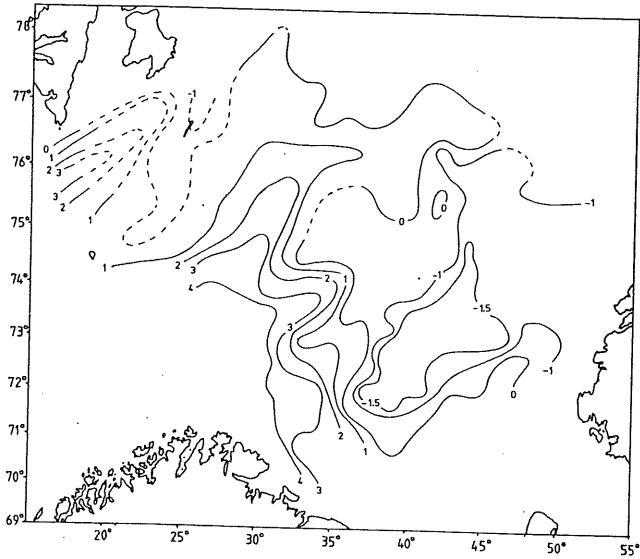
Annex 1, Figure 13. Distribution of temperature ( t^{\circ}\text{C} ) in 200 m depth.
