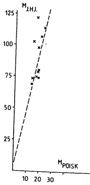
App. 1 to Annex 1, Fig. 1. Intercalibration "Johan Hjort"- "Poisk"
