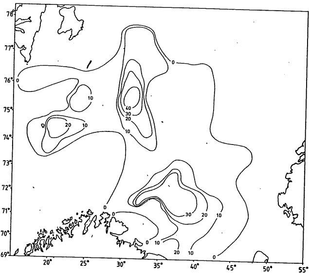
Annex 1, Figure 4. Estimated density distribution of 1-year old capelin (tonnes/(nautical mile) 2 ).
