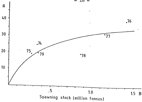
Figure 2.1 Stock-recruitment relation of Barents Sea capelin. The solid line shows the function R = \frac{44,5 \cdot B}{0,43 + B} where R = recruited individuals \times 10^{10} and B = spawning stock biomass in mill. tonnes.
