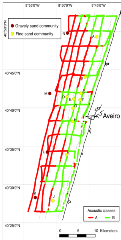
Figure b10. GIS representation of the acoustic classes and the biological affinity groups in the near shore shelf off Aveiro (area C (Freitas, 2003b)).
