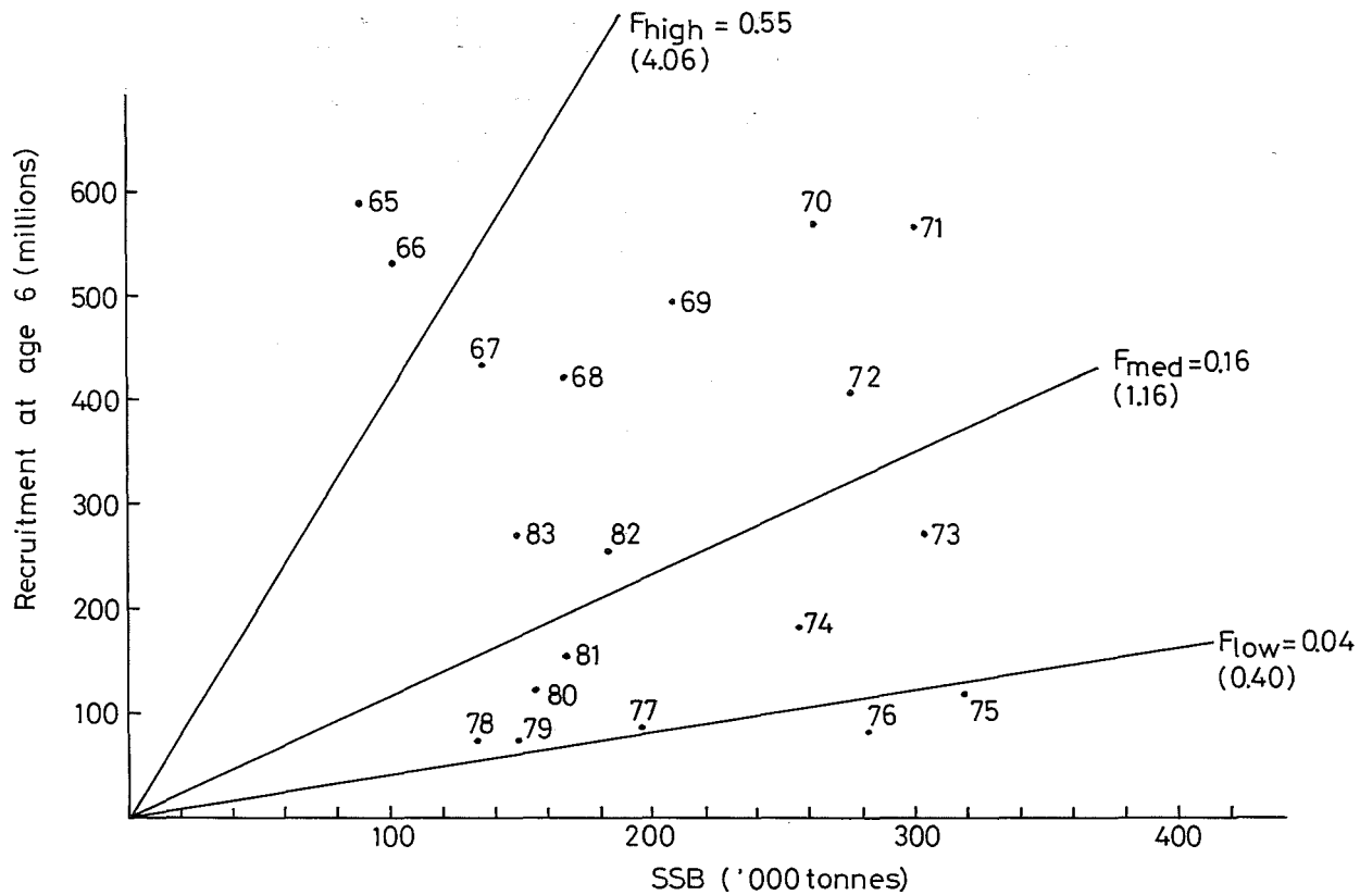
Figure 6.4 Stock-recruitment plot for Sebastes mentella .
