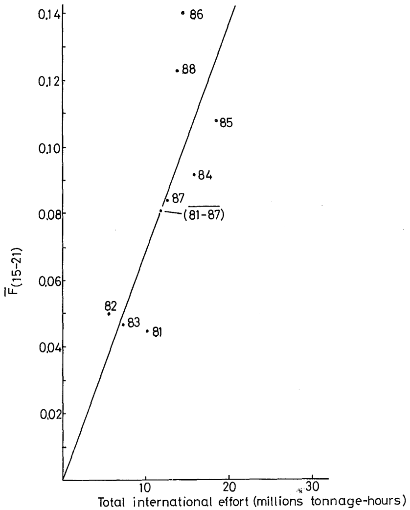
Figure 6.6 Sebastes marinus in Sub-areas I and II. Fishing mortality vs. total effort.
