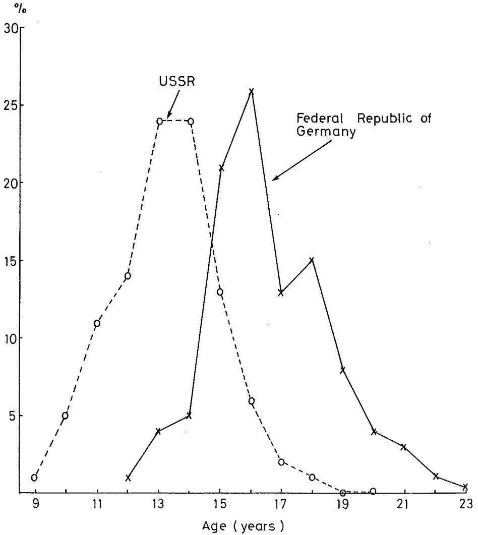
Figure 6.1B Sebastes mentella . Corresponding age distributions (%) of the landings in 1988 from the USSR and the Federal Republic of Germany.
