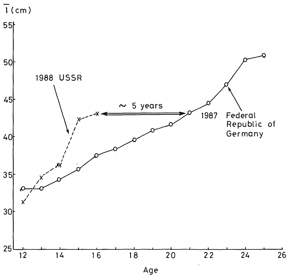
Figure 6.2 Sebastes mentella . Age-length relationship for the USSR and the Federal Republic of Germany landings presented to the Arctic Fisheries Working Group in 1988.
