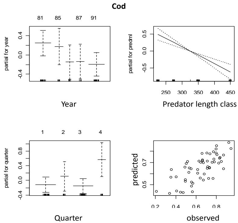
Figure 9.2.2. Fitted relative stomach contents for Other Food as a function of year, quarter and predator length class. In addition, the relationship between observed and predicted relative stomach contents for cod is shown.
