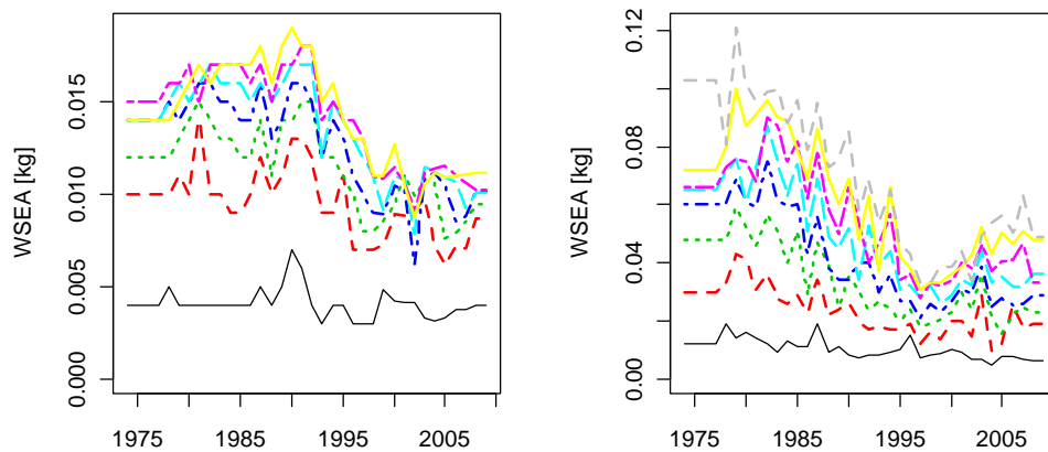
Figure 10.3.1. Weight in the sea by age group for Eastern Baltic sprat (left panel) and Eastern Baltic herring (excl. Gulf of Riga, right panel).
