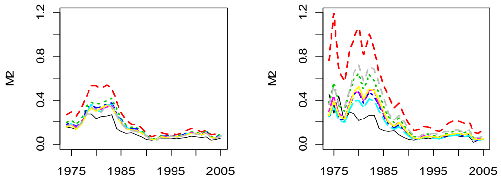
Figure 10.3.4. Predation mortality (M2) of sprat, left SMS, right 4M, increasing age from top to bottom.
