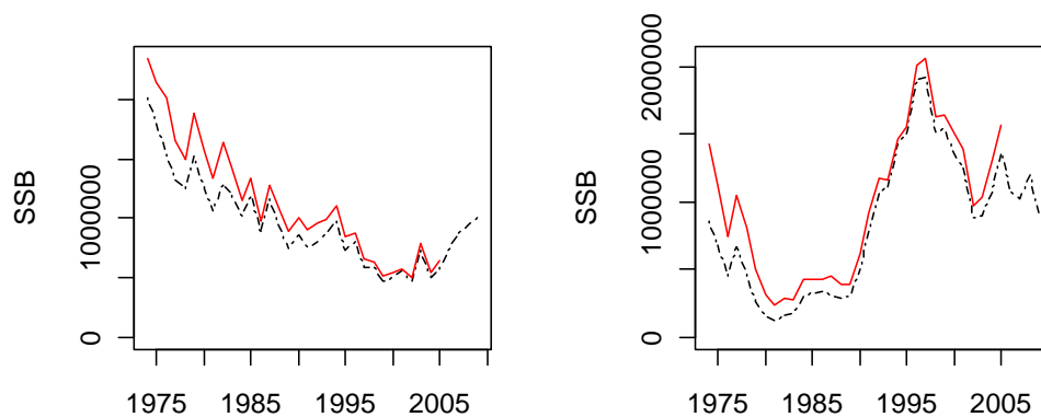
Figure 10.3.3. Time series of Eastern Baltic herring (left) and sprat (right) SSB, based on 4M (red solid), and SMS (black dot-dashed).
