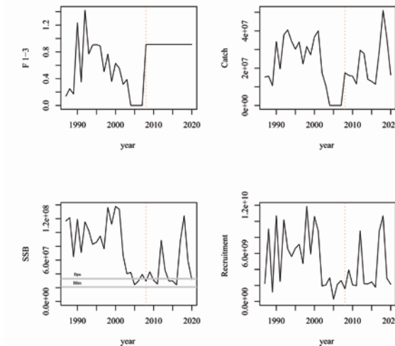
Figure 3.7.1. Summary of the evolution of the anchovy population dynamics in the Bay of Biscay.
