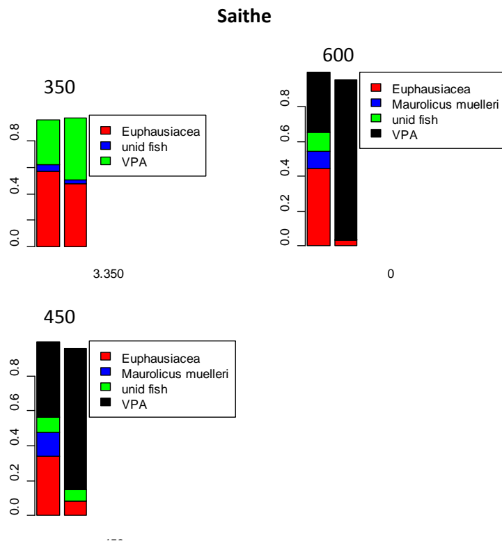
Figure. 9.2.7. Diet composition of different predator length classes of saithe in the third quarter. Only prey types with more than 3% relative stomach content are taken into account.
