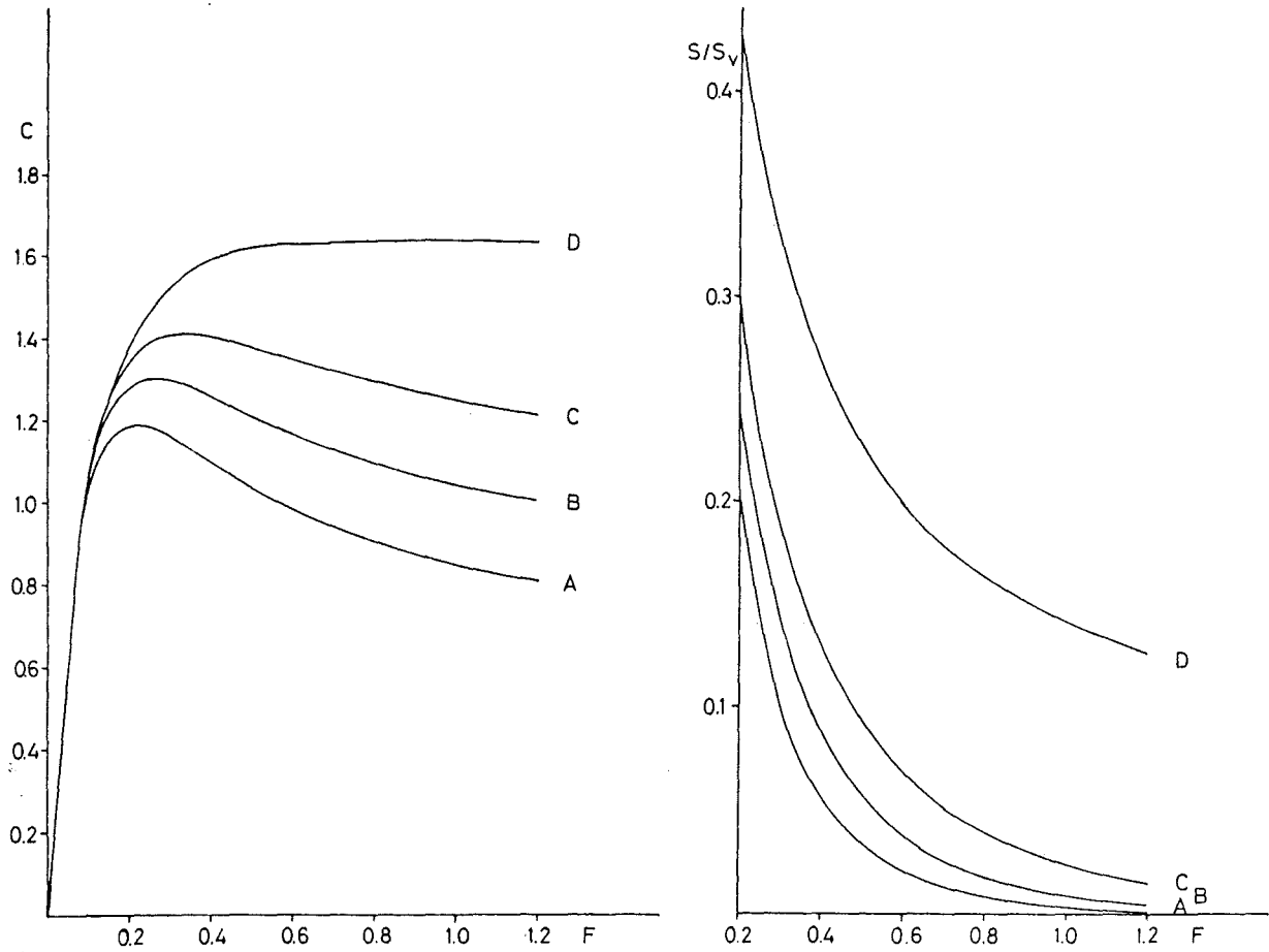
Fig. 1. Yield per recruit (C) and spawning stock per recruit ( S/S_v where S_v = spawning stock per recruit in unexploited stock) against fishing mortality (F).
