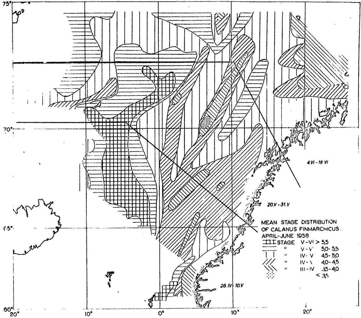
Fig. 8. The mean stage distribution of Calanus finmarchicus April-June 1958.
