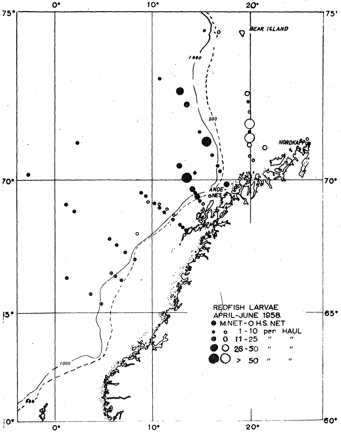
Fig. 17. The quantitative distribution of redfish larvae April-June 1958.
