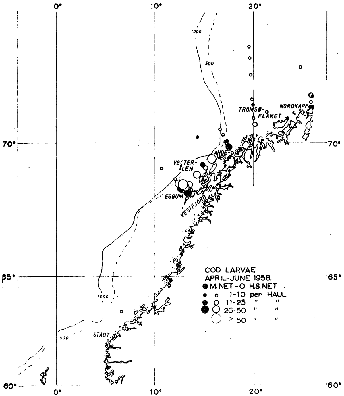
Fig. 12. The quantitative distribution of cod larvae April-June 1958.
