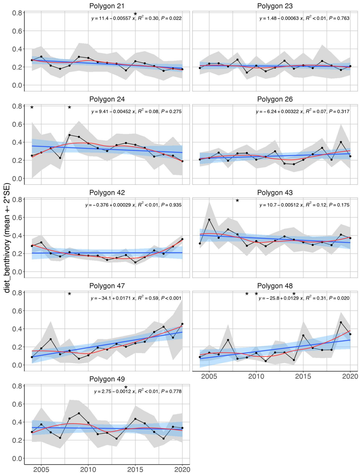
Figure A.3.6. Mean ( \pm 2 *SE) biomass proportion of the benthivorous feeding guilds in the Arctic Barents Sea (Black dots and grey shading). Linear regression fit with 95% CI is shown in blue, and the statistical results are given in the top of each plot. A local smoother is added in red to assist visual interpretation of non-linear changes during the period. Stars indicate years with low sample size (< 5 trawls).
