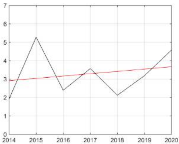
Figure A.29.2 Themisto libellula time series and fitted trend represented by the red line. The fitted trend is of degree 1 (linear) with R^2=0.05 . Residual variance after fitting was 1.55.
