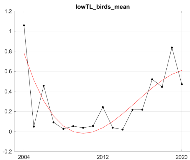
Figure A.8.2 The red line represents fitted trend of degree 3 (cubic). After fitting, residuals variance was 0.03, R^2=0.66 .
