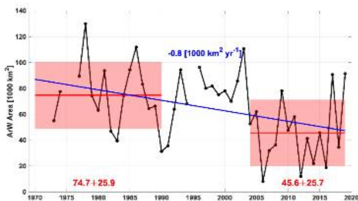
Figure A.38.1 Estimated area covered by Arctic Water in the water column. Means and standard deviations for 1970-1990 and 2004-2019 are shown by red lines and pale red boxes with actual shown in red. Linear trends 1970-2019 and 2004-2019 are shown in blue when statistically significant at the 95% level (with actual values also in blue).
