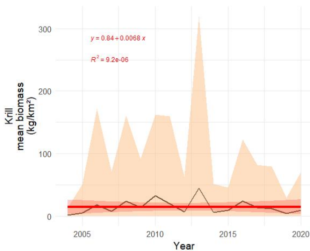
Figure S. 21.1. The time series of estimated biomass of krill (kg wet wt. km 2 ) shown with light shaded areas indicating \pm 1 SD. Red line and red shaded areas indicate fitted linear trend and 95% confidence band, with equation and R^2 indicated in red.
