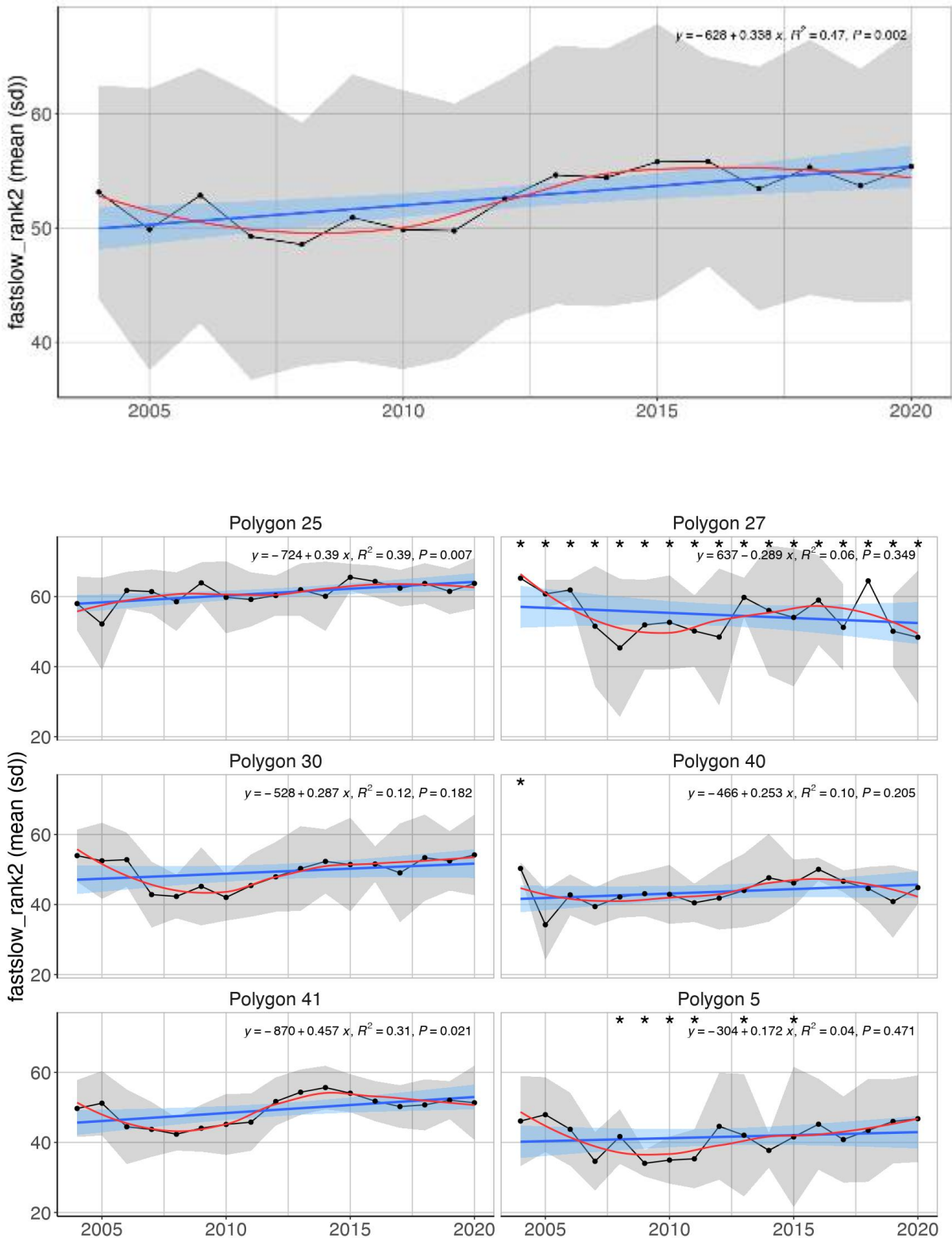
Figure S.15.2 Mean ( \pm sd) biomass weighted fast-slow life history rank value in the Sub-Arctic part of the Barents Sea (Black dots and grey shading). High values translate to slow life history strategy. Linear regression fit with 95% CI is shown in blue, and the statistical results are given in the top of each plot. A local smoother is added in red to assist visual interpretation of non-linear changes during the period. Stars denote years with low sample size (< 5 trawls).
