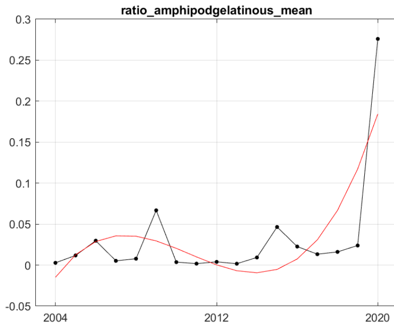
Figure A.13.2 Estimated ratio of biomass of pelagic amphipods ( \text{kg}/\text{km}^2 wet wt.) to biomass of gelatinous zooplankton ( \text{kg}/\text{km}^2 wet wt.) and fitted trend represented estimated by the best fitted trend approach by the red line. The fitted trend is of degree 3 (cubic) with R^2=0.60 . Residual variance after fitting was 0.001.
