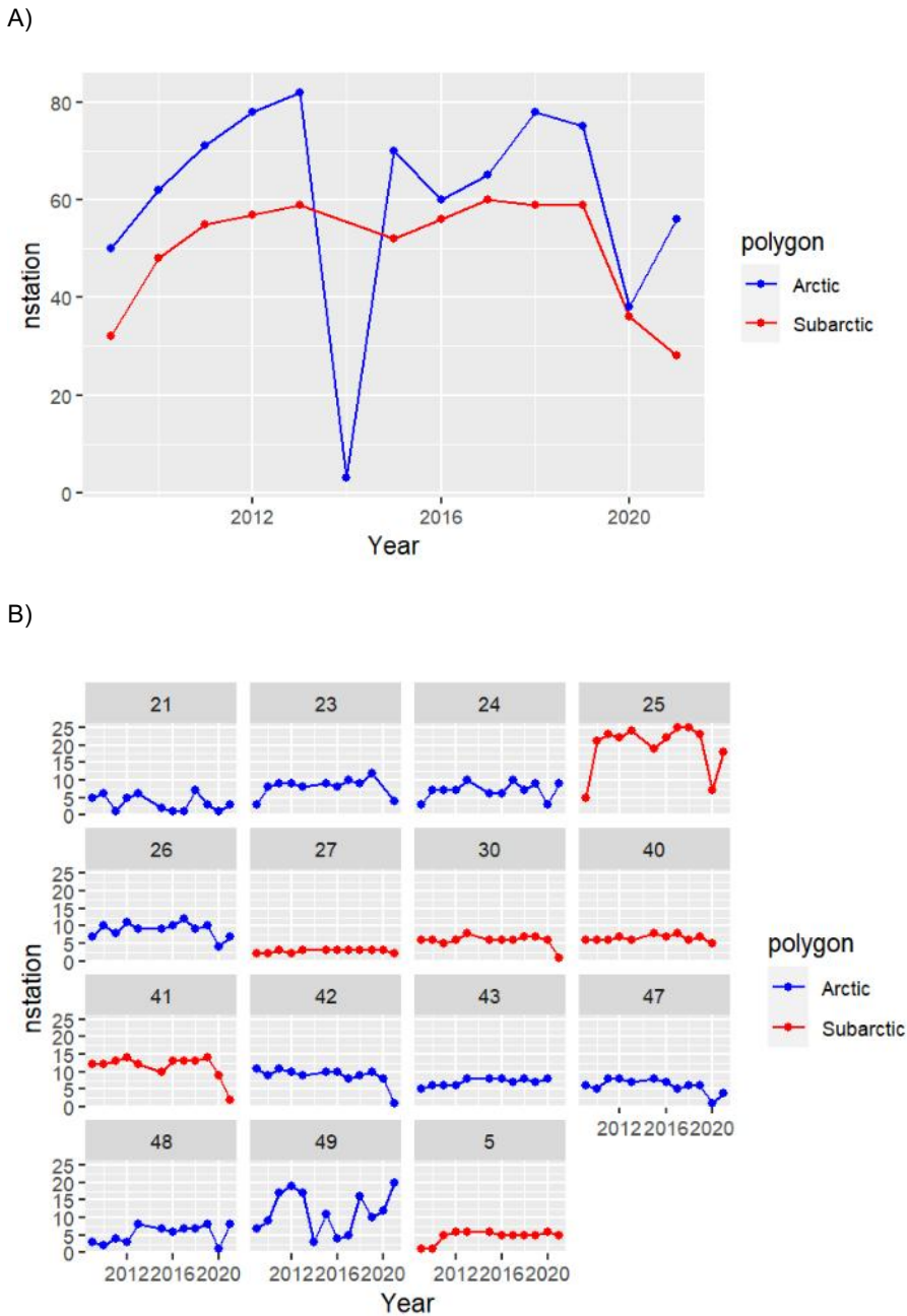
Figure A.30.4 Number of stations used in the data. Top: in the whole area. Bottom: per polygon.
