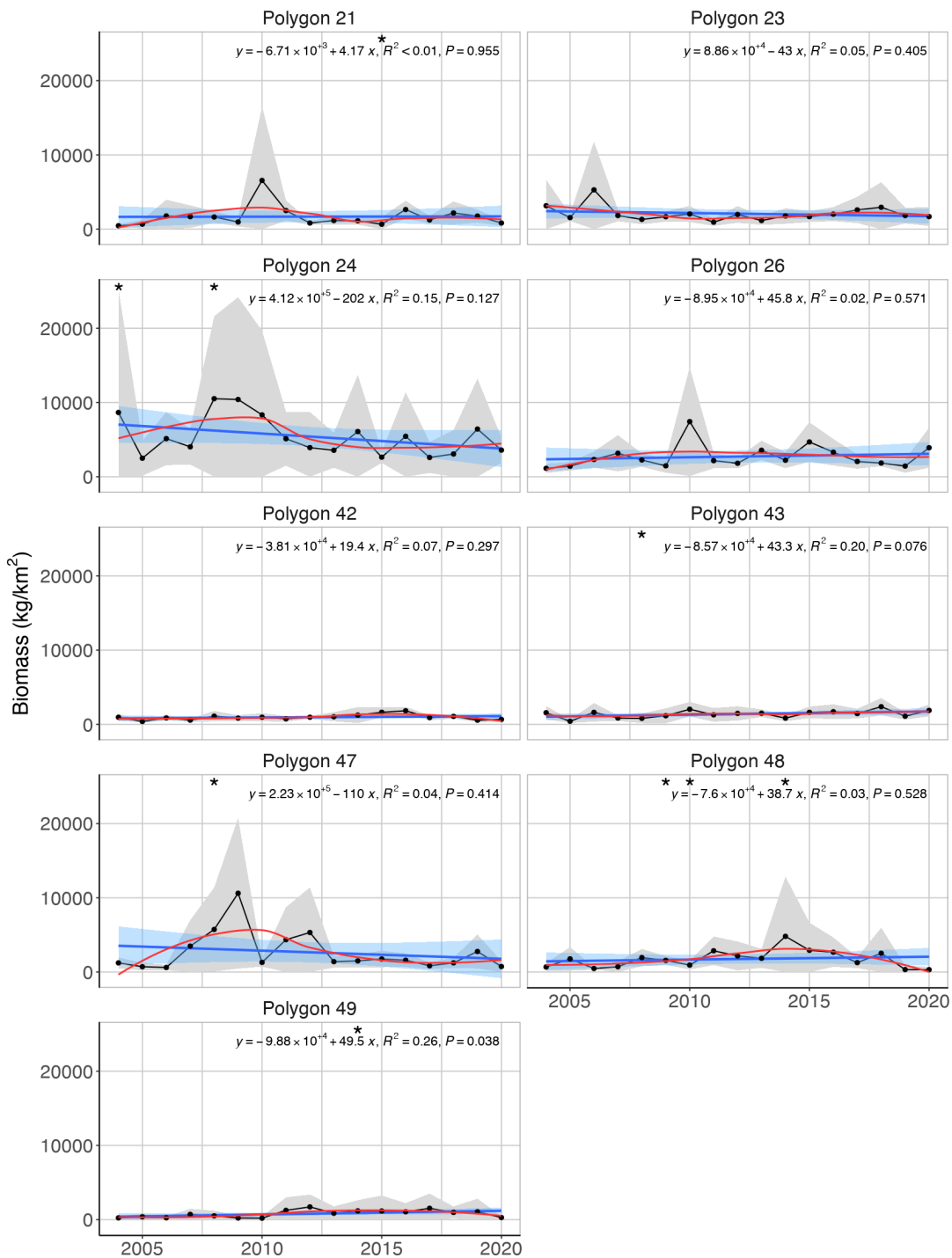
Figure A.2.3. Mean ( \pm 2 SE) biomass of high trophic level demersal fish, for polygons in the Arctic Barents Sea (Black dots and grey shading). Linear regression fit with 95% CI is shown in blue, and the statistical results are given in the top of each plot. A local smoother is added in red to assist visual interpretation of non-linear changes during the period. Stars indicate years with low sample size (< 5 trawls).
