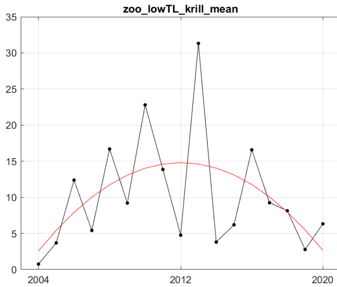
Figure S.3.2 Estimated krill biomass (kg wet wt. km 2 ) and fitted trend using best fitted trend approach represented by the red line. The fitted trend is of degree 2 (quadratic) with R^2=0.27 . Residual variance after fitting was 46.38.
