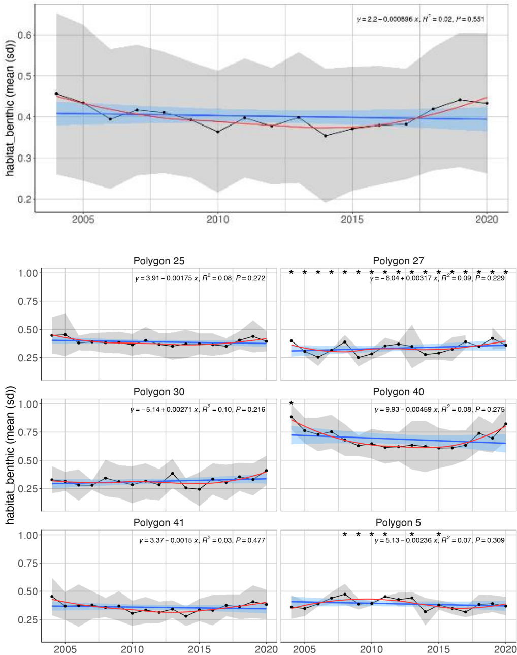
Figure S.16.3 Mean (± sd) log biomass proportion of benthic fish species excluding cod in the Sub-Arctic part of the Barents Sea (Black dots and grey shading). Linear regression fit with 95% CI is shown in blue, and the statistical results are given in the top of each plot. A local smoother is added in red to assist visual interpretation of non-linear changes during the period. Stars denote years with low sample size (< 5 trawls).
