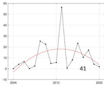
Figure S.3.4 Mean biomass of low trophic level krill ( \text{kg wet wt. km}^{-2} ) in each polygon in the Subarctic part of the Barents Sea (number on top of each panel) shown with fitted trends estimated using the best fitted trend approach represented by the red line.
