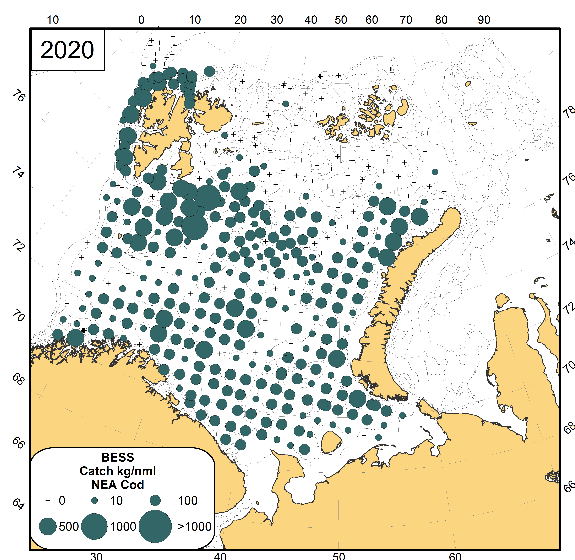
Figure A.26.4. Geographical distribution of cod from the Barents Sea Ecosystem Survey in 2004, 2013 and 2020 (WGIBAR report 2021).
