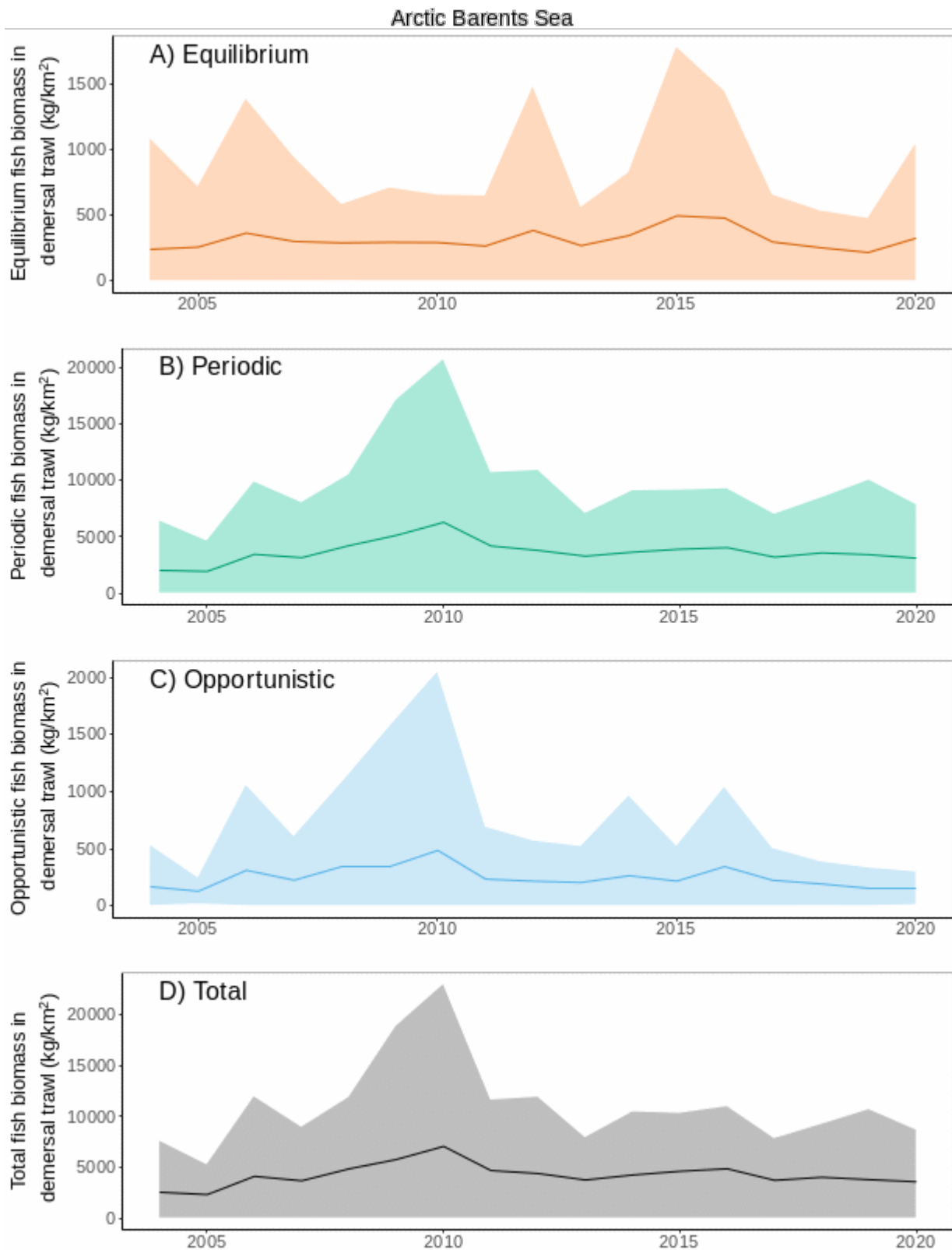
Figure A.16.8 Mean ( \pm sd) biomass of three different life history strategies the Arctic part of the Barents Sea
