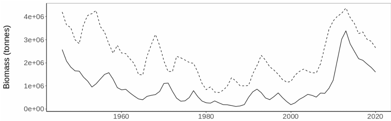
Figure S.24.2 Biomass of large cod (> 6 years; solid line) compared to total stock biomass (stippled line).
