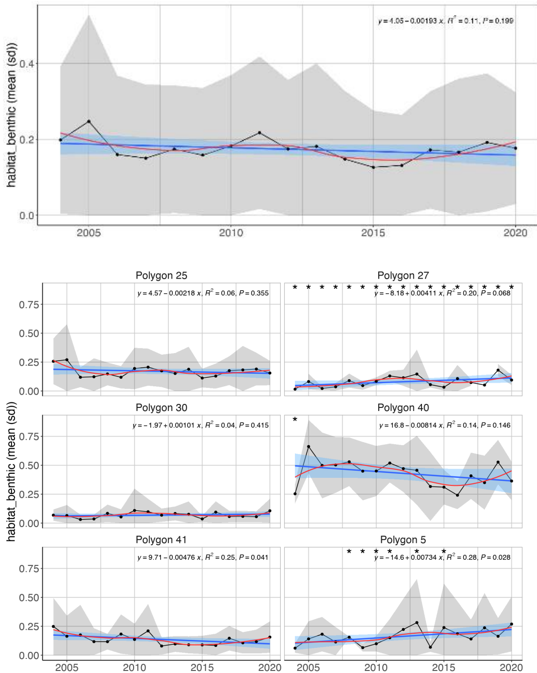
Figure S.16. 1 Mean ( \pm sd) biomass proportion of benthic fish species in the Sub-Arctic part of the Barents Sea (Black dots and grey shading). Linear regression fit with 95% CI is shown in blue, and the statistical results are given in the top of each plot. A local smoother is added in red to assist visual interpretation of non-linear changes during the period. Stars denote years with low sample size (< 5 trawls).
