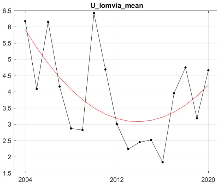
Figure A.9.2 A) Mean ( \pm sd) biomass (kg / km 2 ) of thick-billed murre ( U. lomvia ) in the Arctic Barents Sea from BESS. B) The red line represents fitted trend of degree 2 (quadratic). After fitting, residuals variance was 1.37, R^2=0.34 .
