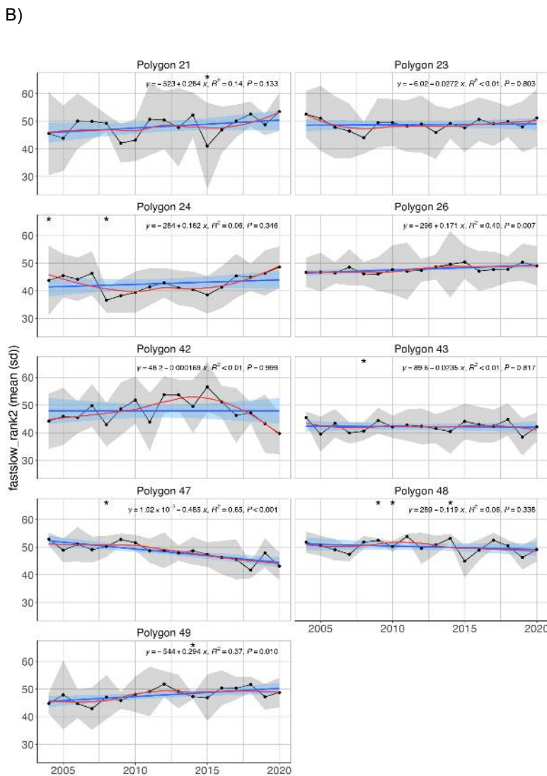
Figure A.16.2 Mean ( \pm sd) biomass weighted fast-slow life history rank value in the Arctic part of the Barents Sea (Black dots and grey shading). High values translate to slow life history strategy. Linear regression fit with 95% CI is shown in blue, and the statistical results are given in the top of each plot. A local smoother is added in red to assist visual interpretation of non-linear changes during the period. Stars denote years with low sample size (< 5 trawls). A) in the whole area. B) per polygons.
