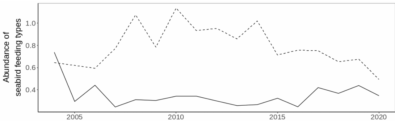
Figure A.18. 5 Mean sum of normalized logged counts of diving (solid line) and surface feeding (stippled line) seabird species in the Arctic Barents Sea.
