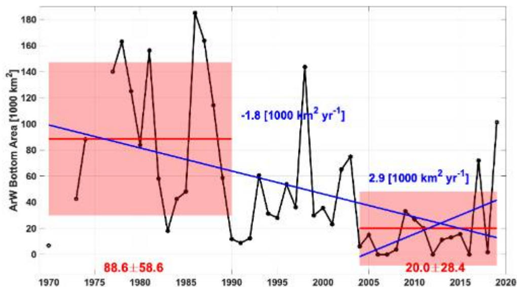
Figure A.27.1 Estimated area covered with cold-water ( T < 0^\circ\text{C} ) temperature niches at bottom. Means and standard deviations for 1970-1990 and 2004-2019 are shown by red lines and pale red boxes with actual values shown in red. Linear trends 1970-2019 and 2004-2019 are shown in blue when statistically significant at the 95% level (with actual values also in blue).
