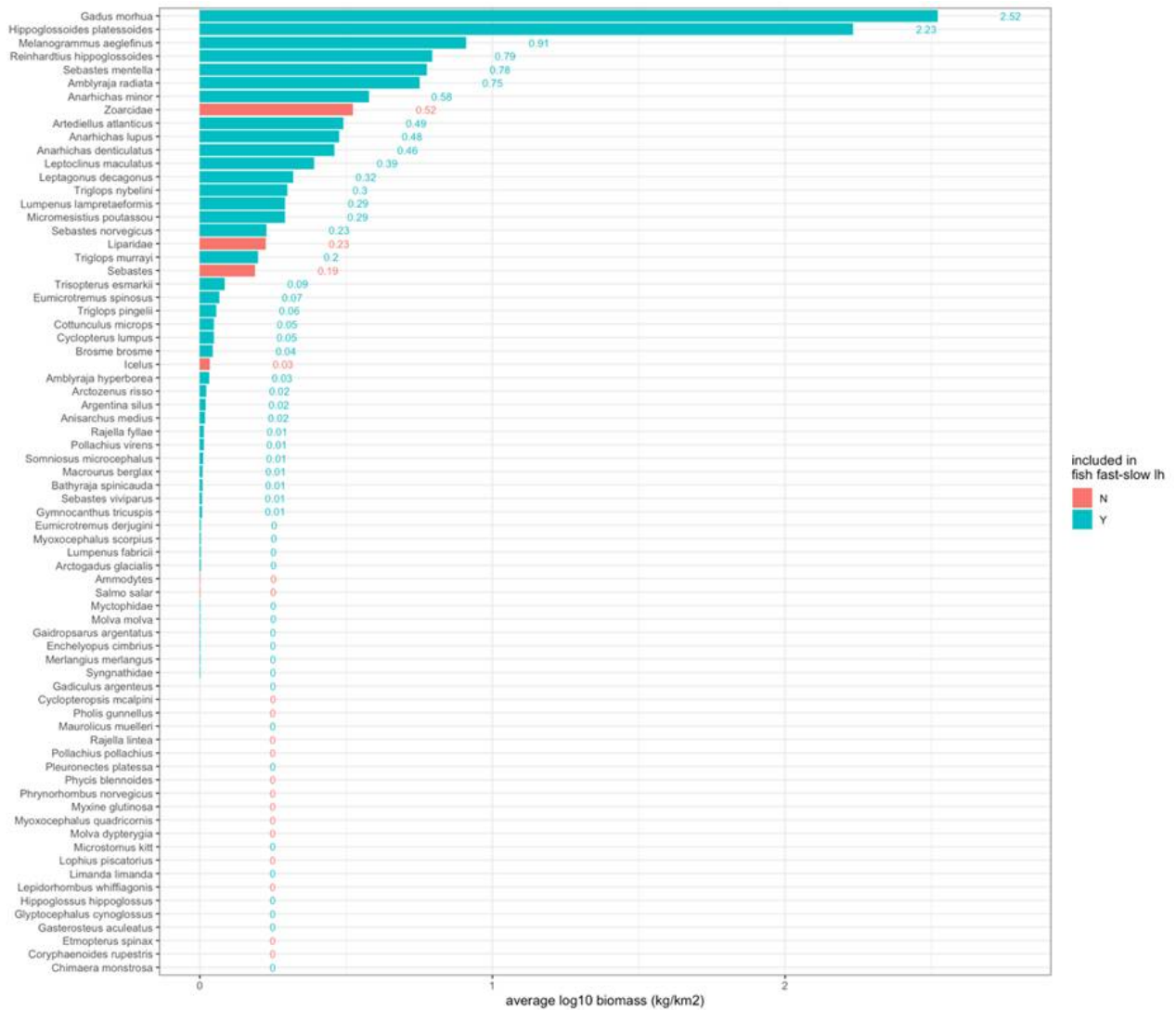
Figure A. 16.9 Mean biomass of demersal fish species in the Arctic part of the Barents Sea. Blue bars denote species included in A) the three life history strategies, B) the fast-slow life history continuum.
