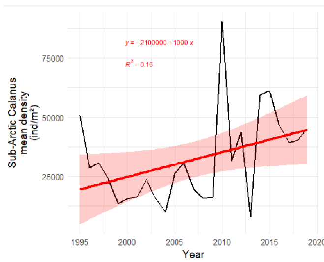
Figure S.20.1. The time series of estimated abundance of sub-Arctic Calanus (ind. m^{-2} ). Red line and shaded areas indicate fitted linear trend and 95% confidence band, with equation and R^2 indicated in red.
