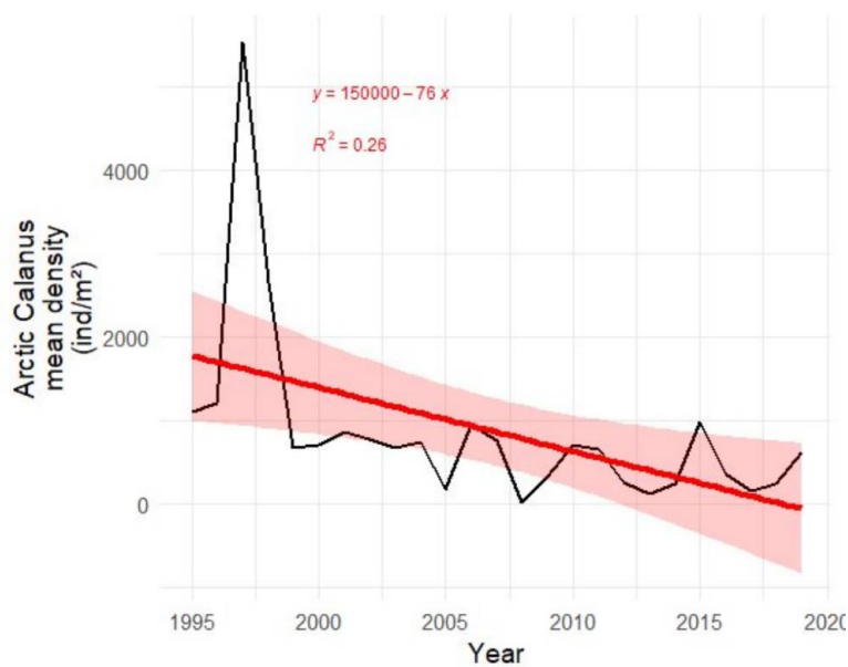
Figure S. 19.1. The time series of estimated abundance of Arctic Calanus species (ind. m 2 ). Red line and shaded areas indicate fitted linear trend and 95% confidence band, with equation and R^2 indicated in red.
