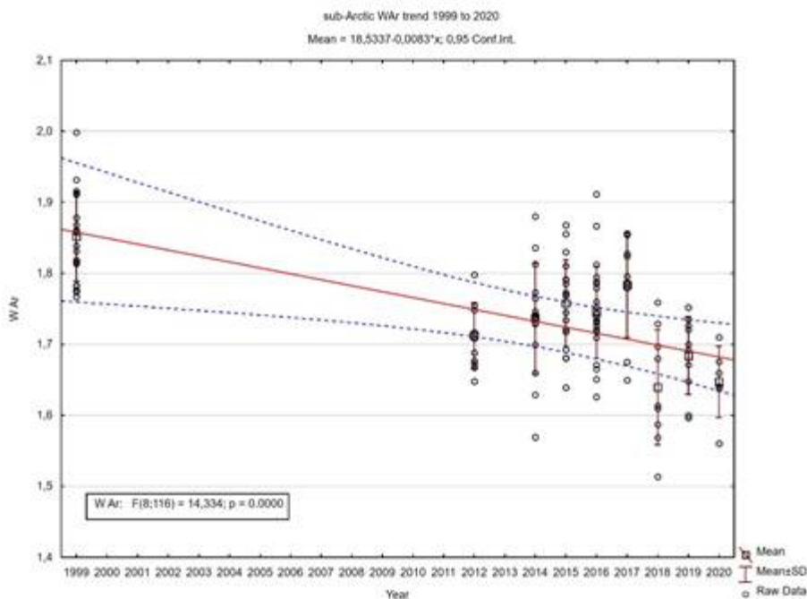
Figure S.36.1 The time series of aragonite saturation ( \Omega_{\text{Ar}} = \text{WAr} ) in the period 1999 to 2020 in the sub-Arctic ( T > 3^\circ\text{C} ) waters. The linear fit (red line) is based on annual mean values (black squares) from observational data (circles). The blue hashed lines denote the area of 95% confidence.
