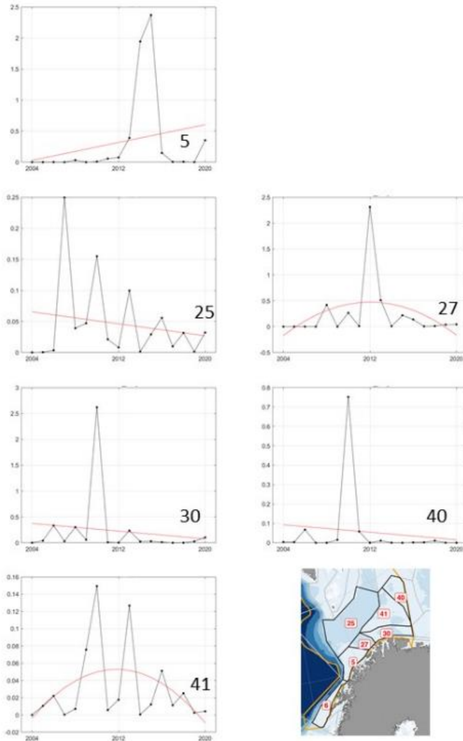
Figure S.12.5. Estimated ratio of the biomass ( \text{kg wet wt. km}^{-2} ) of krill to the biomass gelatinous plankton and fitted trend using the best fitted trend approach represented by the red line in each polygon in the sub-Arctic part of the Barents Sea (number on top of each panel).
