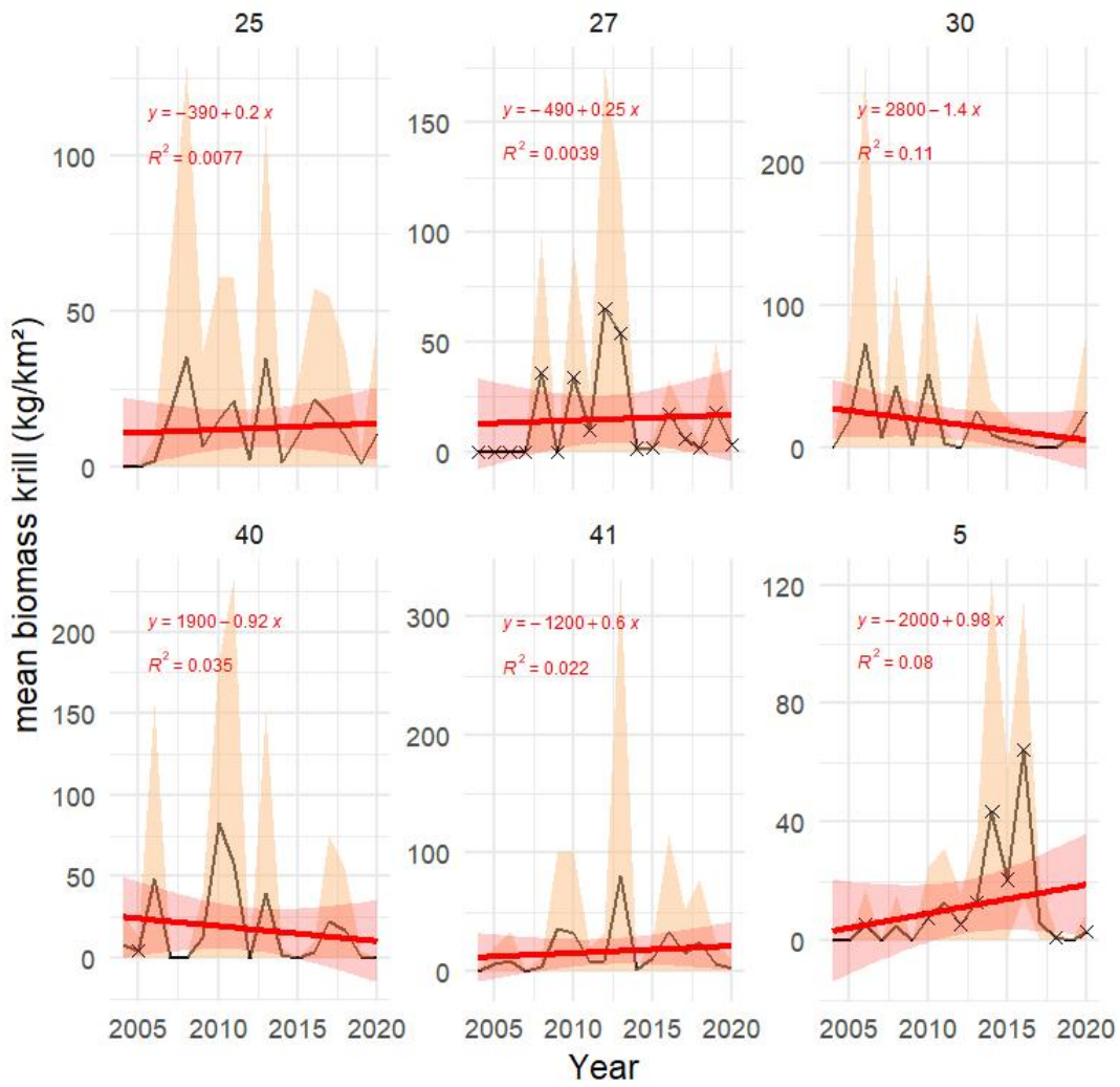
Figure S.21.3 Mean biomass of krill (kg wet wt. km -2 ) in each polygon in the subarctic part of the Barents Sea (number on top of each panel) with light shaded area indicating ± 1 SD. Red line and red shaded areas indicate fitted linear trend and 95% confidence band, with equation and R 2 indicated in red. Stars denote years with low sample size (< 5 trawls).
