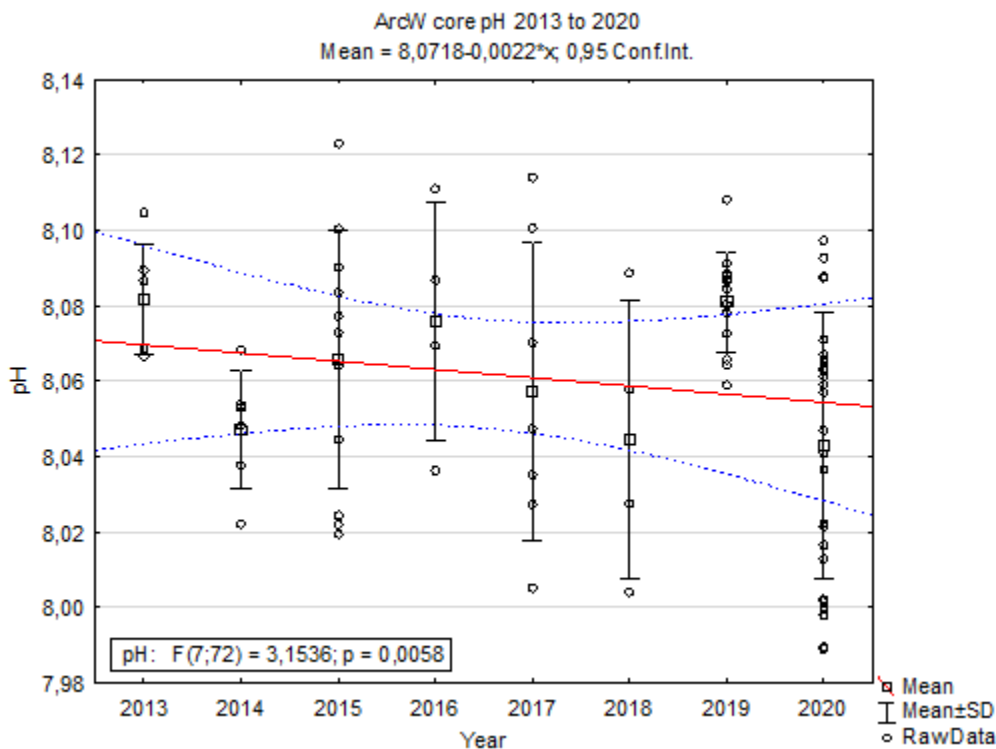
Figure A.41.1 The time series of pH in the period 2013 to 2020 in the Arctic core waters ( T < 0^\circ\text{C} ). The linear fit (red line) is based on annual mean pH values (black squares) from observational data (circles). The blue hashed lines denote the area of 95% confidence.
