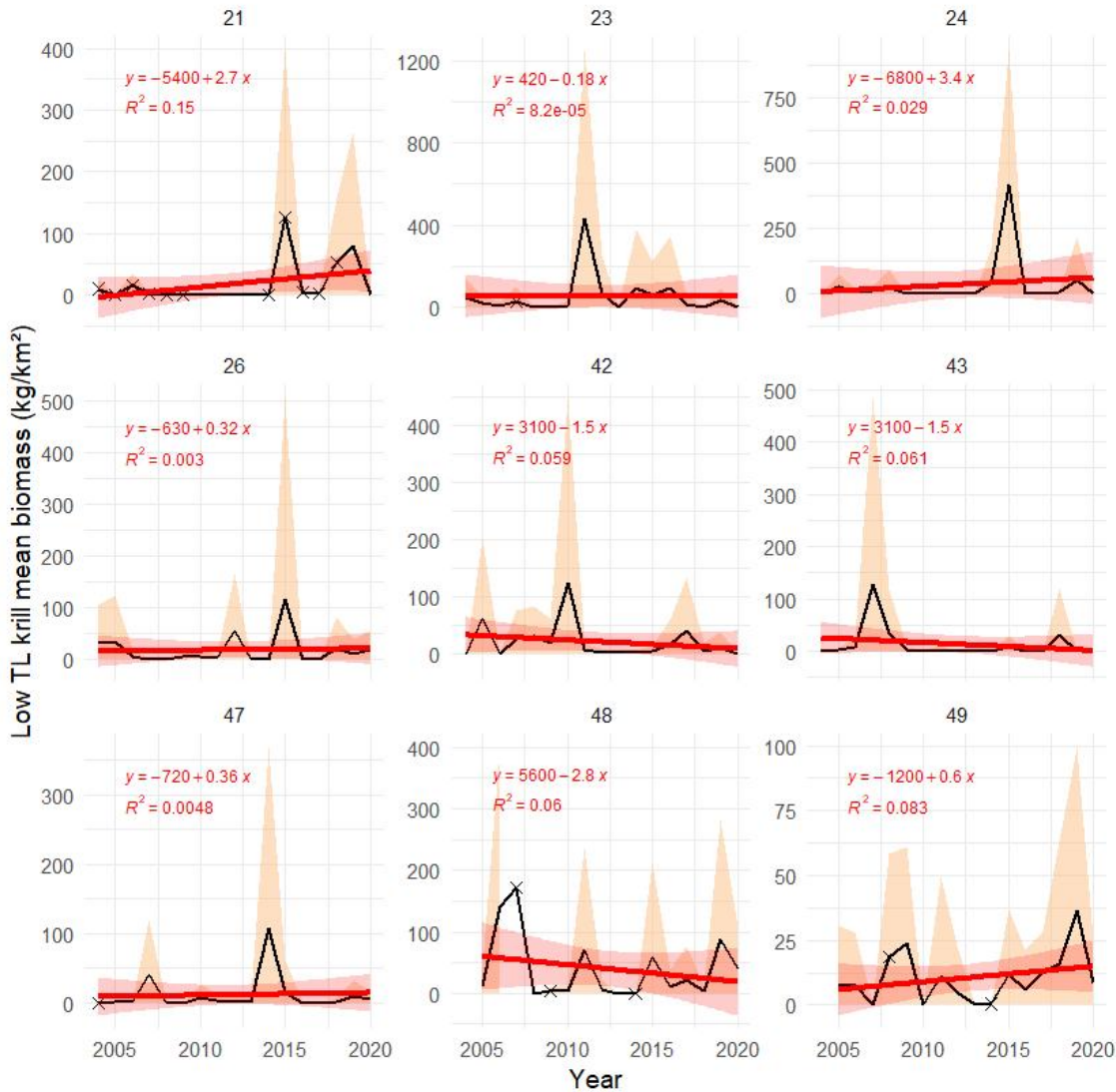
Figure A.3.3 Mean biomass / km 2 of low trophic level krill (Kg km -2 wet wt) in each polygon in the Arctic part of the Barents Sea (number on top of each panel) with \pm 1 SD indicated with light shading. Red line and dark shaded areas indicate fitted linear trend and 95% confidence bands, with equation and R^2 indicated in red. Stars denote years with low sample size (< 5 trawls).
