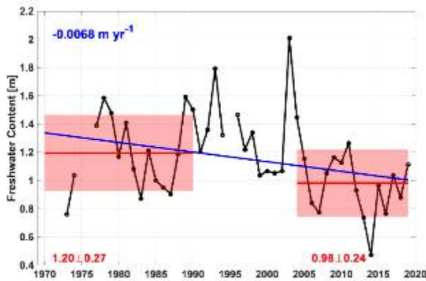
Figure A.39.1 The time series of estimated freshwater content. Means and standard deviations for 1970-1990 and 2004-2019 are shown by red lines and pale red boxes with actual shown in red. Linear trends 1970-2019 and 2004-2019 are shown in blue when statistically significant at the 95% level (with actual values also in blue).
