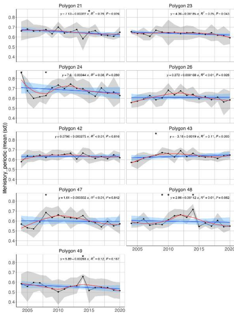
Figure A.16.5 Mean ( \pm sd) log biomass proportion of the periodic life history strategy excluding cod in the Arctic part of the Barents Sea (Black dots and grey shading). Linear regression fit with 95% CI is shown in blue, and the statistical results are given in the top of each plot. A local smoother is added in red to assist visual interpretation of non-linear changes during the period. Stars denote years with low sample size (< 5 trawls). A) in the whole area. B) per polygons.
