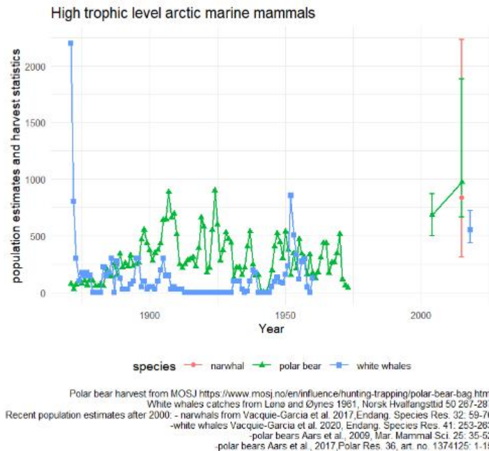
Figure A.12.1: recent population estimates and catch and harvest statistics for high trophic levels marine mammals
