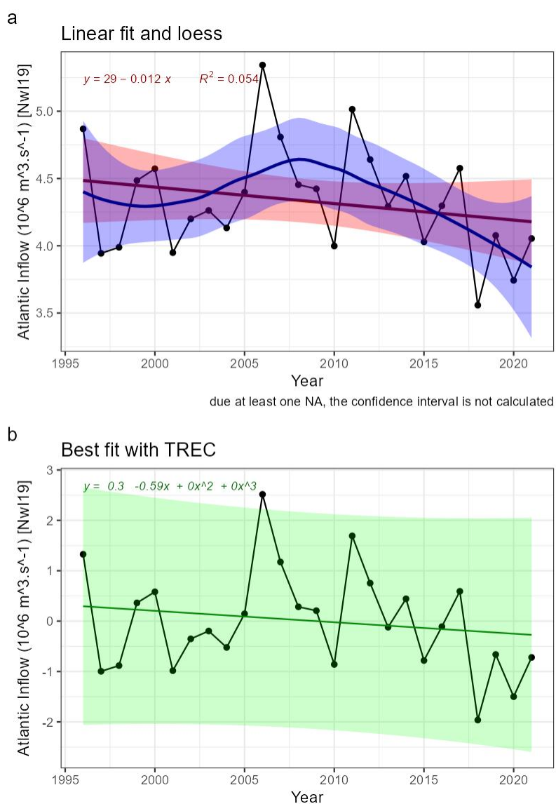
Fig. 19: Indicator time series and fitted trends. A) linear trend fitted with Least-square method (not adapted for short time series) in red, and loess in blue, for information. B) Best fitted trend using the first steps of a TREC analysis on scaled time series
