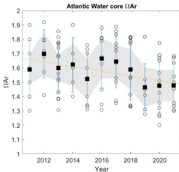
Fig.22: The time series of aragonite saturation ( \Omega Ar ) in the period 2011 to 2021 in the Atlantic Water (salinity ^3 34.9, temperature ^3 0°C, depth ^3 200 m) in the Norwegian Sea. The linear regression fit (orange line; gradient = -0.0164 \pm 0.0060 , p = 0.0239 , R^2 = 0.45 ) is based on annual mean \Omega Ar values (black squares) from observational data (circles). Bars are \pm 1 standard deviation for each annual mean. The grey shaded area represents the 95% confidence limits.
