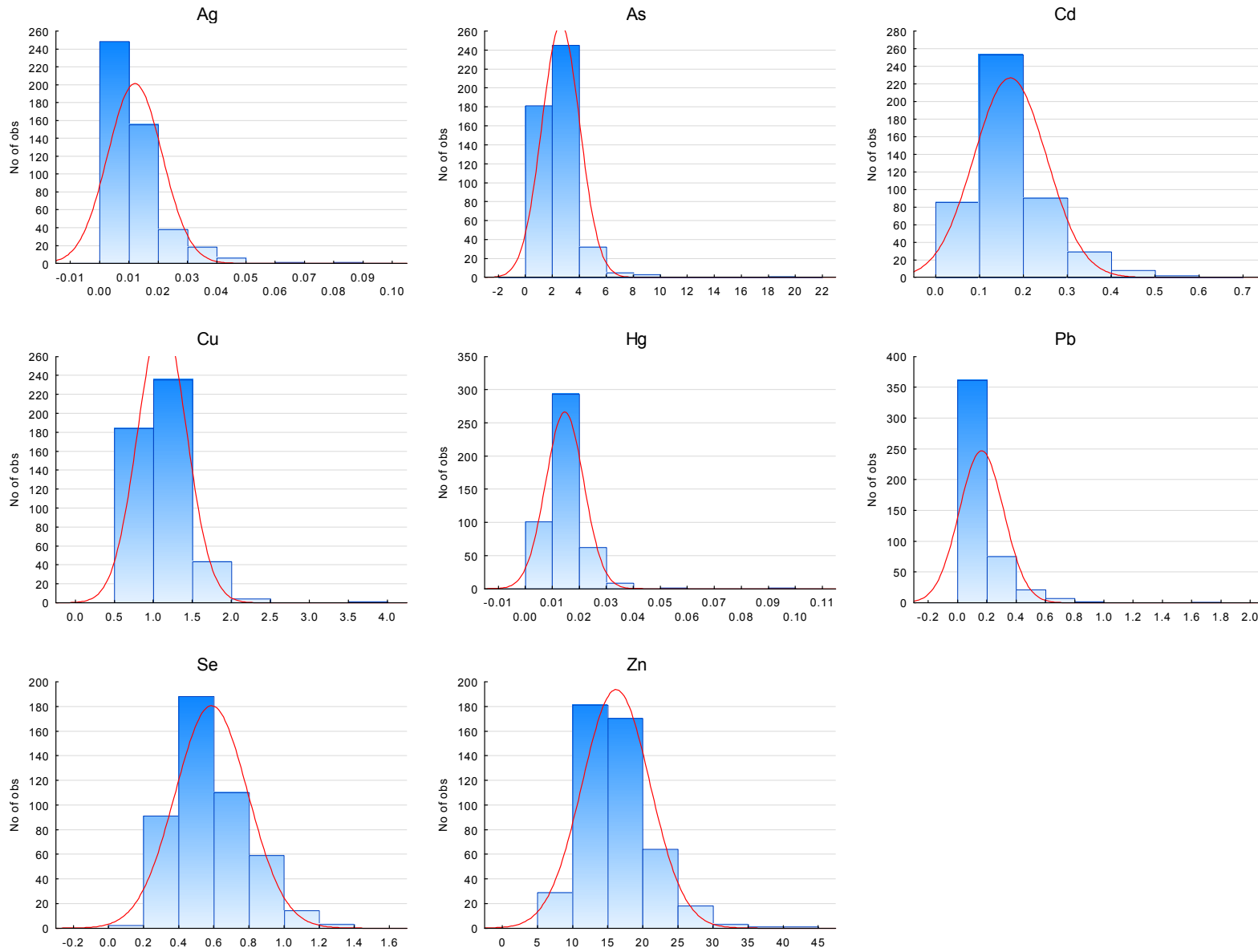
Figur 1. Histograms showing the distribution of metal concentrations in mussels ( Mytilus edulis ) from the shellfish monitoring programme between 2005 and 2014. All concentrations are given as mg/kg wet weight.
