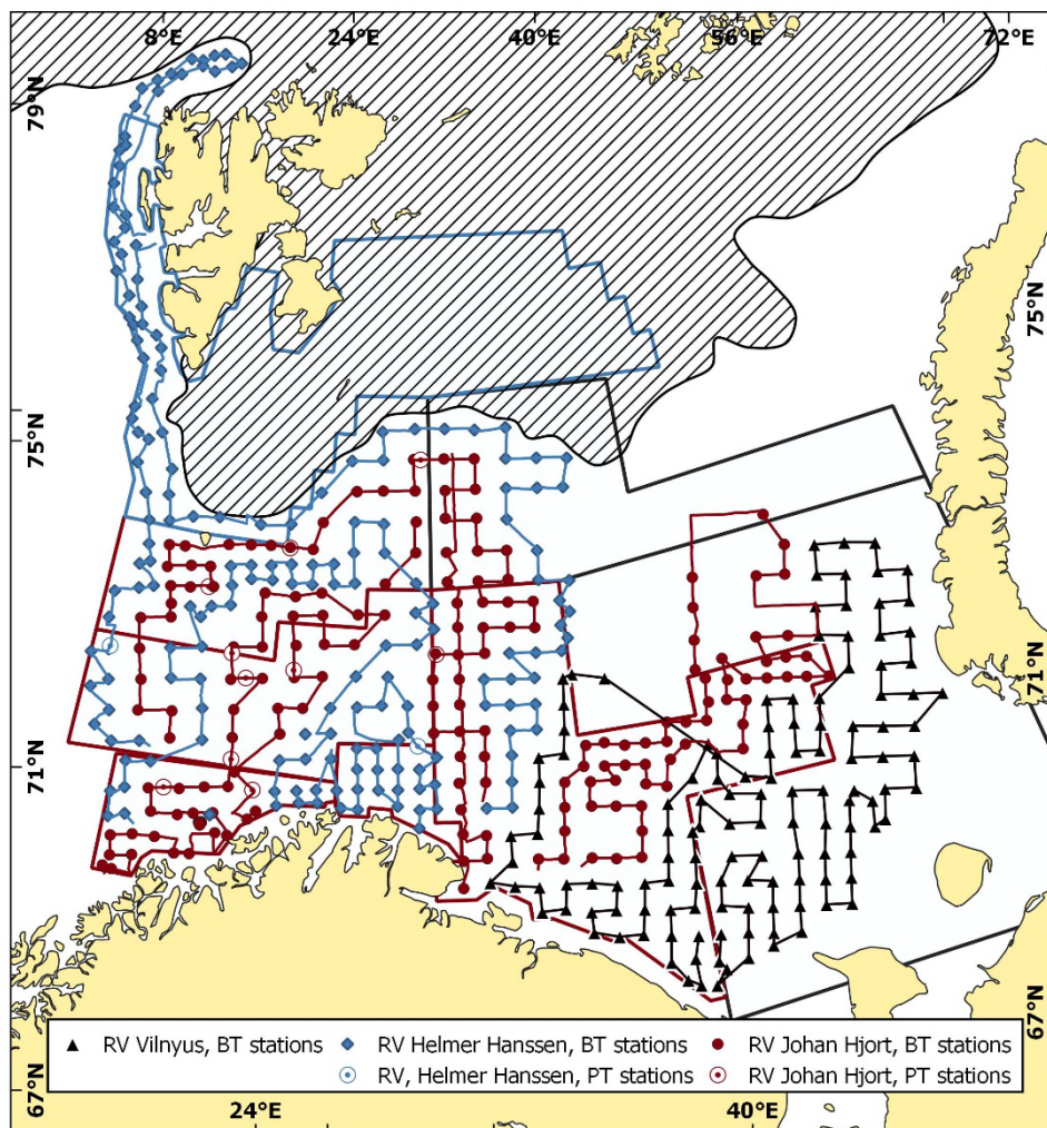
Figure 3.1. Survey tracks and all trawl stations in the winter survey 2020. Data source for the ice cover: https://cryo.met.no/archive/ice-service/icecharts/quicklooks/2020/
