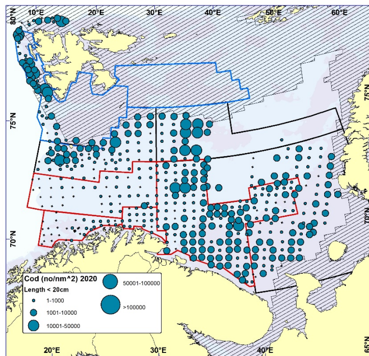
Figure 5.1. COD < 20 cm. Distribution in valid bottom trawl catches winter 2020 (number per \text{nm}^2 ). Black crosses indicate zero catches. Data source for the ice cover: https://cryo.met.no/archive/ice-service/icecharts/quicklooks/2020/
