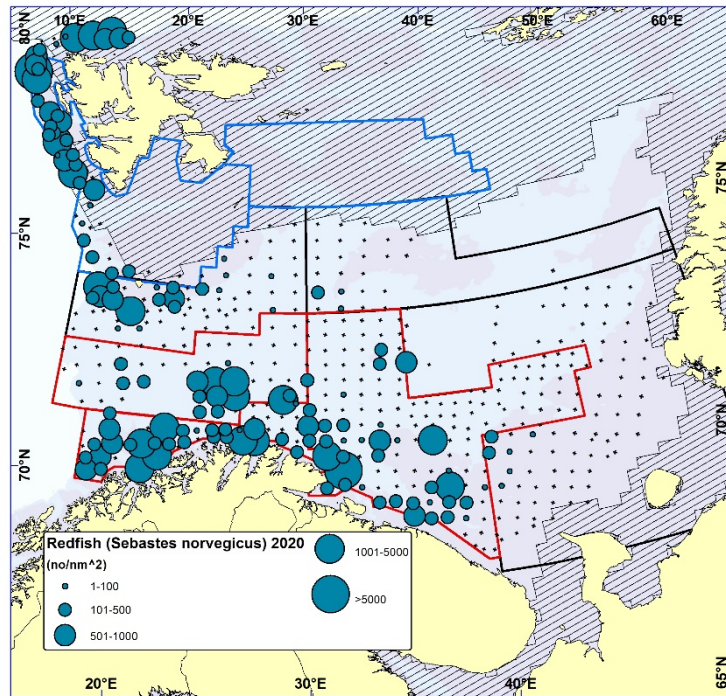
Figure 7.1. GOLDEN REDFISH ( Sebastes norvegicus ). Distribution in the trawl catches winter 2020 (number per \text{nm}^2 ). Black crosses indicate zero catches.
