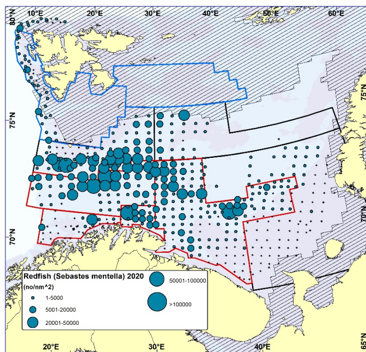
Figure 7.2. BEAKED REDFISH ( Sebastes mentella ). Distribution in the trawl catches winter 2020 (number per \text{nm}^2 ). Black crosses indicate zero catches.
