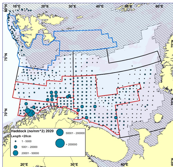
Figure 6.1. HADDOCK < 20 cm. Distribution in valid bottom trawl catches winter 2020 (number per nm 2 ). Black crosses indicate zero catches.
