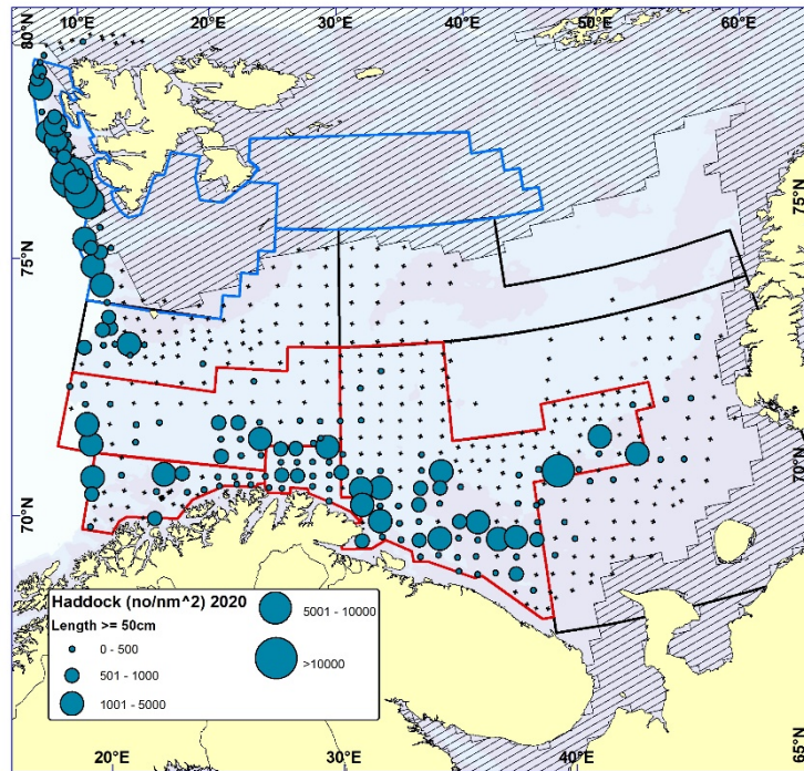
Figure 6.4. HADDOCK \geq 50 cm. Distribution in valid bottom trawl catches winter 2020 (number per \text{nm}^2 ). Black crosses indicate zero catches.
