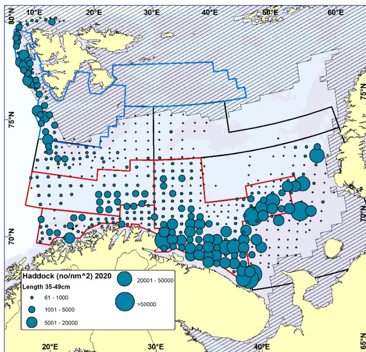
Figure 6.3. HADDOCK 35-49 cm. Distribution in valid bottom trawl catches winter 2020 (number per \text{nm}^2 ). Black crosses indicate zero catches.
