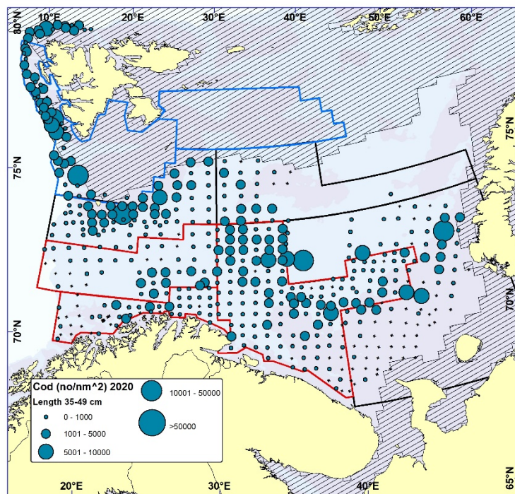
Figure 5.3. COD 35-49 cm. Distribution in valid bottom trawl catches winter 2020 (number per \text{nm}^2 ). Black crosses indicate zero catches.
