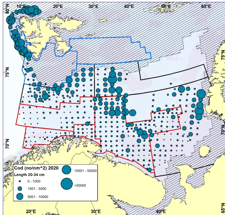
Figure 5.2. COD 20-34 cm. Distribution in valid bottom trawl catches winter 2020 (number per \text{nm}^2 ). Black crosses indicate zero catches.
