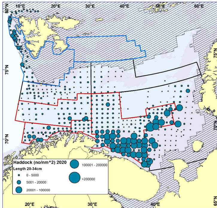
Figure 6.2. HADDOCK 20-34 cm. Distribution in valid bottom trawl catches winter 2020 (number per \text{nm}^2 ). Black crosses indicate zero catches.
