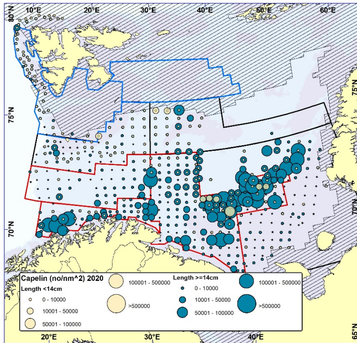
Figure 9.1. CAPELIN. Distribution in the trawl catches winter 2020 (number per nm 2 ). Black crosses indicate zero catches.
