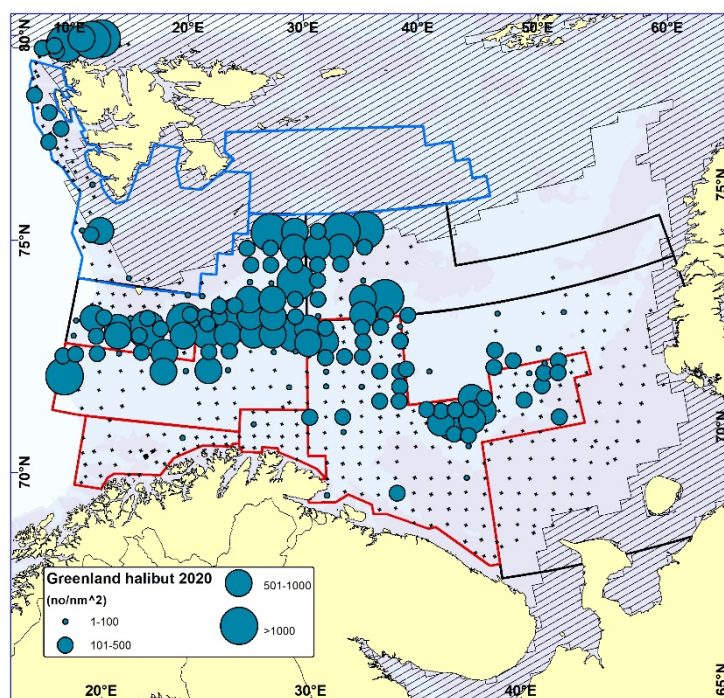
Figure 8.1 GREENLAND HALIBUT. Distribution in the trawl catches winter 2020 (number per \text{nm}^2 ). Black crosses indicate zero catches.
