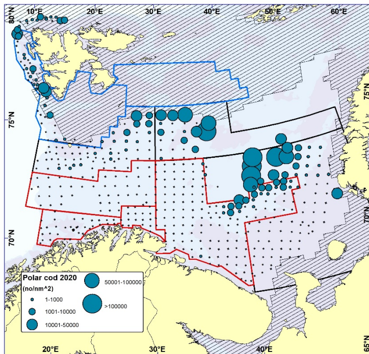
Figure 9.2 POLAR COD. Distribution in the trawl catches winter 2020 (number per nm 2 ). Black crosses indicate zero catches.
