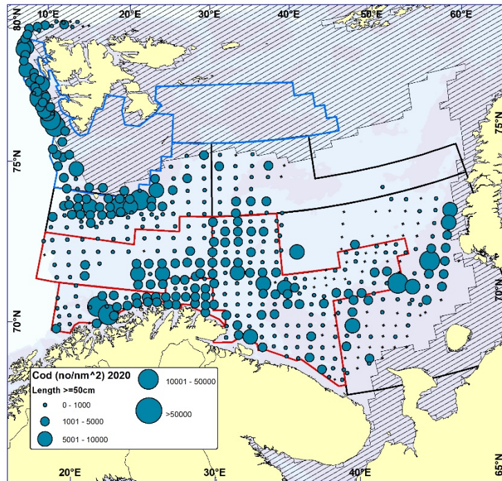
Figure 5.4. COD \geq 50 cm. Distribution in valid bottom trawl catches winter 2020 (number per \text{nm}^2 ). Black crosses indicate zero catches.
