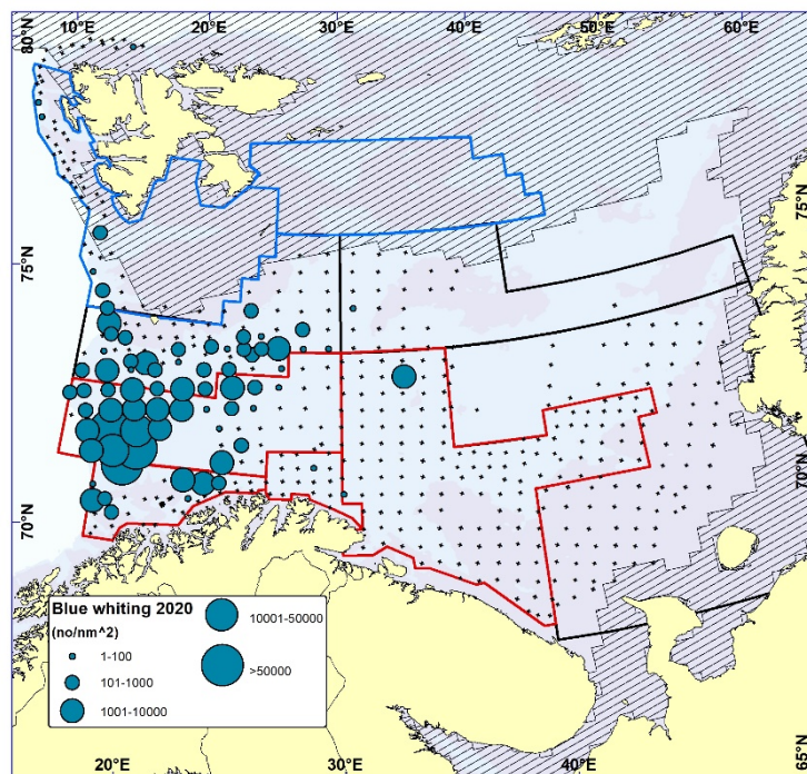
Figure 9.3 BLUE WHITING. Distribution in the trawl catches winter 2020 (number per \text{nm}^2 ). Black crosses indicate zero catches.
