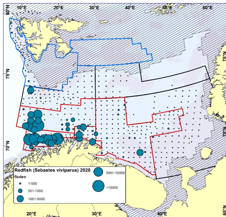
Figure 7.3. NORWAY REDFISH ( Sebastes viviparus ). Distribution in the trawl catches winter 2020 (number per nm 2 ). Black crosses indicate zero catches.
