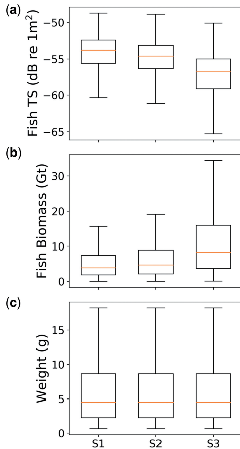
Figure 5. Summarized mesopelagic fish biomass model results for each scenario. (a) Mean fish TS = 10\log_{10}(\sigma_{b_{sf}}) , (b) global fish biomass, and (c) mean individual fish weight. Scenario 1 (S1) all fish have gas bladders, whereas in scenarios 2 (S2) and 3 (S3), a proportion of fish are without gas bladders. Horizontal line within each box is the median value, box limits are the inter-quartile range, i.e. 25 and 75% quantiles. The whiskers (vertical lines) are 1.5 times the inter-quartile range. Outliers not plotted.
