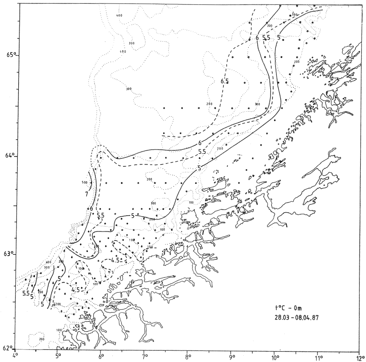
Fig. 2. Surface temperature, 28 March - 8 April 1987.
