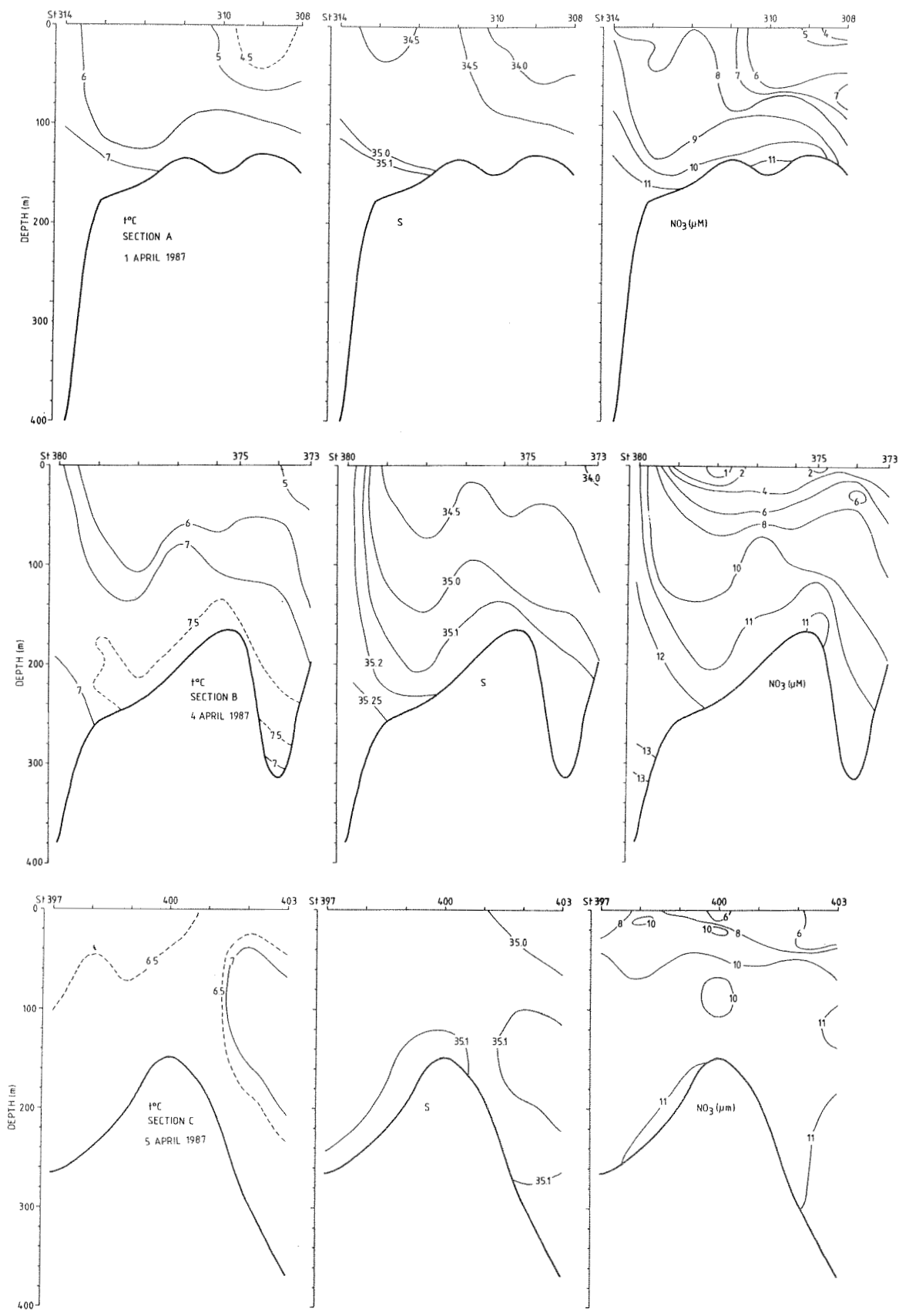
Fig. 5. Hydrographic sections A, B and C. The location of these is indicated in Fig. 1.
