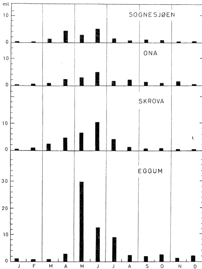
Fig. 10. Seasonal variations in the volumes of net plankton, 0—50 m, at the stations Sognesjøen, Ona, Skrova and Eggum. (Redrawn after WIBORG 1954, Fig. 24.)
