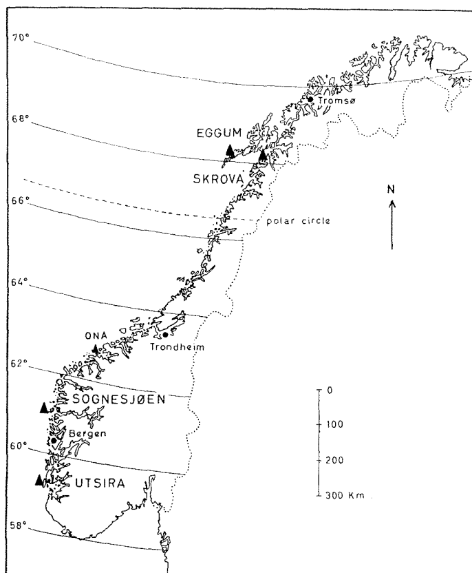
Fig. 1. The permanent oceanographic stations Utsira, Sognesjøen, Ona, Skrova and Eggum.
