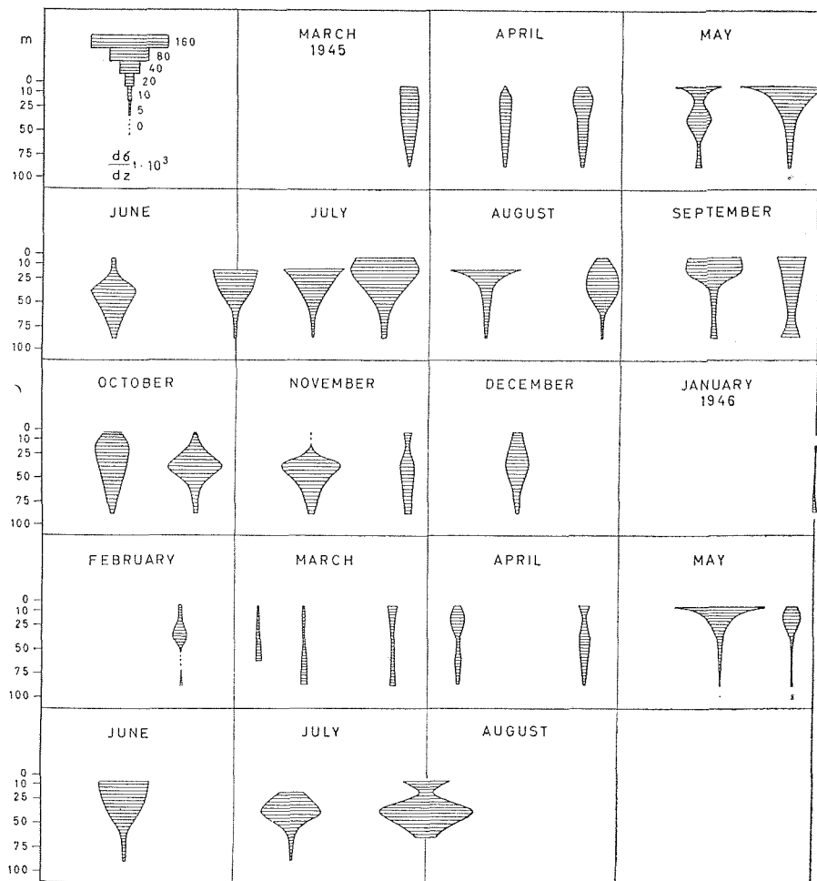
Fig. 3. Stability diagrams for station Sognesjøen during the period of investigation.
