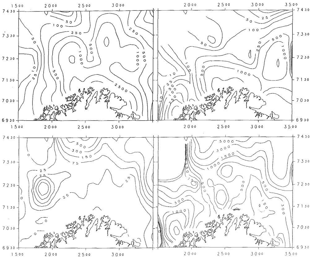
Fig. 8. Isolines for the amount of capelin (in 10 kg per square nautical mile) in the southern part of the Barents Sea during the period January–April. Upper part: Catches by Norway. Left, 1977. Right, 1984. Lower part: Resources calculated. Right 1984. Left, 1986. The two figures to the right are comparable. In the southern part of the Barents Sea, where the Norwegian capelin winter fisheries mostly take place, there is good agreement between the available resources and the catches.
