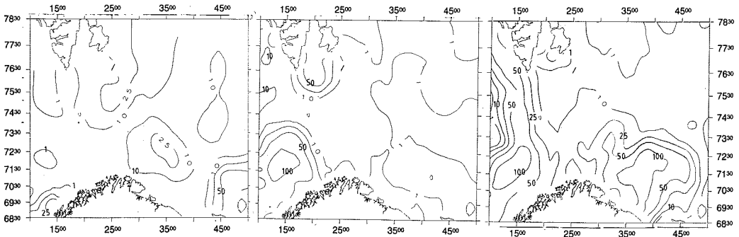
Fig. 7. Integrator values of "plankton" in the Barents Sea, average 1983–1987. Left, January–April. Middle, May–August. Right, September–October.
