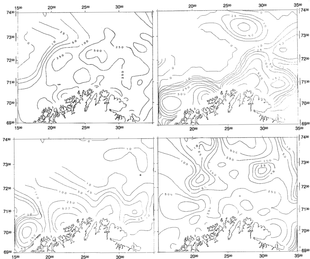
Fig. 13. Spawning migration of cod and haddock in the southern Barents Sea, winter 1985. Upper left, resources in February. Upper right, modelling result for migration 59 days from February in one step at the "preference" temperature 5.5°C. Lower left, same but the migration is carried out in two steps in the model. Lower right, resources in April same year.
