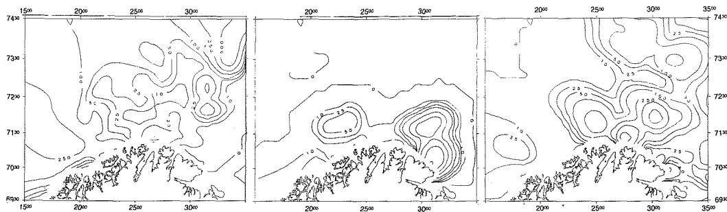
Fig. 11 Spawning migration of capelin in the southern Barents Sea, winter 1985. Left, resources in February. Middle, model prediction of resources 89 days after February, assuming the "preference" temperature 3.5^{\circ}\text{C} . Right, observed resources in May same year.
