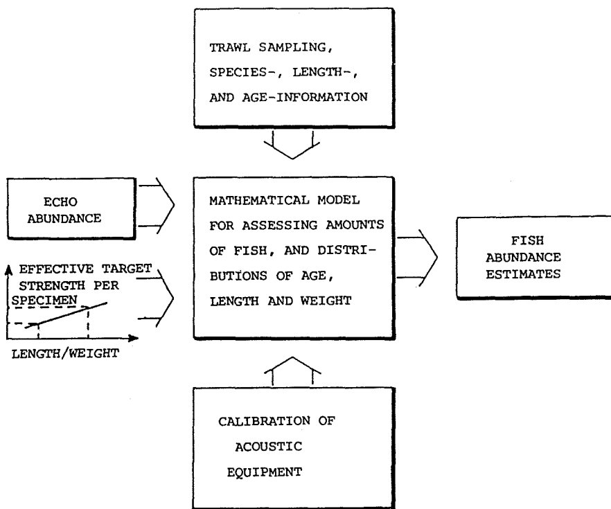
Fig. 4. The processes of the extended acoustic method for fish abundance estimation (Dalen and Smedstad, 1983).
