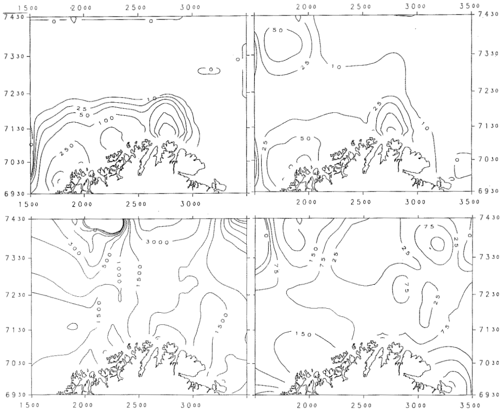
Fig. 10 Isolines (in 10 kg per square nautical mile) for the catches in the cod fisheries (upper part) and the resources of cod and haddock (lower part) in the southern part of the Barents Sea. Left, January–April 1985. Right, September–December 1984.
