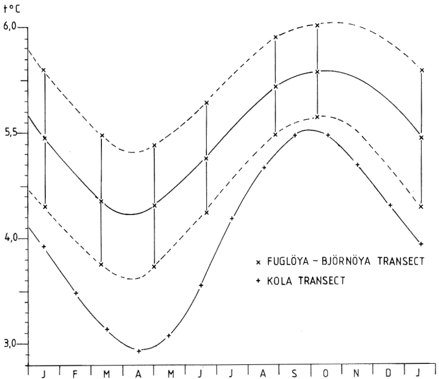
Fig. 2. Calculated average temperatures in degrees Celsius at 50–200 m depth for various months along the Fugløya-Bjørnøya (Bear Island) transect of the Barents Sea in the period 1977–1986 (dotted lines indicate the standard deviation), and for the Kola transect at 0–200 m depth in the period 1921–1980 (H. Loeng, pers. comm.).
