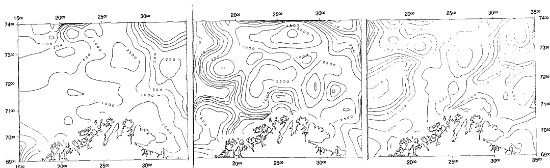
Fig. 14. "Feeding migration" of immature cod and haddock in the southern Barents Sea, summer 1985. Left, resources in May. Middle, modelling result for migration 153 days from May in one step at the "preference" temperature 3.0°C. Right, resources in October same year.
