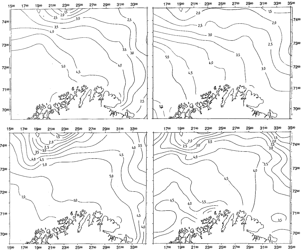
Fig. 6. Average sea temperatures at 50–200 m depth in the southern Barents Sea in May (top) and October (bottom). Left, 1984. Right, 1987.
