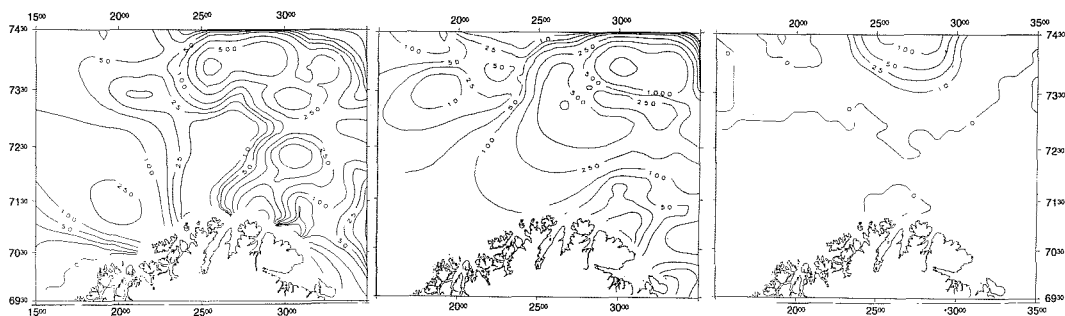
Fig. 12. "Feeding migration" of immature capelin in the southern Barents Sea, summer 1985. Left, modelling result for migration 123 days from May, assuming the "preference" temperature 3.5^{\circ}\text{C} . Middle, same, but at the temperature 1^{\circ}\text{C} . Right, observed resources in September same year.
