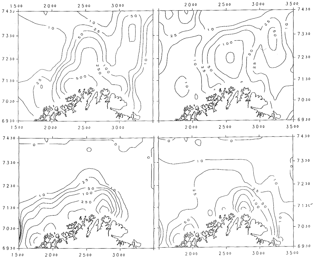
Fig. 9. Isolines for the catches in the cod fisheries (in 10 kg per square nautical mile) in the southern part of the Barents Sea. Upper part, 1976, lower part, 1981. Left, January–April. Right, September–December.
