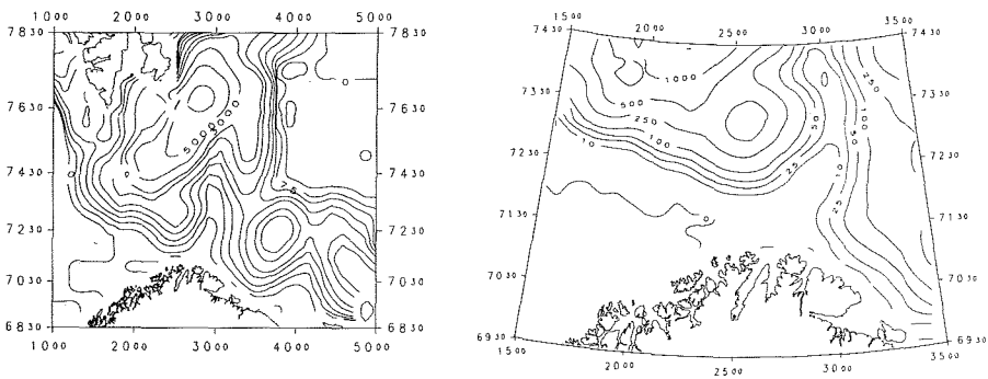
Fig. 3. Left. Map in Mercator projection for a large sector of the Barents Sea. Isolines of total capelin resources in September–December 1983 given in 10 kg per square nautical mile. Right. Map in UTM projection for a relatively small sector of the Barents Sea. Isolines of young capelin resources in September 1983 in 10 kg per square nautical mile.
