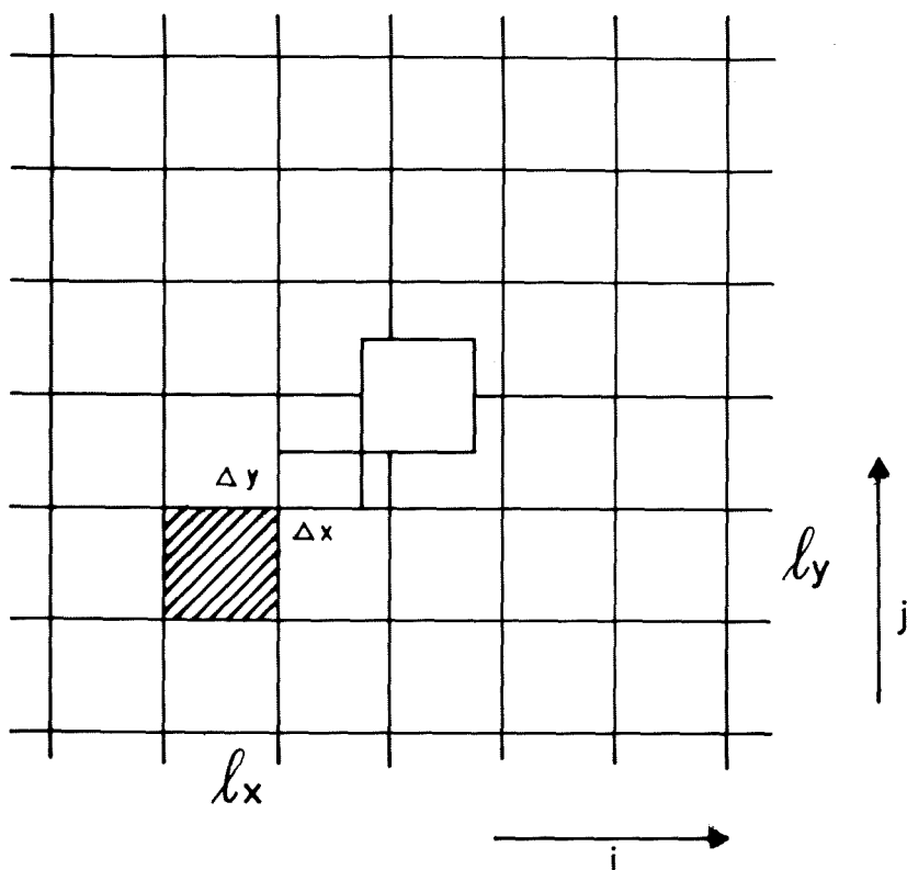
Fig. 5. Some squares in the 100 by 80 data matrix of the Barents Sea area. Further explanation in the text.
