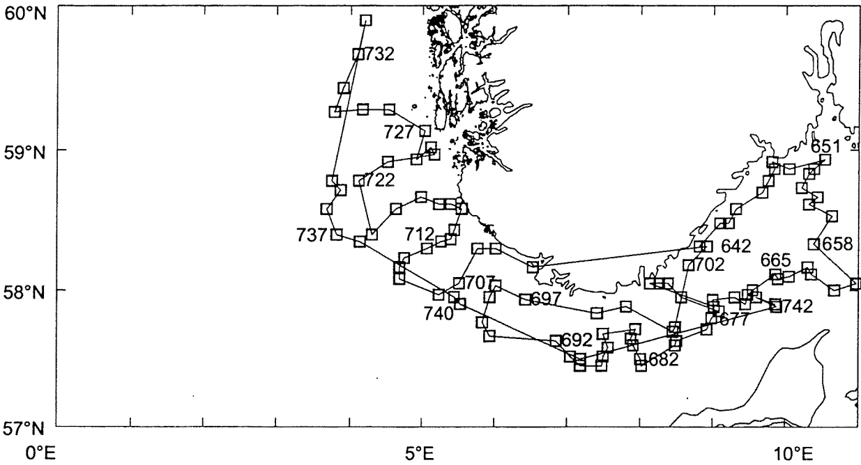
7 - 27 Oct 1998 Cruise no 1998113
