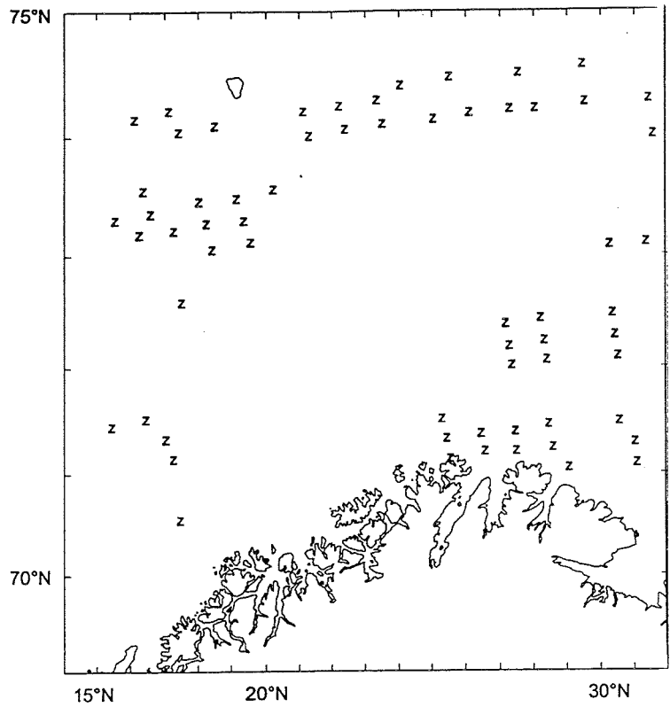
31 Jan - 24 Feb 1998 z CTD "Jan Mayen"
