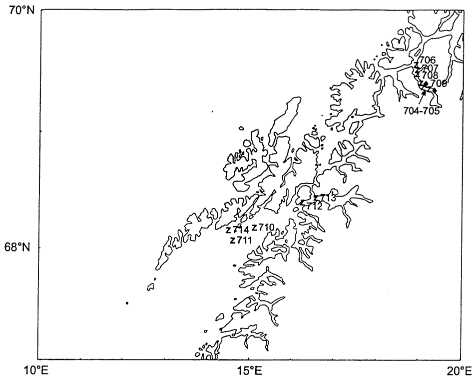
9 - 18 October 1998 z CTD st.no 704-715 "Johan Hjort" Cruise no 1998213 (st.715:62°41'N07°00'E) ♦ Mocness st.(at ctd st.705 and 709)
