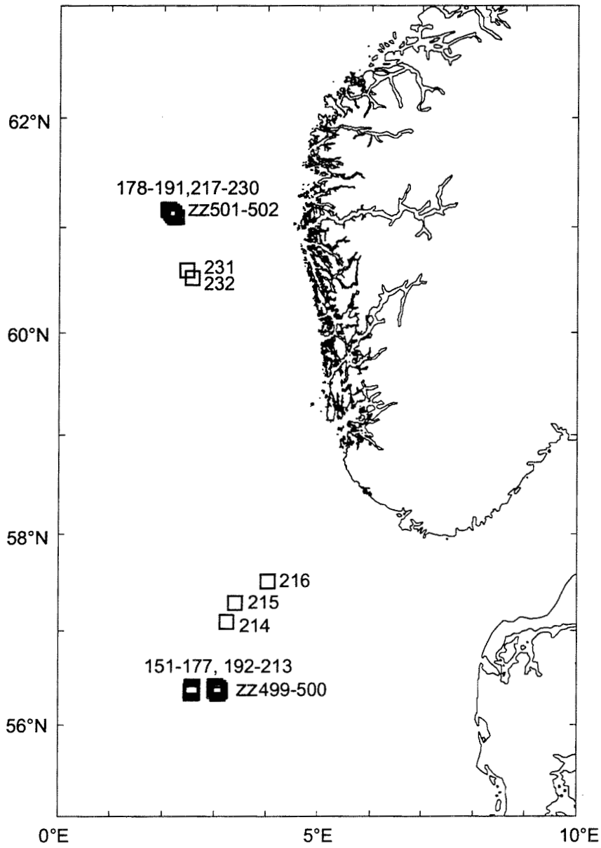
11 - 25 May 1998 □ Bottom TRAWL st.no 151-232 "Michael Sars" Cruise no 1998106 z CTD st.no 499-502
