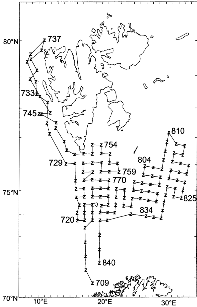
30 Jul - 22 Aug 1998 z CTD st.no 709-840 "Michael Sars" Cruise no 1998109
