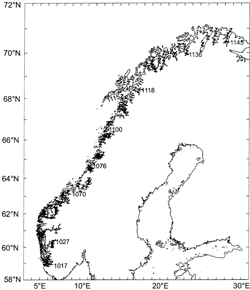
28 Oct - 10 Dec 1998 z CTD St.no 1017-1145 Michael Sars" Cruise no 1998114
