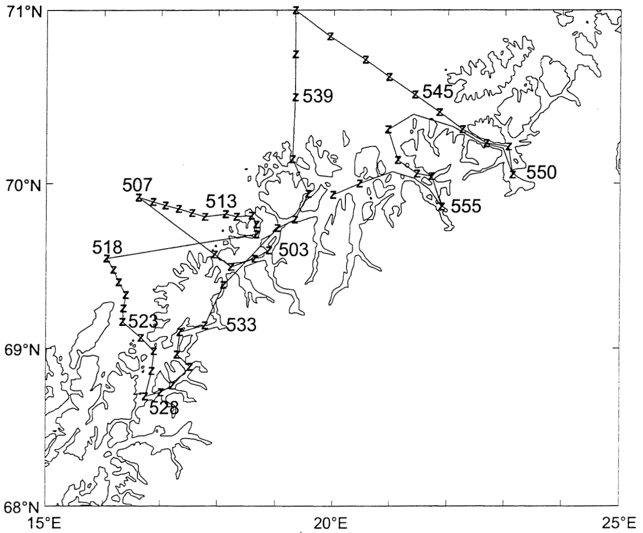
3-8 June 1998 z CTD st.no 503-557 "Michael Sars" Cruise no 1998116
