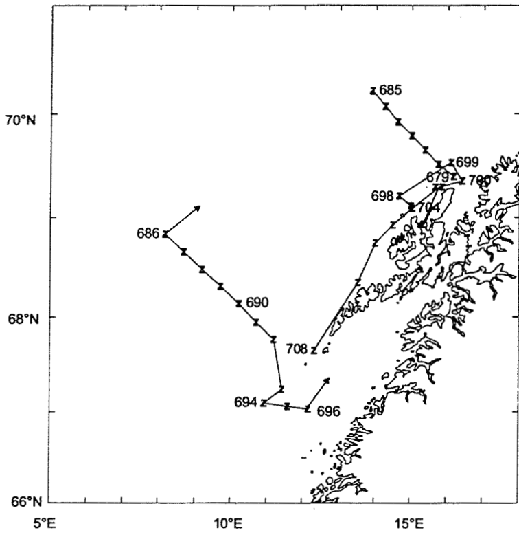
10-21 July 1998 z CTD St.no 679-708 "Michael Sars" Part II Cruise no 1998108
