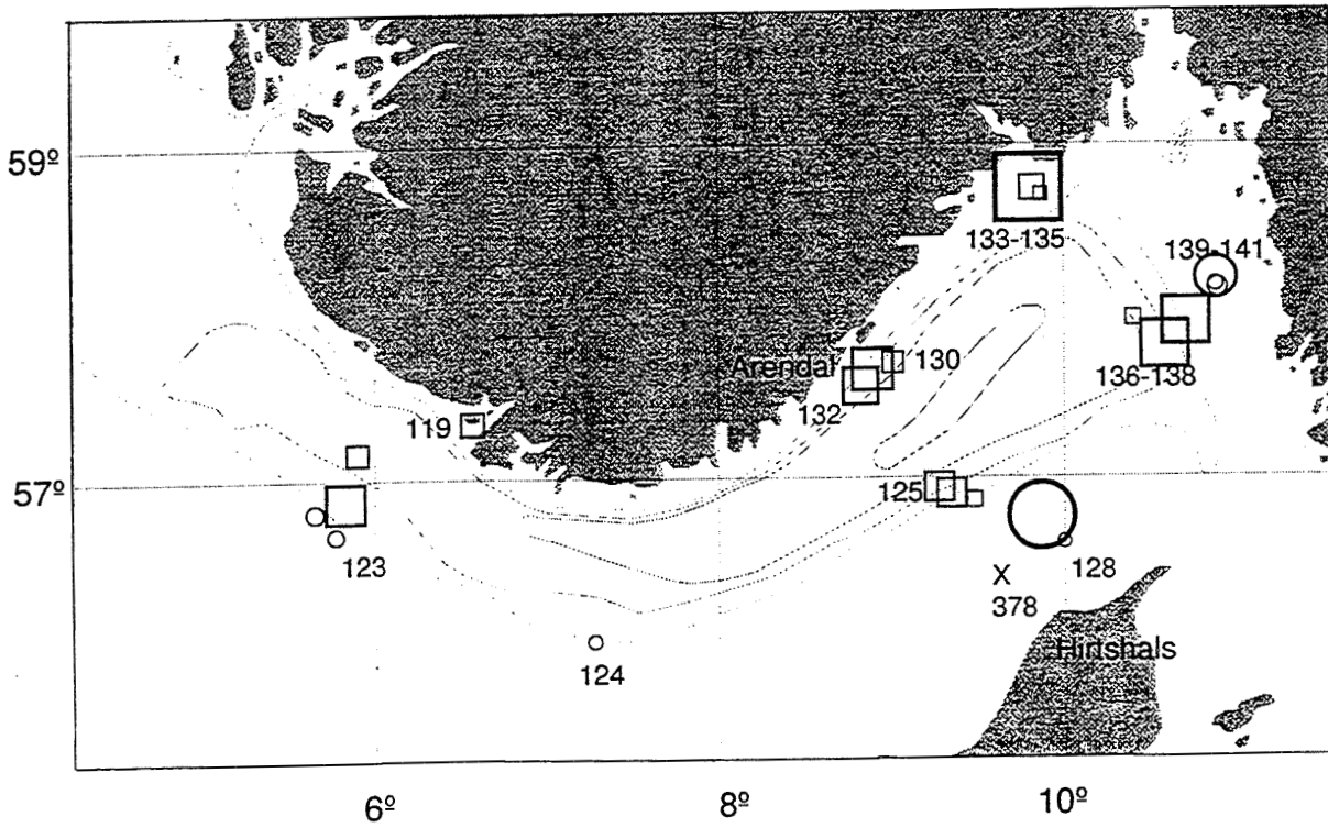
19 - 26 June 1998 TRAWL st.no 119-141 "G.M. Dannevig" Cruise no 1998329
