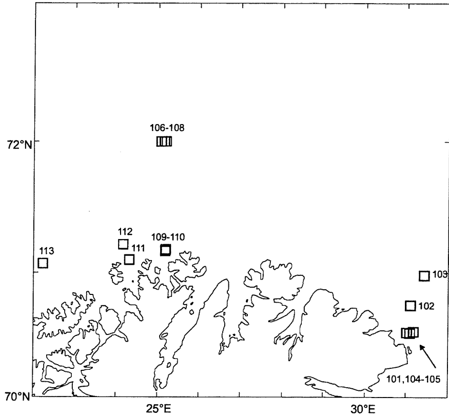
3-12 Mar 1998 Bottom TRAWL st.no 101-113 "G.O. Sars" Cruise no 1998003
