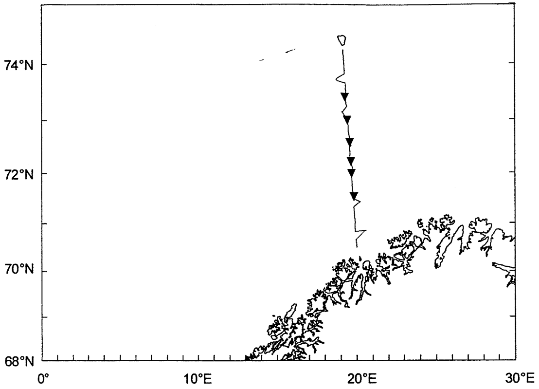
Deployed half-year mooring MAIA with current meters Cruise no 2000211
