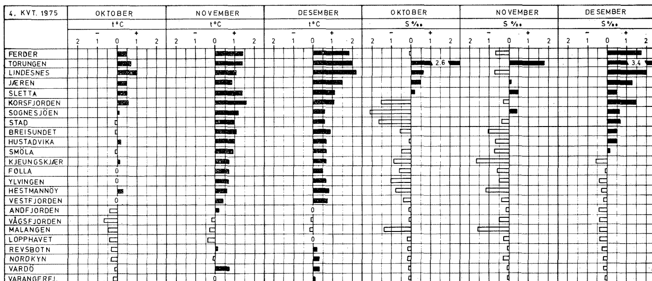
10 dagers middeltemperatur og månedsmiddel for saltholdighet langs Norskekysten i 4. kvartal 1975. [10 days mean temperature and monthly means of salinity along the Norwegian coast in 4 quarter of 1975].
