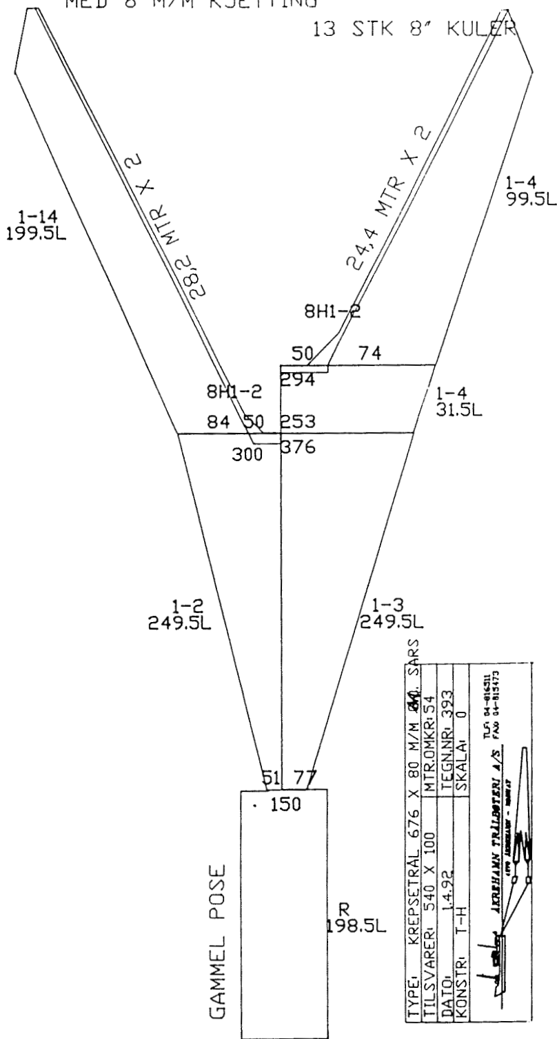
Figur 4. Krepsetrål, 676 masker i 80 mm [Nephrops trawl, 676 meshes in 80 mm].
