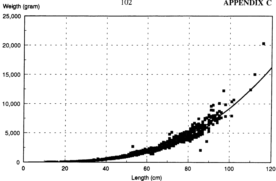
Figure 3. Length-weight relationship for cod in the southwestern part of the Barents Sea in 1992. Source: Demersal Fish Section, Institute of Marine Research. Fitted curve: w = 6.30 \cdot 10^{-3} L^{3.083} , weight w in grams, length L in centimeters.
