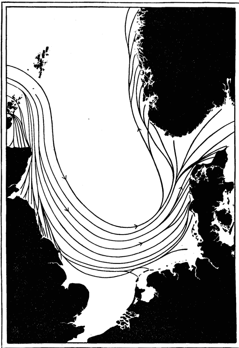
Fig. 35. Results of Dr. FULTON'S Drift bottle Experiments in the North Sea.
