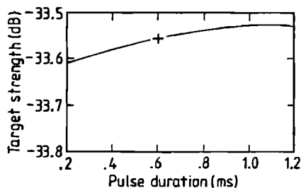
FIG. A4. Dependence of the target strength of the 60-mm copper sphere on the duration of the transmit pulse of the EK-38 echo sounder. The plus sign indicates a common datum with Figs. A2 and A3.
