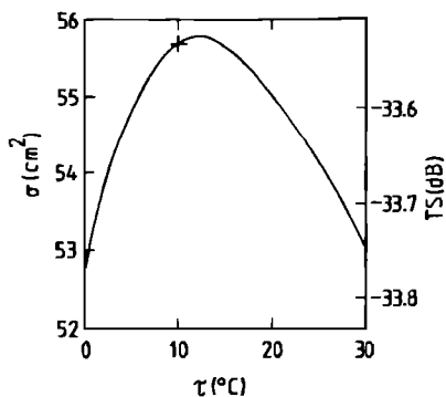
FIG. 3. Effects of variations in the medium temperature \tau on \sigma and TS of the examined calibration sphere. A constant medium salinity of 35 ppt is assumed. The plus indicates the numerical baseline.
