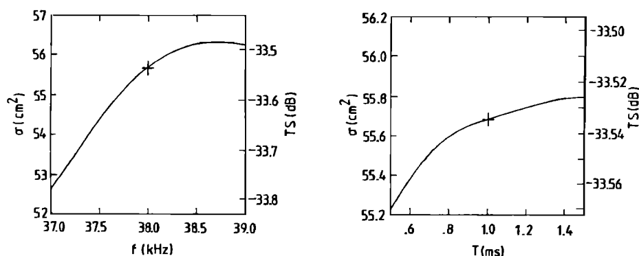
FIG. 4. Effects of variations in the center frequency f and duration T of the transmit pulse on \sigma and TS of the examined calibration sphere. The plus indicates the numerical baseline.
