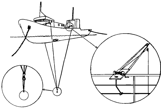
FIG. A1. Rigging of a research vessel for calibration.
