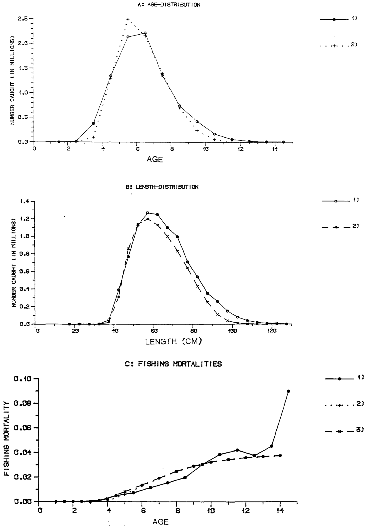
Fig. 5a-c. The UK trawlfishery in Division IIa. Numbers caught and fishing mortality. Legend: 1) Observed 2) Estimated from the age distributions 3) Estimated from the length distributions.
