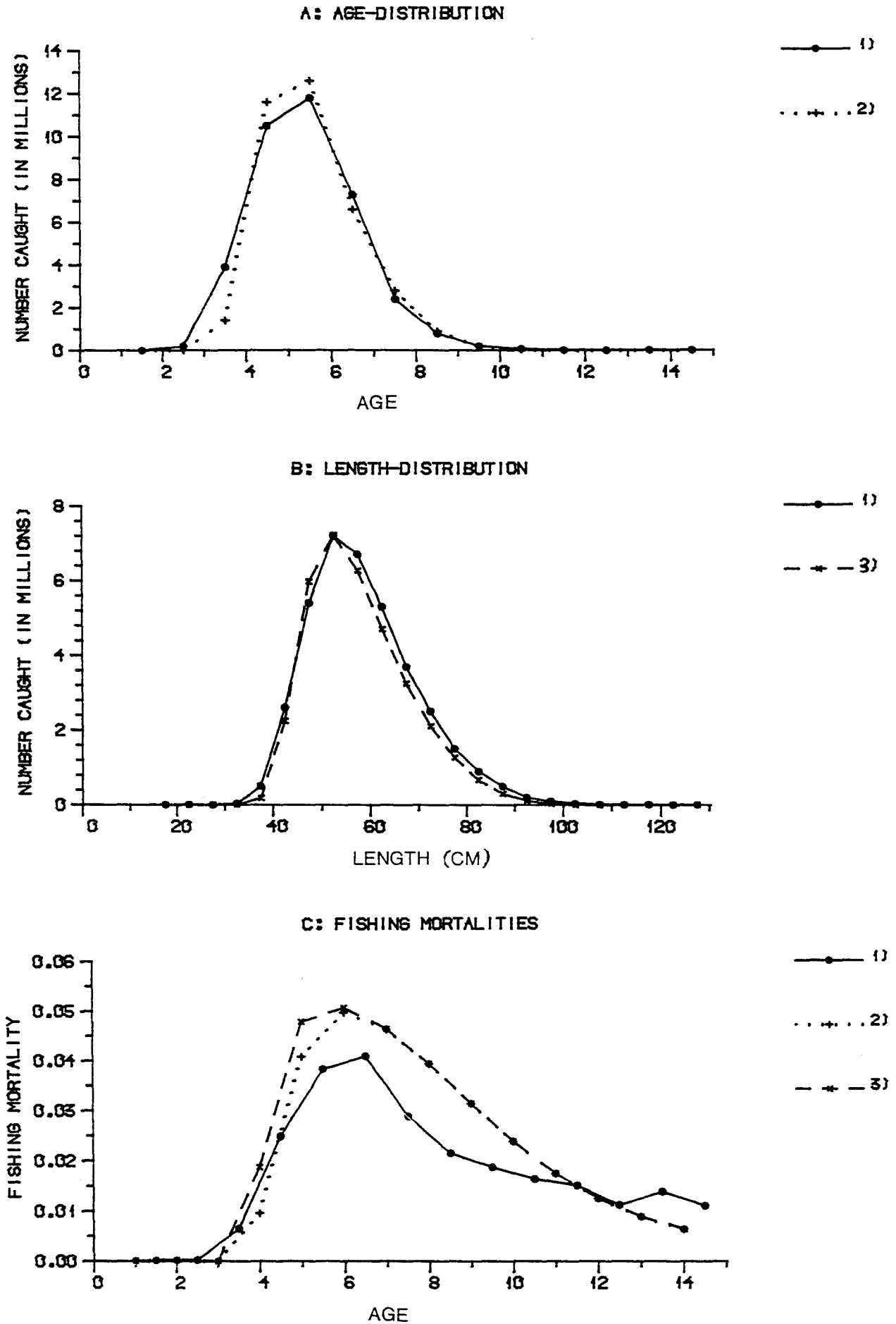
Fig. 4a-c. The UK trawlfishery in Sub-area I. Numbers caught and fishing mortality. Legend: Observed 2) Estimated from the age distributions 3) Estimated from the length distributions.
