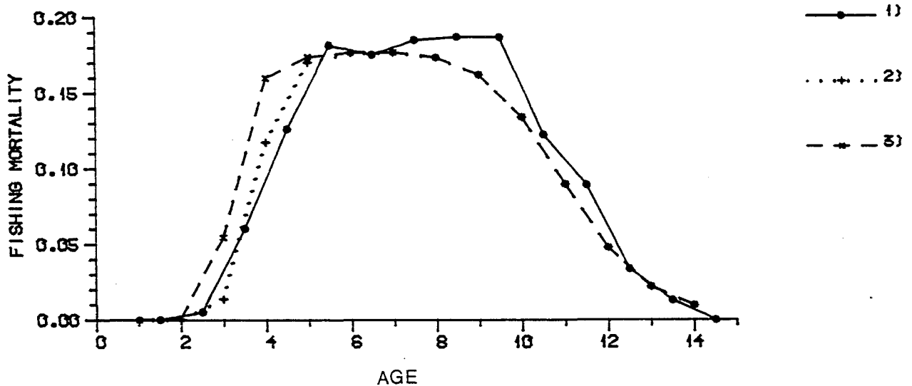
Fig. 2a-c. The USSR trawlfishery in Sub-area I. Numbers caught and fishing mortality. Legend: 1) Observed 2) Estimated from the age distributions 3) Estimated from the length distributions.
