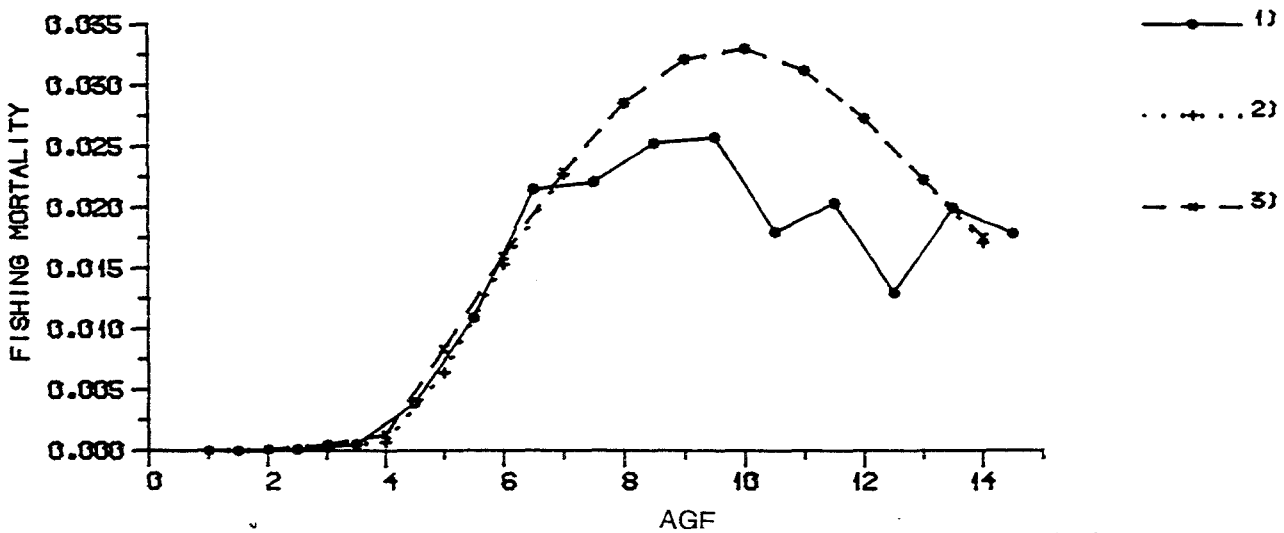
Fig. 9a-c. The Norwegian trawlfishery in Division IIIa. Numbers caught and fishing mortality. Legend: 1) Observed 2) Estimated from the age distributions 3) Estimated from the length distributions.
