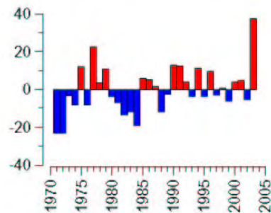
Figure 3: Annual mean biomass deviations from the long-term mean ( x = 37.2 \text{ ml/m}^3 ) of all biomass values.
