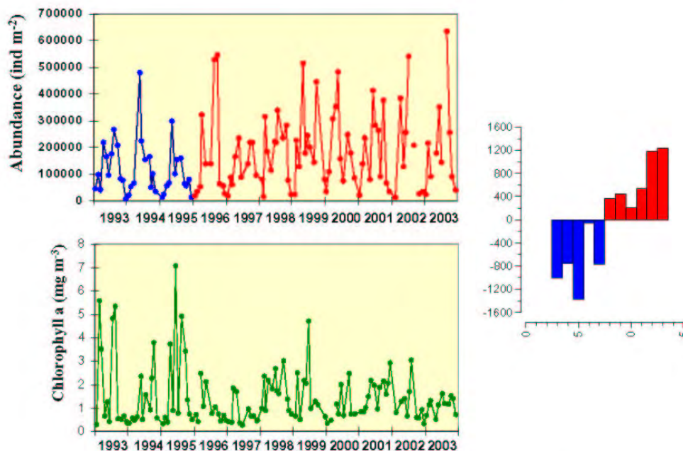
Figure 19: Left: Monthly zooplankton abundance (upper panel) and chlorophyll a in a neritic station off A Coruña. Right: Annual mean abundance deviations from the long-term mean ( \bar{x} = 2922 \text{ ind/m}^2 ) of all abundance values.
