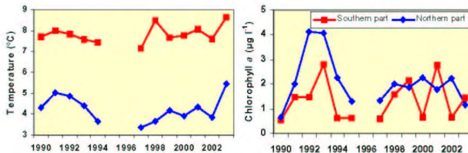
Figure 11. Temperature (left) and chlorophyll a (right) concentrations at 0-50 m depth on section North, May 1990-2003. The chl. a values for 2003 are preliminary.
