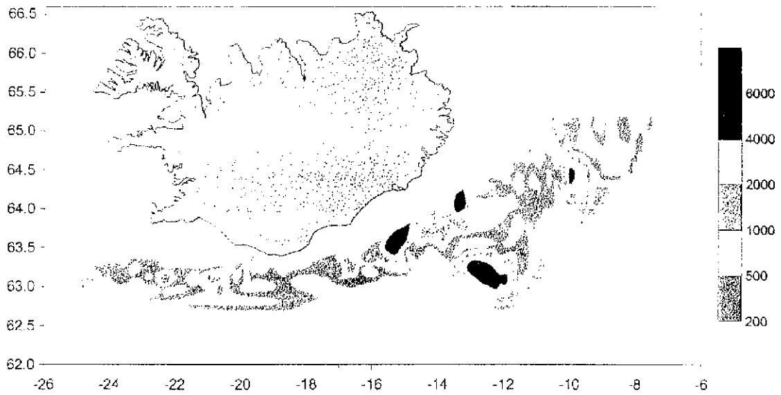
Figure 6. Cruise track of RV Árnir Friðriksson 21.06-06.07, 1999. Isolines are distribution of blue whiting represented by Sa values.
