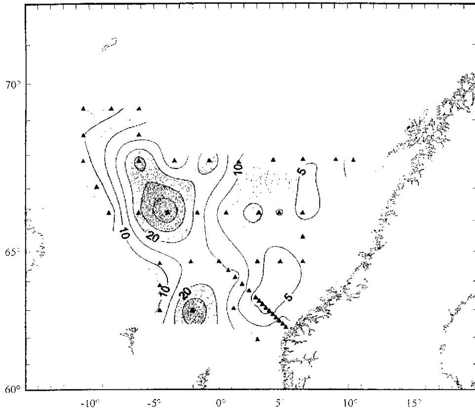
Figure 27. Zooplankton biomass [g dw*m -2 ] (200-0m) July-August 1999.
