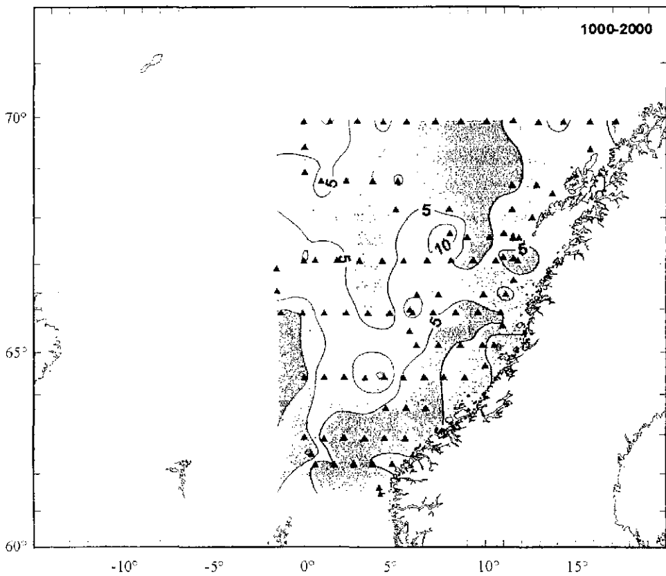
Figure 24. Zooplankton biomass in size fraction 1000-2000 \mu\text{m} [ \text{g dw}\cdot\text{m}^{-2} ] (200-0m) April-June 1999.
