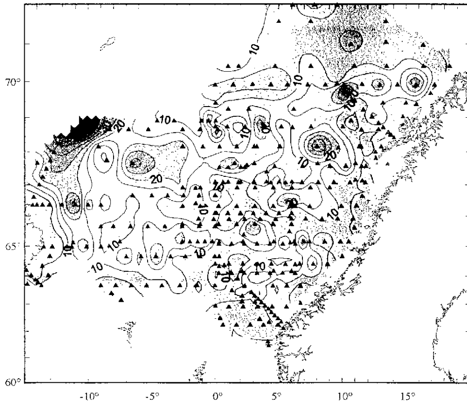
Figure 22. Zooplankton biomass [g dw·m -2 ] (200-0m) April-June 1999.
