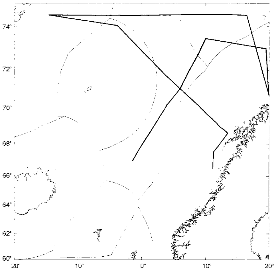
Figure 7. Cruise track of RV Johan Hjort 15.06-09.07, 1999.
