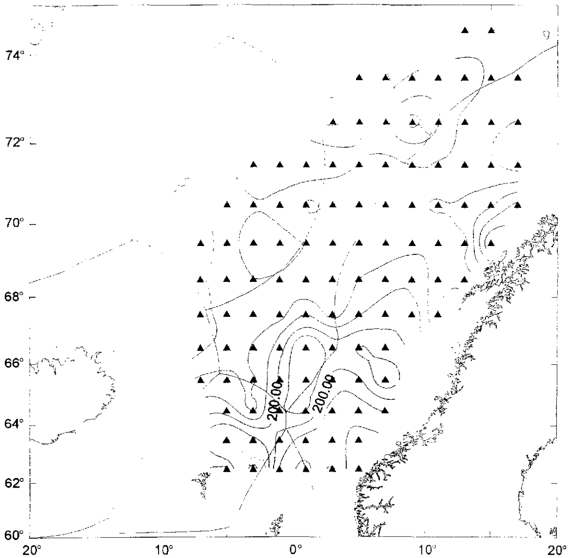
Figure 36. Distribution of blue whiting in July-August 1999 as measured by the RV G.O.Sars.
