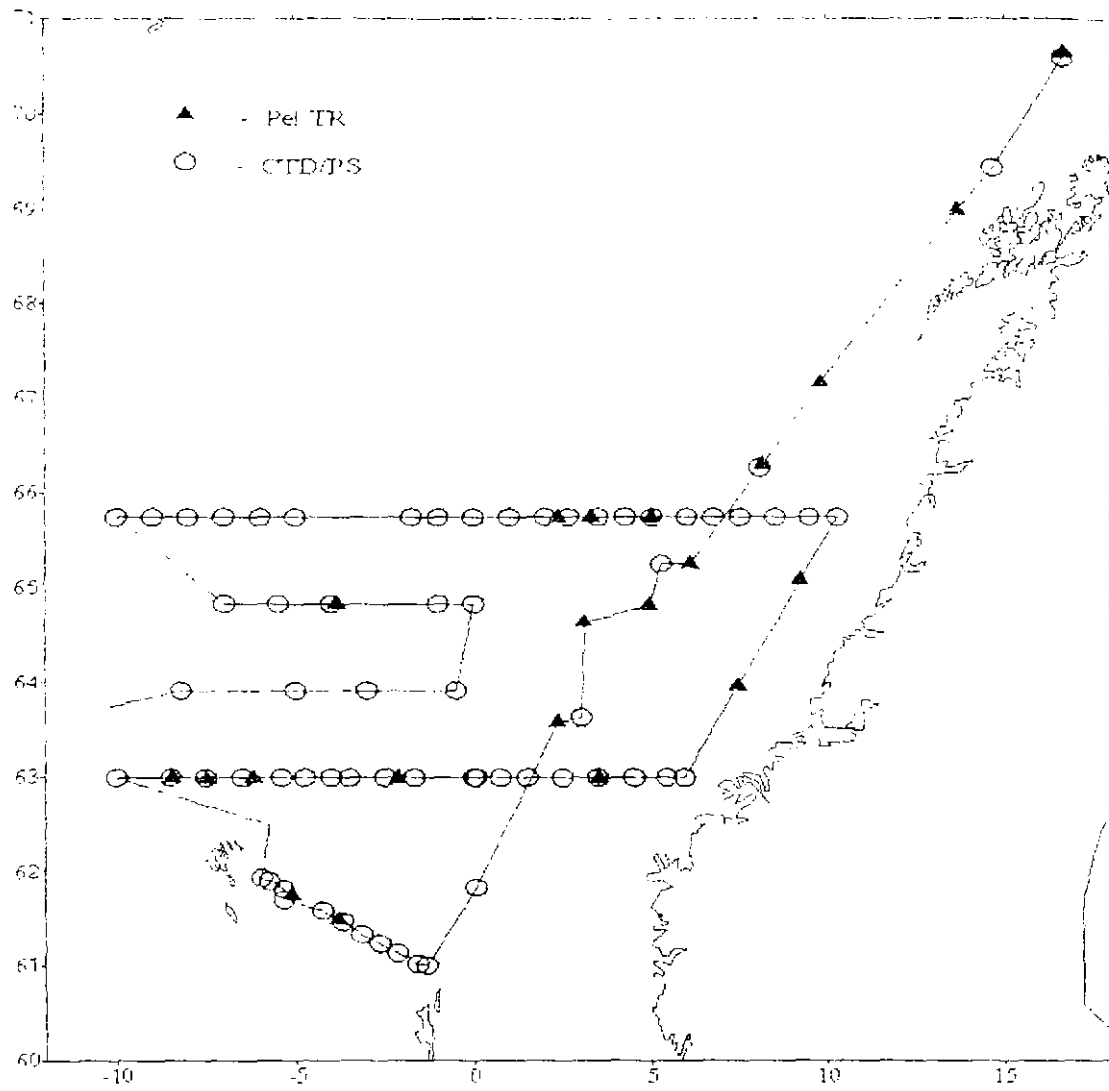
Fig. 88 Survey transects, trawl and CTD stations R/V "Fr. Nansen" during 03.06-22.06.1999.
