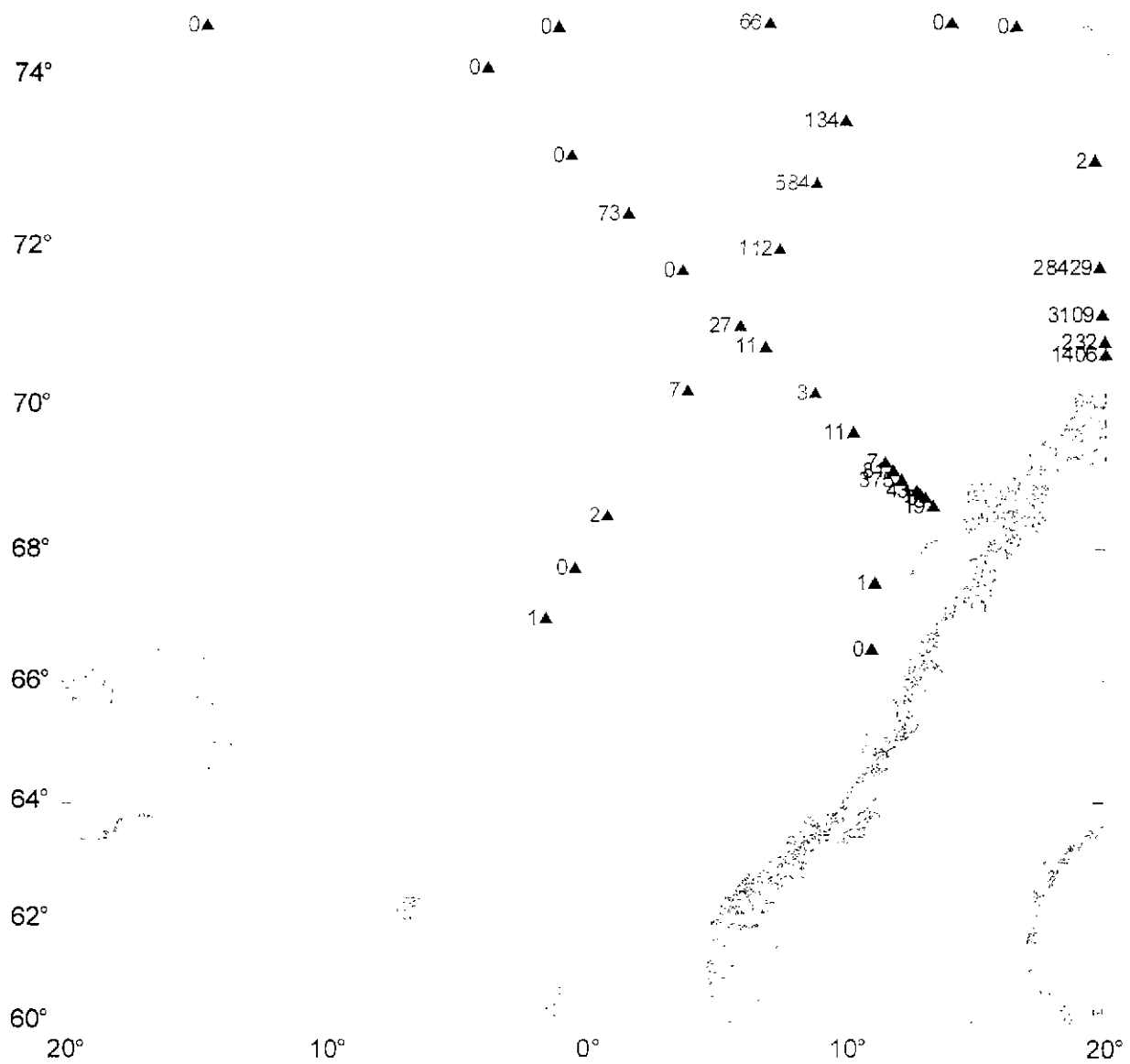
Figure 30. Herring catch in numbers taken by the RV Johan Hjort during the period 15.06-06.07, 1999.
