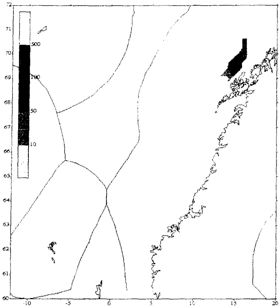
Fig. 29. Distribution of herring in the Norwegian Sea, map of Sa values, FF "F.Nansen" 03.06-22.06. 1999,
