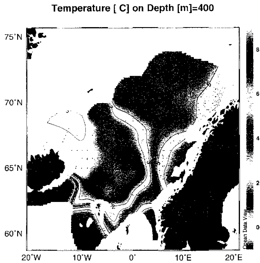
Figure 20. Temperature and salinity at 400 m depth, April - June 1999
