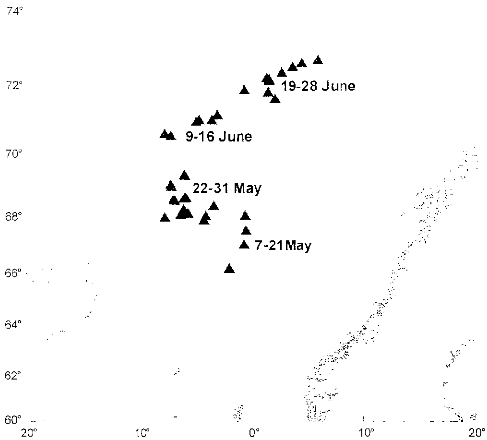
Figure 32. Positions and dates of herring samples obtained from Faroese and Icelandic fishing vessels.
