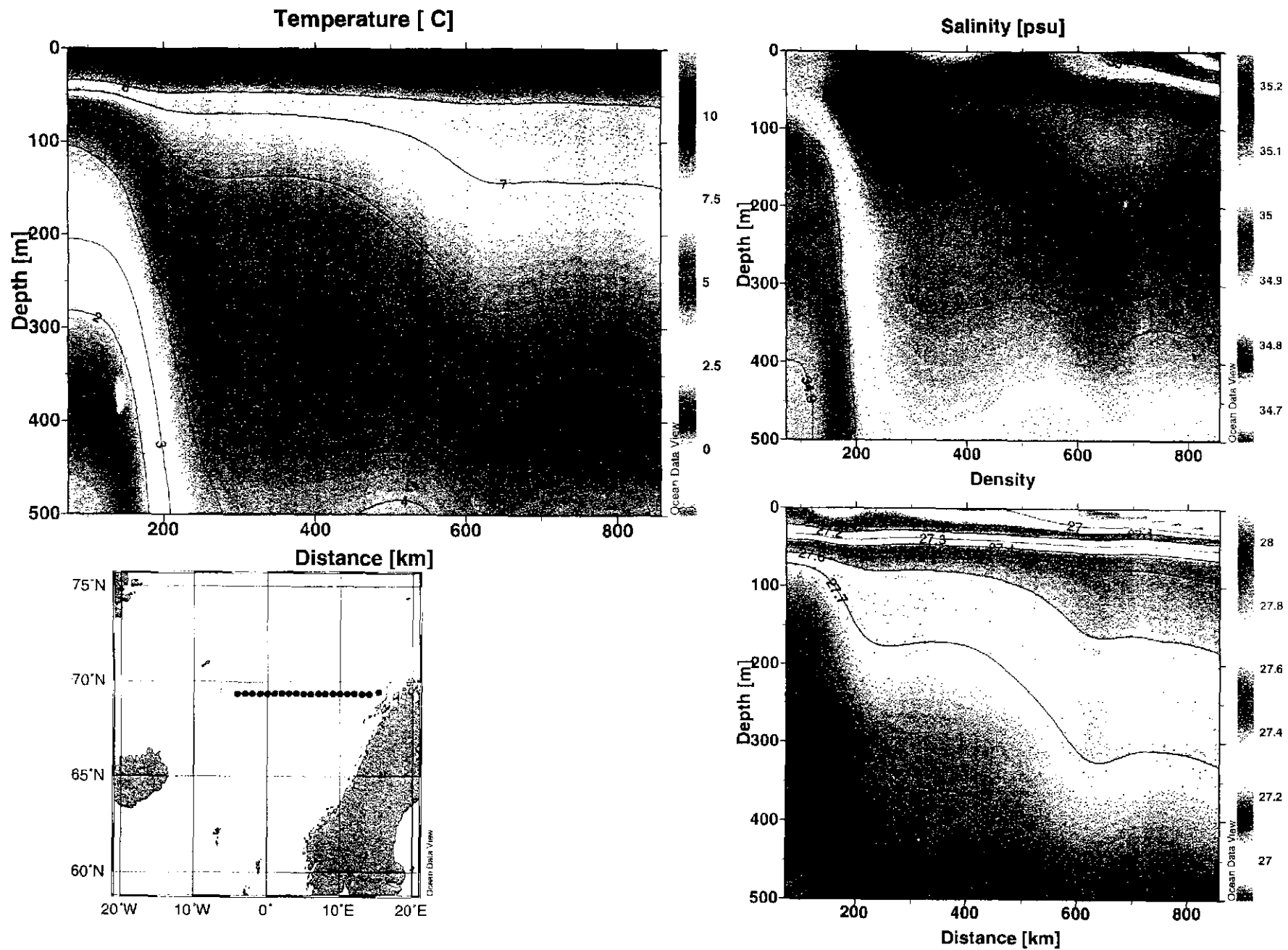
Figure 14. Temperature and salinity along 69°20'N in July 1999
