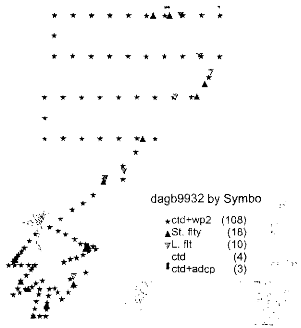
Figure 2. Cruise tracks of RV Magnus Heinasson during the international acoustic survey on Norwegian spring spawning herring in April-May 1999.
