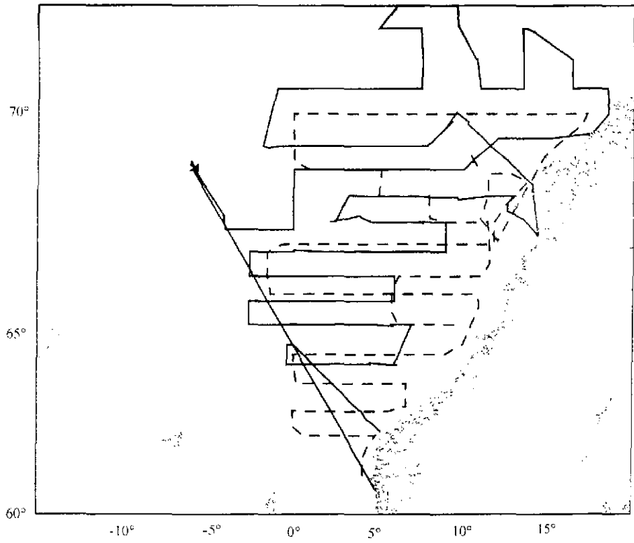
Figure 1. Cruise tracks of the RV G.O Sars (whole line) and the FRV Walther Herwig III (stippled line) during the international acoustic survey on Norwegian spring spawning herring in April-May 1999.
