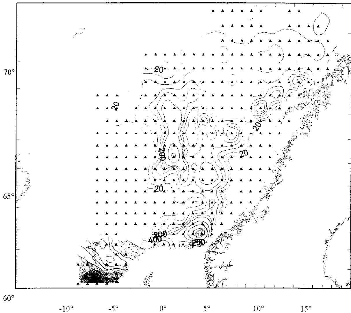
Figure 35. Distribution of blue whiting in May 1999 as measured by the RV Árne Fríðriksson, the RV G.O.Sars, the RV Magnus Heinason and the RV Walther Herwig III during the international coordinated herring survey.
