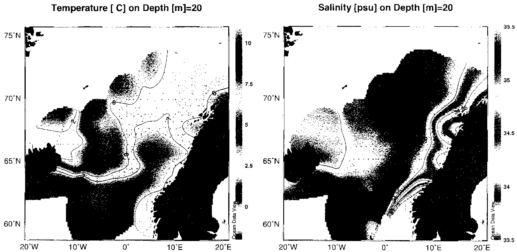
Figure 15. Temperature and salinity at 20 m depth, April - June 1999
