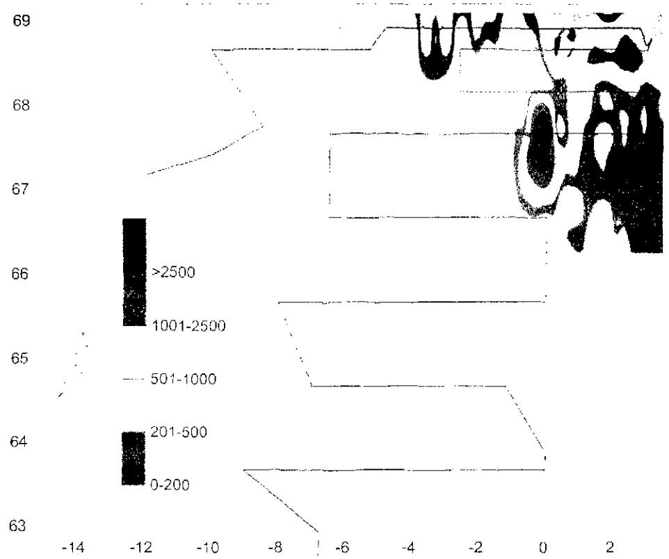
Figure 3. Cruise tracks of the RV Árni Fridriksson during the international acoustic survey on Norwegian spring spawning herring in April-May 1999. Isolines are Sa values of herring.
