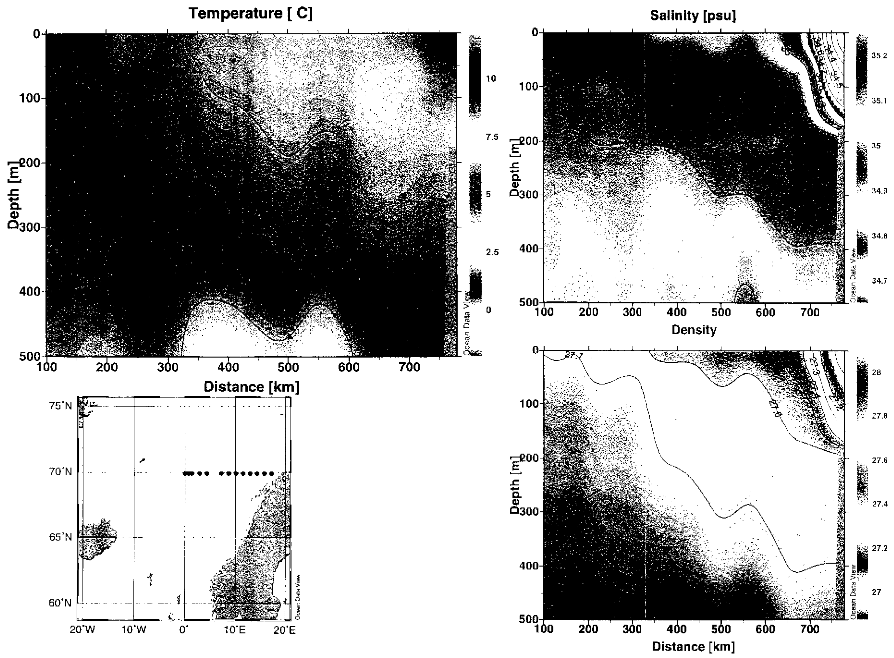
Figure 13. Temperature and salinity along 70° N in May 1999
