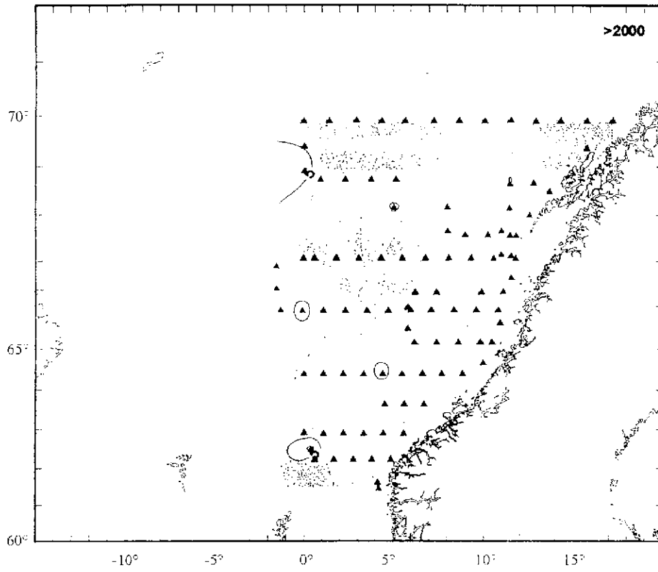
Figure 25. Zooplankton biomass in size fraction >2000 \mu\text{m} [ \text{g dw} \cdot \text{m}^{-2} ] (200-0m) April-June 1999.
