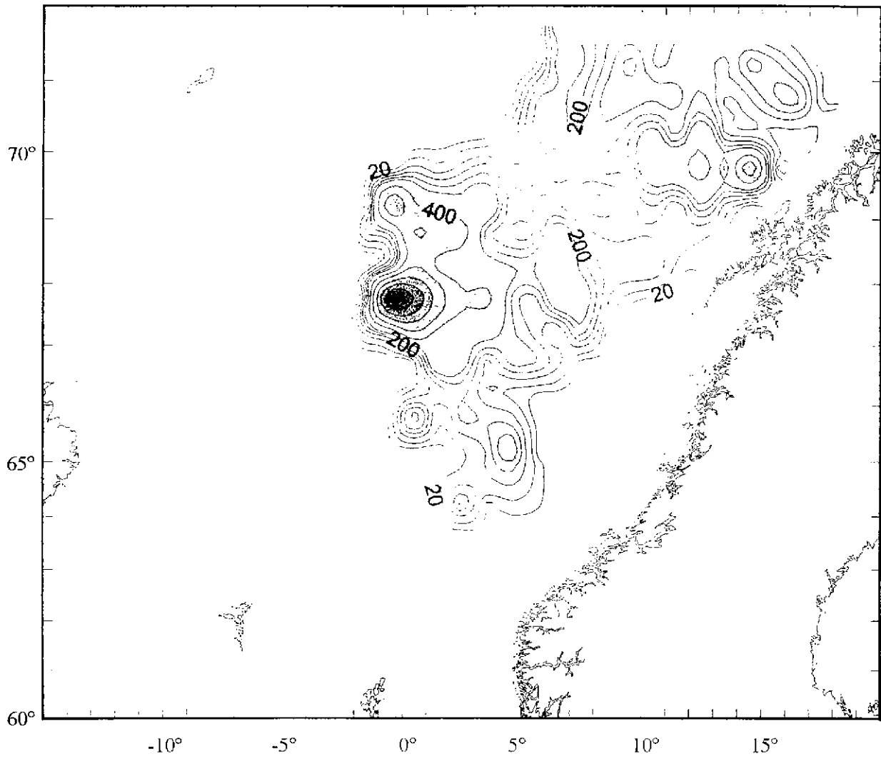
Figure 28. Distribution of Norwegian spring spawning herring in May 1999 as measured by the RV Árne Fridriksson, the RV G.O.Sars, the RV Magnus Heinason and the RV Walther Herwig III during the international coordinated herring survey.
