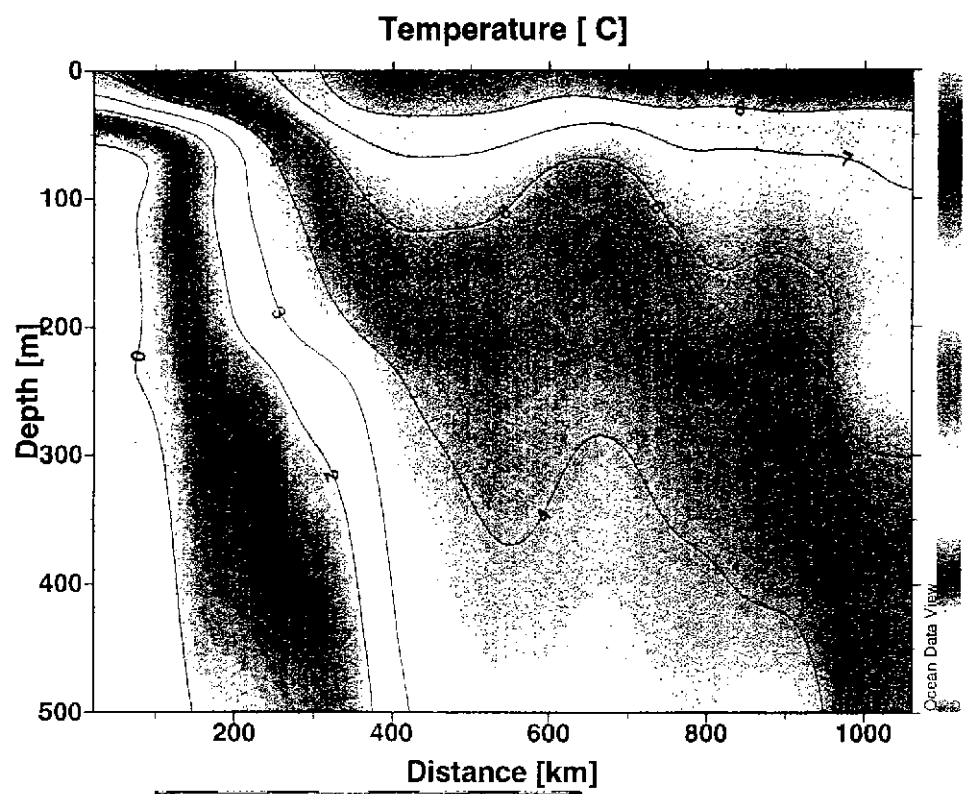
Figure 12. Temperature and salinity along 69°20'N in July 1998
