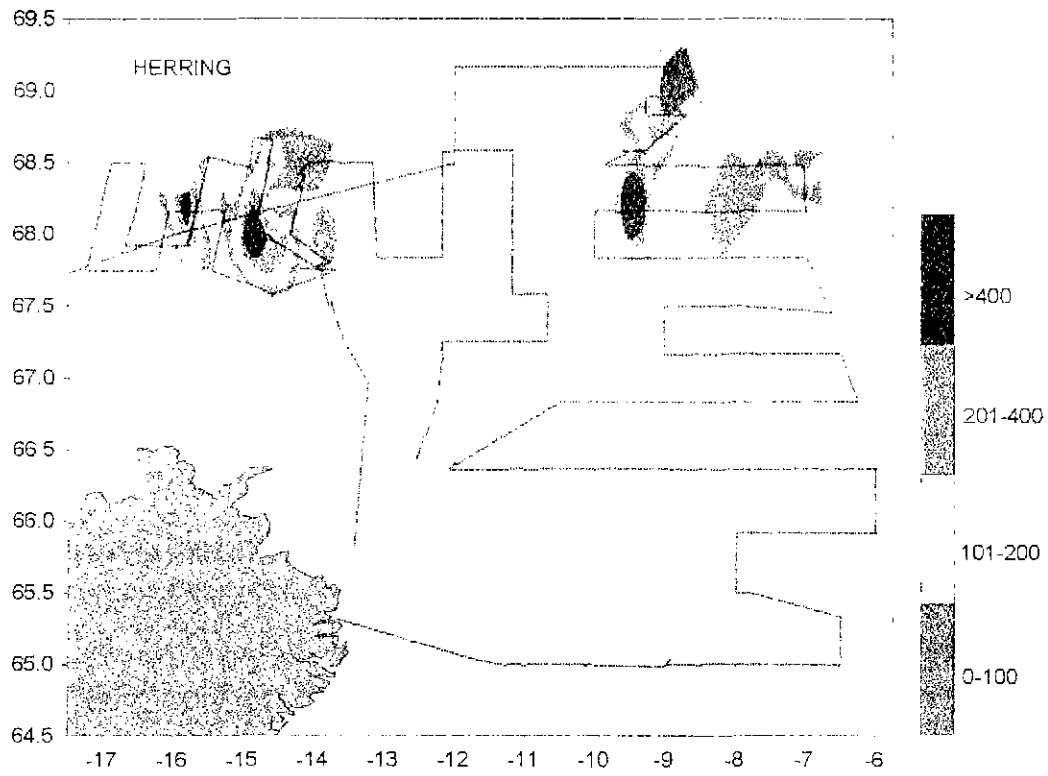
Figure 4. The observed distribution and relative density ( S_A -values) of herring during 22 June - 06 July 1999.
