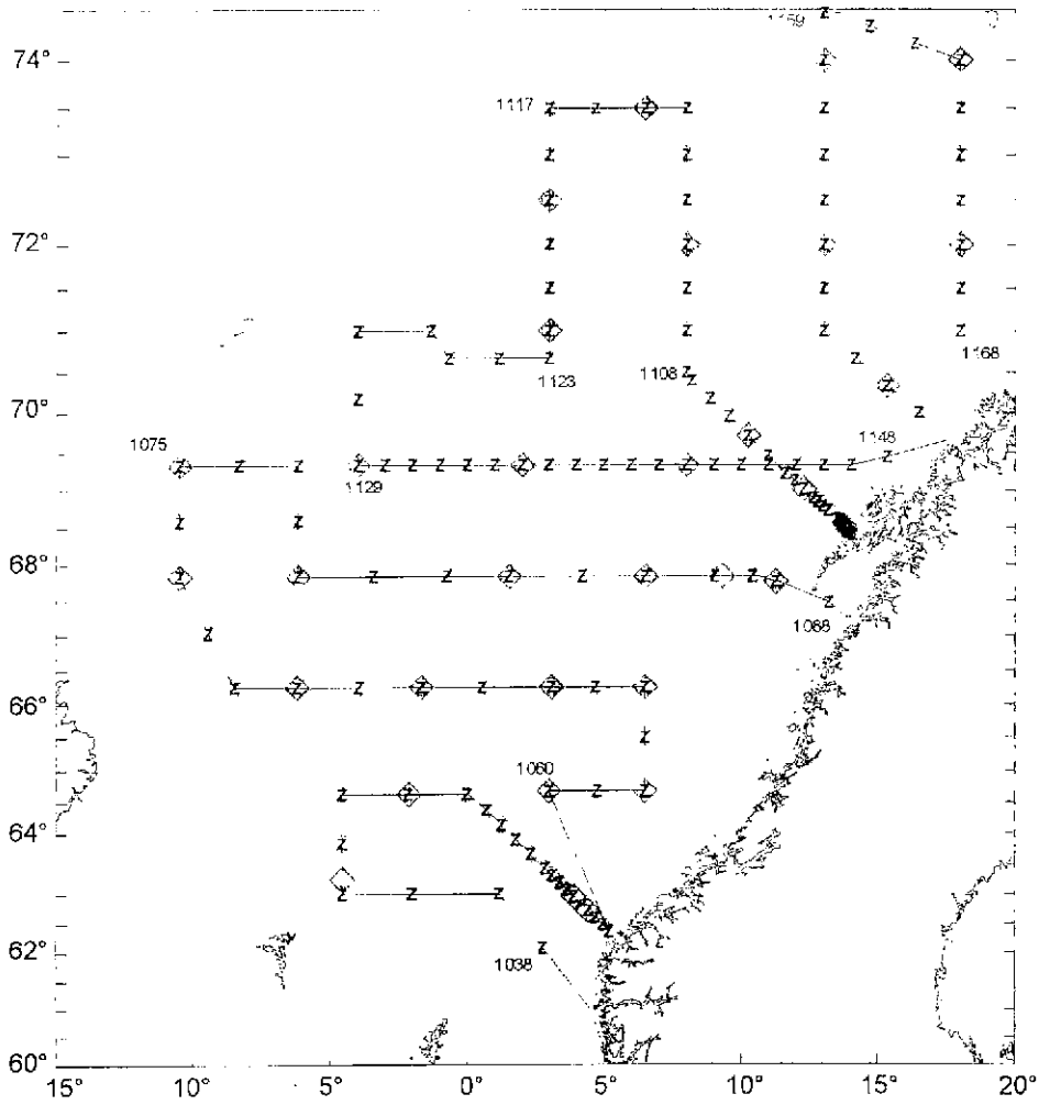
Figure 9. Cruise track of RV G.O.Sars 21.07-22.08, 1999, Z = CTD, \square = WP-2, square = Mocness.
