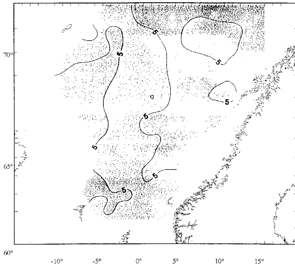
Figure 26. Zooplankton biomass [ \text{g dw} \cdot \text{m}^{-2} ] (200-0m) July-August 1998.
