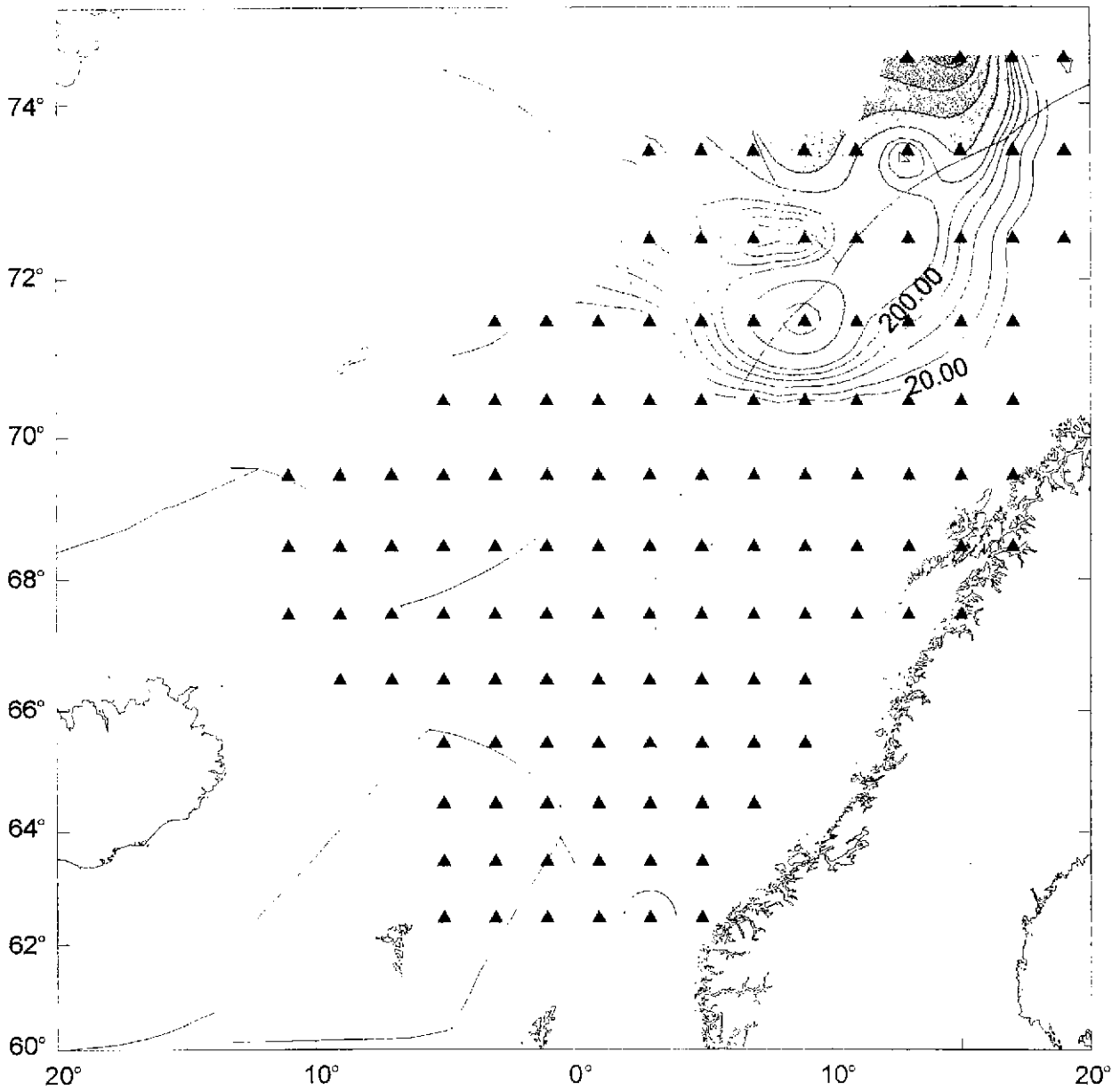
Figure 31. Herring distribution as observed by the RV G.Osars during the period 21.07-22.08 1999. Black triangles indicate squares with Sa values.
