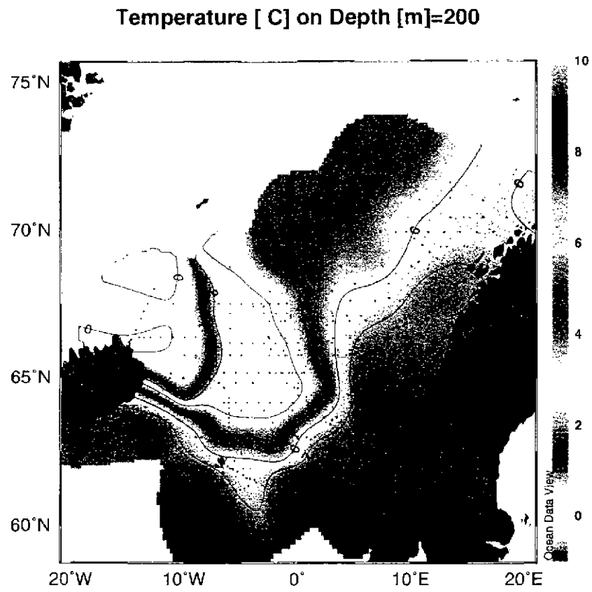
Figure 18. Temperature and salinity at 200 m depth, April - June 1999
