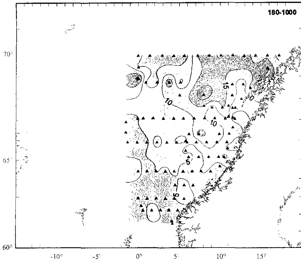
Figure 23. Zooplankton biomass in size fraction 180-1000 \mu\text{m} [ \text{g dw}\cdot\text{m}^{-2} ] (200-0m) April-June 1999.
