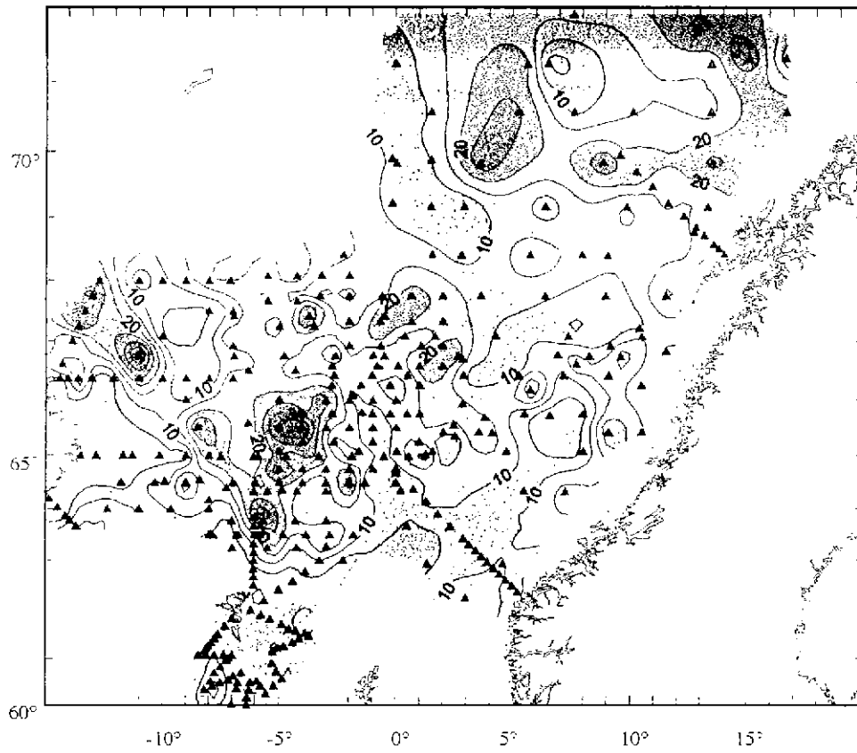
Figure 21. Zooplankton biomass [g dw·m -2 ] (200-0m) April-June 1998
