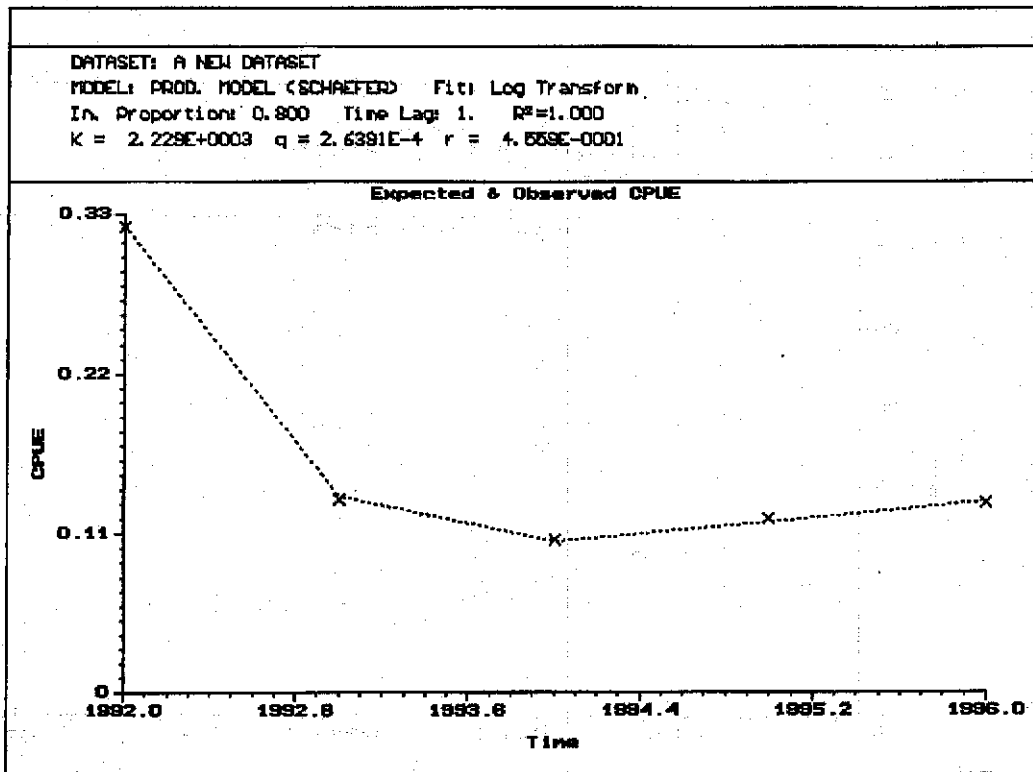
Figure 11.4 Fit of Schaefer production model to CPUE data from French Trawl fleet (directed trips only) - ICES Sub-area VI.
