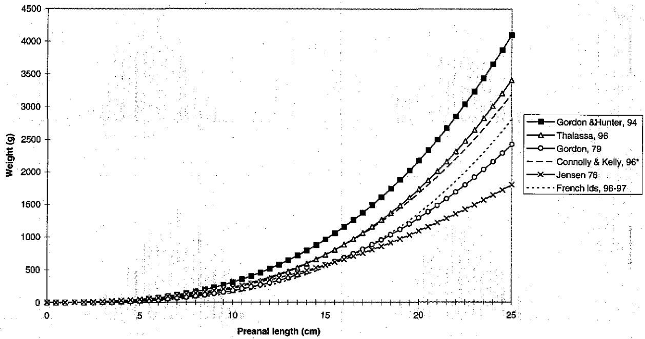
Figure 12.4. Length weight relationships from six different datasets. * : pre-anus length instead of pre-anal fin length.
