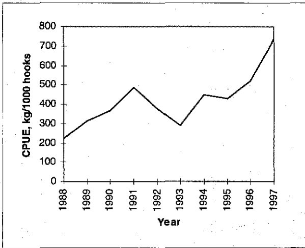
Figure 9.5 TUSK in Division Va. CPUE of Icelandic longliners.
