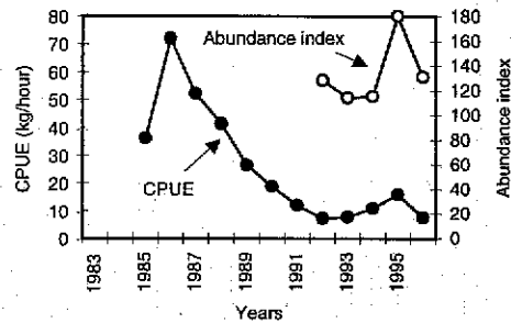
Figure 8.3 Blue ling in Division Vb. CPUE from the French trawler fleet and abundance indices from a multiplicative model using selected vessels from the same fleet.
