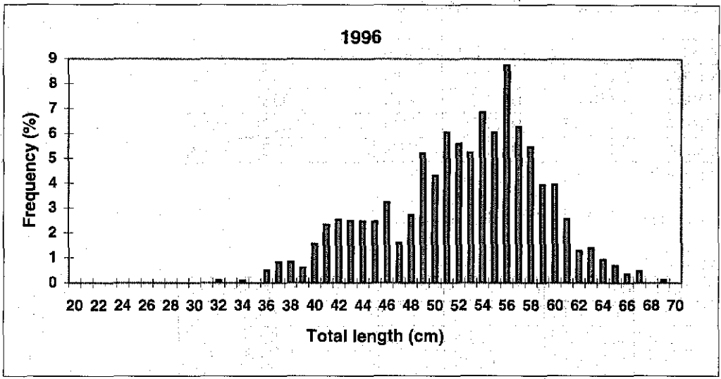
Figure 11.1. Length distribution of French landings of Orange Roughy in 1996
