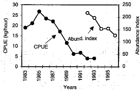
Figure 8.4 Blue ling in Sub-Area VI. CPUE from the French trawler fleet and abundance indices from a multiplicative model using selected vessels from the same fleet.
