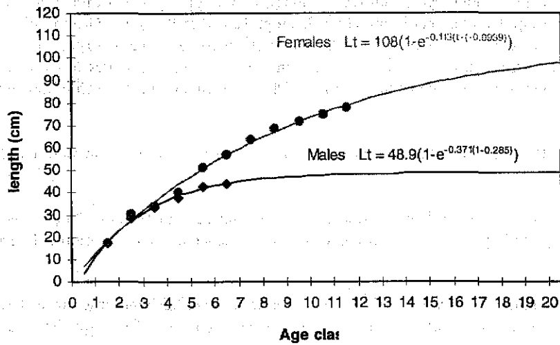
Figure 15.5.-Grwoth curves of P. blennoides by sex in ICES Division VIIIc and IXa. 1996
