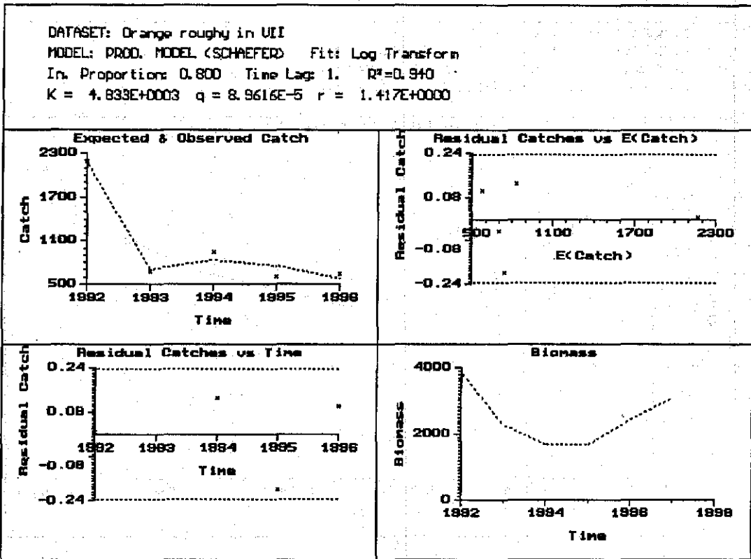
Figure 11.9 Residual plots of expected and observed catch and population numbers over time.
