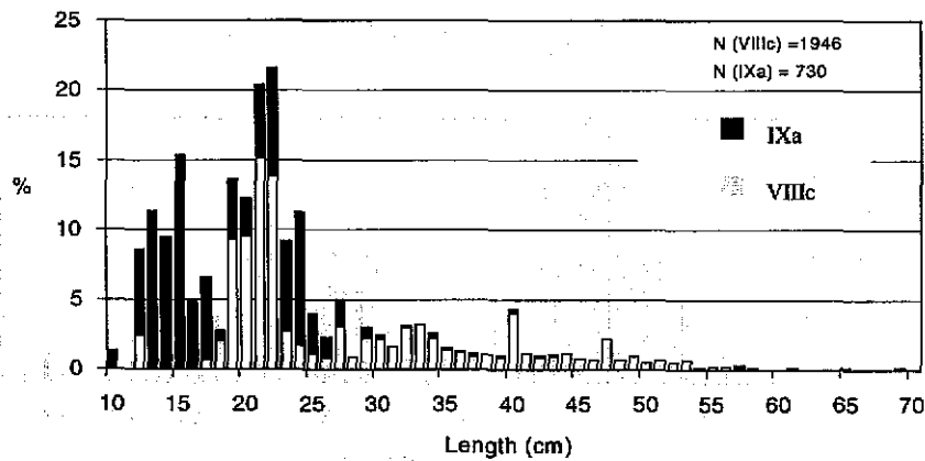
Figure 15.3 - Length composition of P. blennoides catches by the commercial trawler fishery.(1 st quarter 1997), in ICES Division VIIIc and IXa.
