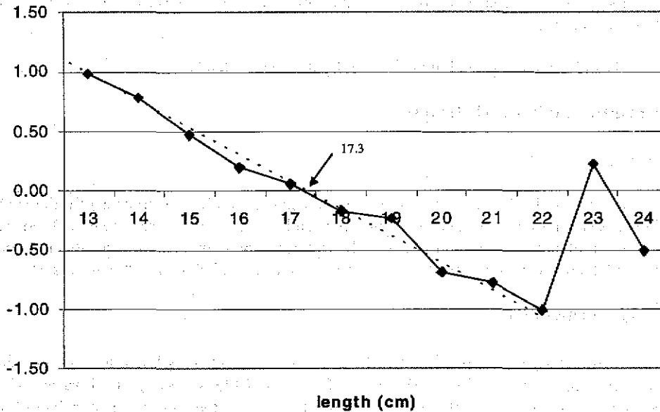
Figure 15.6. First mode of the small specimens (<25 cm) in Demersal research survey "DEM96", defined by Bhattacharya's method, in ICES Division VIIIc and IXa. 1996
