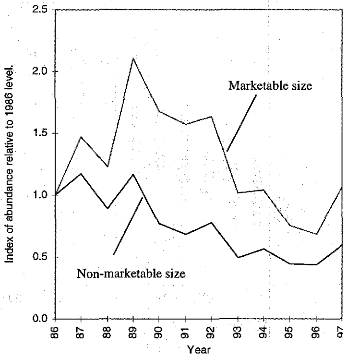
Figure 9.6 TUSK in Va. Index of abundance from the annual Icelandic groundfish survey in March.
