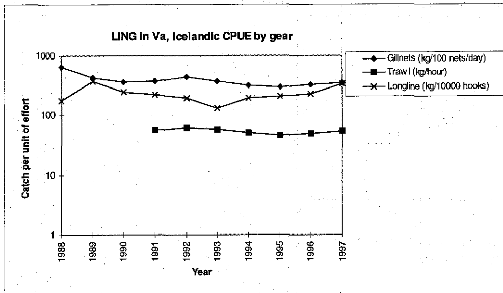
Figure 7.7 LING in Va. Icelandic catch per unit of effort by gear. Note the logarithmic scale on the CPUE axis.
