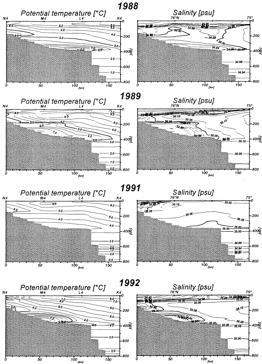
Fig.2 Potential temperature [ ^{\circ}\text{C} ] and salinity [psu] distributions at the northern part of transect 15^{\circ}\text{E} .
