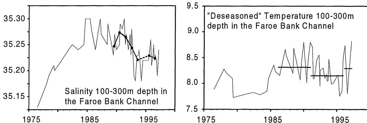
Fig. 2. Salinity (left) and temperature (right) averaged over the 100 - 300 m layer in the middle of the Faroe Bank Channel (white circle on Fig. 1) based upon CTD observations. Temperature has been "deseasoned" by subtracting the typical seasonal variation. Filled circles connected by bold lines on left graph show annual averages of salinity while thick horizontal lines on right graph show temperature over two 5-year periods and the period 1996 - Feb. 1997.
