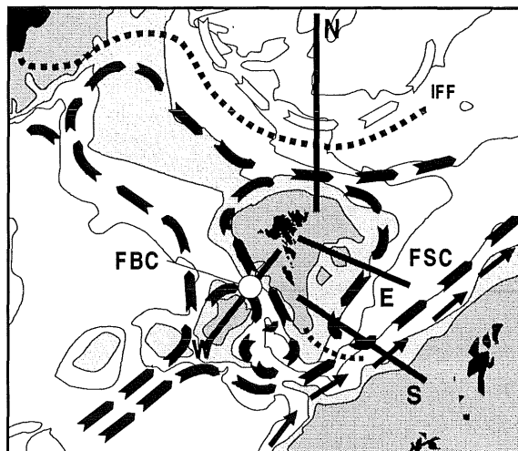
Fig. 1. The bottom topography around the Faroe Islands is indicated with the shallow areas shaded. The main flow in the upper layers is by arrows and the Iceland-Faroe Front by a dotted curve. The four standard sections (N, E, S and W) are shown by thick lines and the white circle indicates the area in the Faroe Bank Channel from which the data in Fig. 2 originate.
