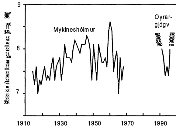
Fig. 3. Annually averaged coastal observations of sea surface temperature in the Faroes at two fairly close locations: Mykineshólmur 1914 - 1969 and Oyrargjógv 1991 - 1996.
