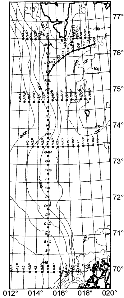
Fig. 1. Area of investigations in Norwegian - Barents Seas Confluence Zone. Transect "O" and northern part of Transect "15" - bold lines.
