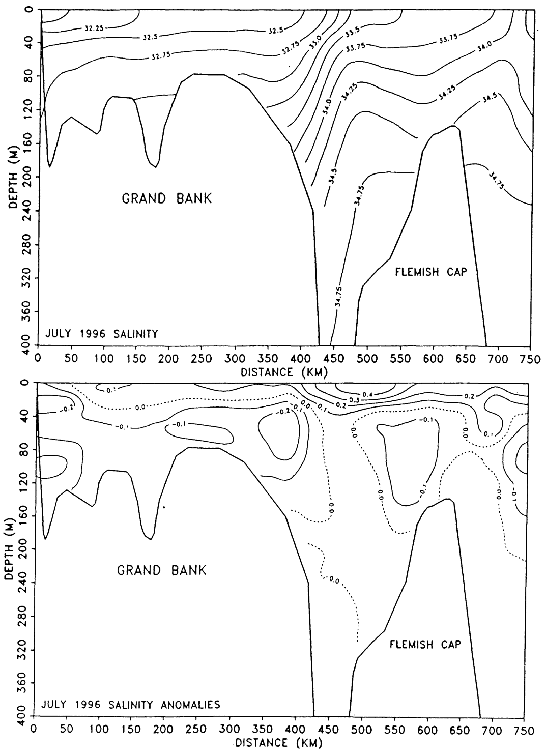
Fig. 9b The vertical distribution of salinity and salinity anomalies along the standard Flemish Cap transect for the summer (July) of 1996.
