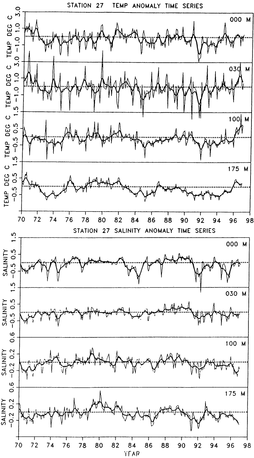
Fig. 11 Time series of monthly temperature and salinity anomalies at Station 27 at standard depths from 1970 to 1996. The heavy lines are the low-passed filtered time series.
