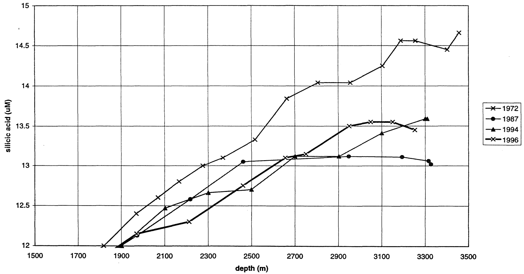
Silicic acid profiles S. Norw. Sea
