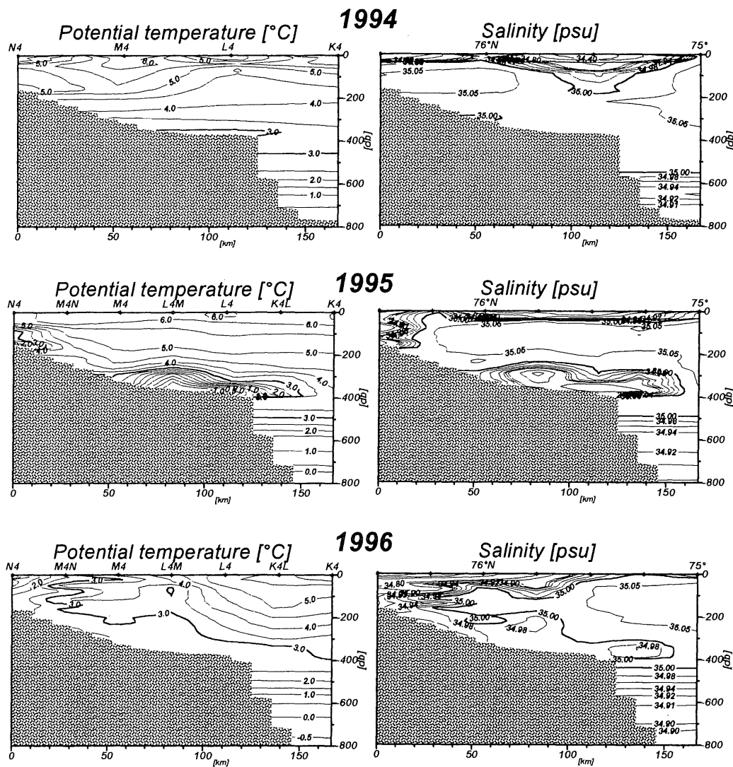
Fig. 2 cont'd Potential temperature [ ^{\circ}\text{C} ] and salinity [psu] distributions at the northern part of transect 15 ^{\circ}\text{E} .
