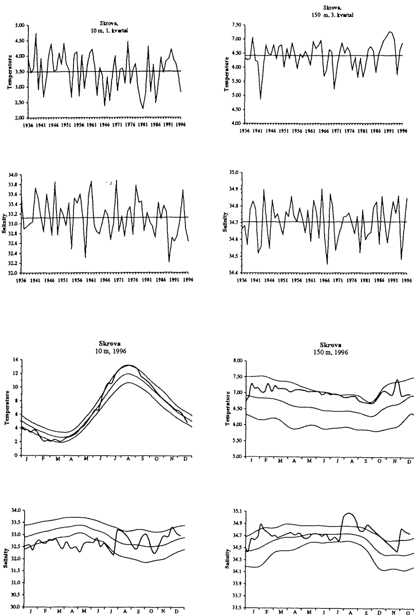
Fig 8. (Uppre panel) Time series of temperature and salinity for the period 1936 - 1996 at the fixed station "Skrova". The figure shows plots of means for the first quarter (Jan.-Mar.) at 10 m depth and of means for the third quarter at 150 m depth. (Lower panel) Seasonal trends of temperature and salinity at 10 m and 150 m depth at "Skrova". Seasonal mean values with standard deviation are also shown.
