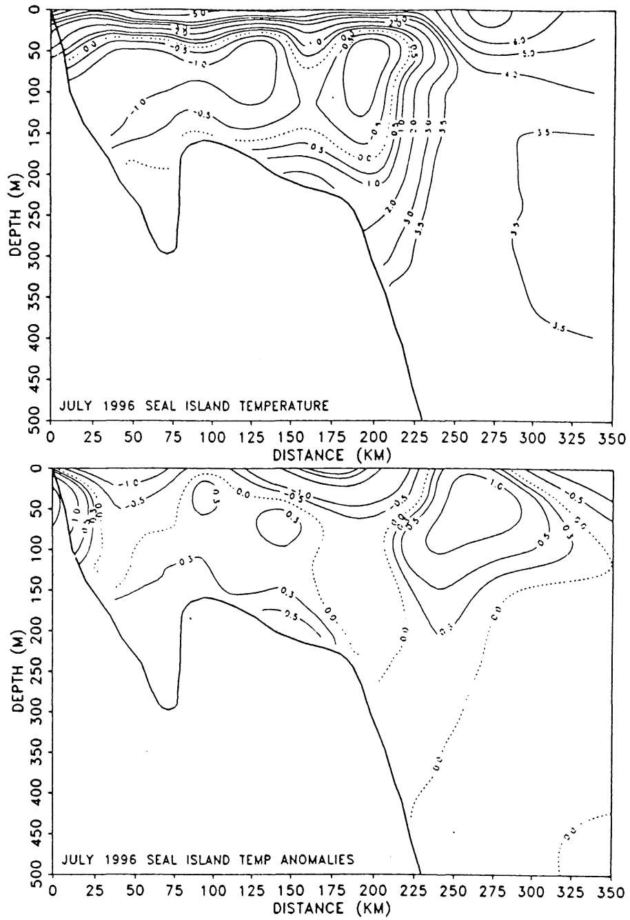
Fig. 7a The vertical distribution of temperature and temperature anomalies along the standard Seal Island transect for the summer (July) of 1996.
