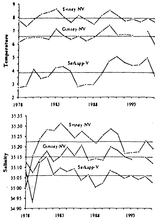
Fig. 5. Temperature and salinity, observed in July/August, in the core of the Atlantic water in the sections Svinøy-NW, Gimsøy-NW and Sørkapp-W, Averaged between 50 and 200 m depth.
