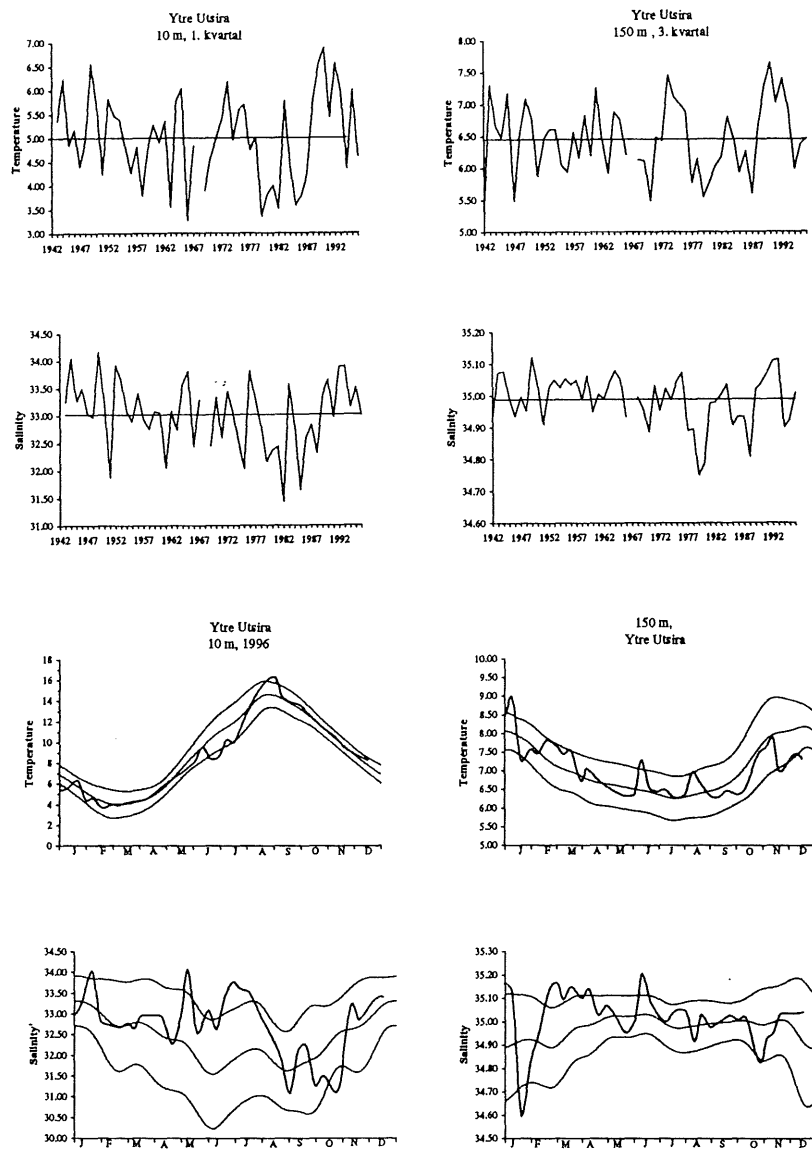
Fig 9. (Upper panel) Time series of temperature and salinity for the period 1942 - 1996 at the fixed station "Utsira". The figure shows plots of means for the first quarter (Jan.-Mar.) at 10 m depth and of means for the third quarter at 150 m depth.
