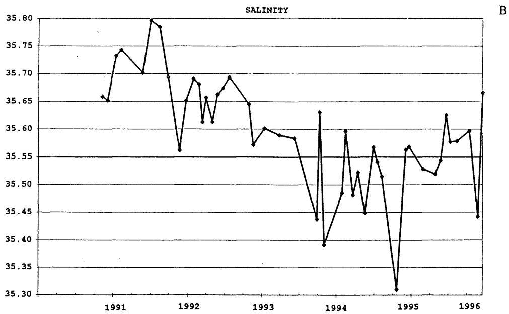
Figure 7. A: Temperature at 10 m depth at station 4. B: Salinity at 50 m depth at station 4 (Santander Section)
