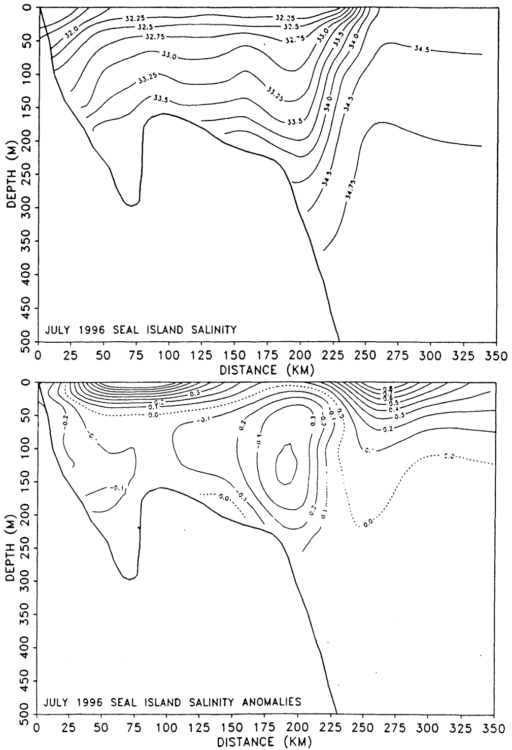
Fig. 7b The vertical distribution of salinity and salinity anomalies along the standard Seal Island transect for the summer (July) of 1996.
