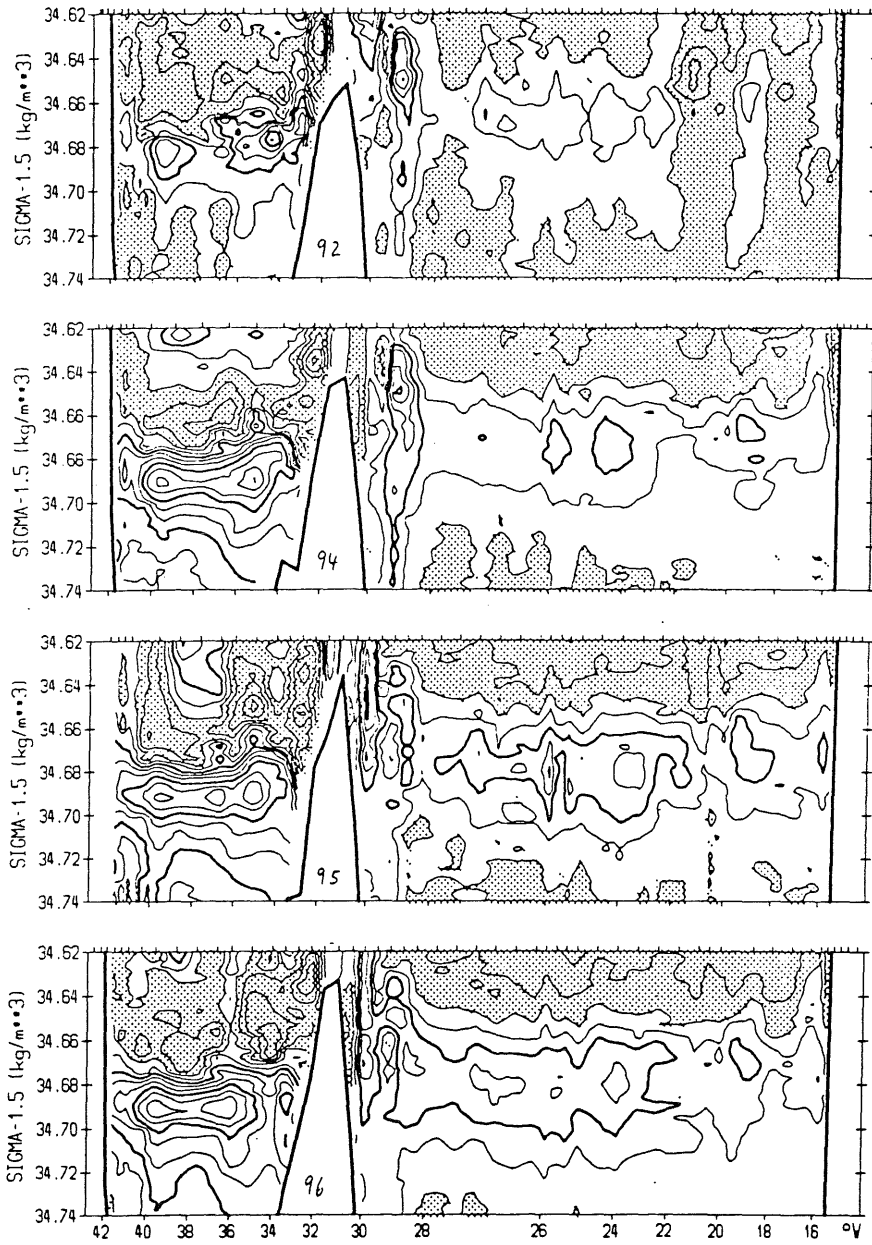
Fig 2 b) As in a), but for Salinity. Hatched: saltier against 1991. The density range covers the Labrador Sea Water (LSW). Agenda item 6: Progress in national and international projects
