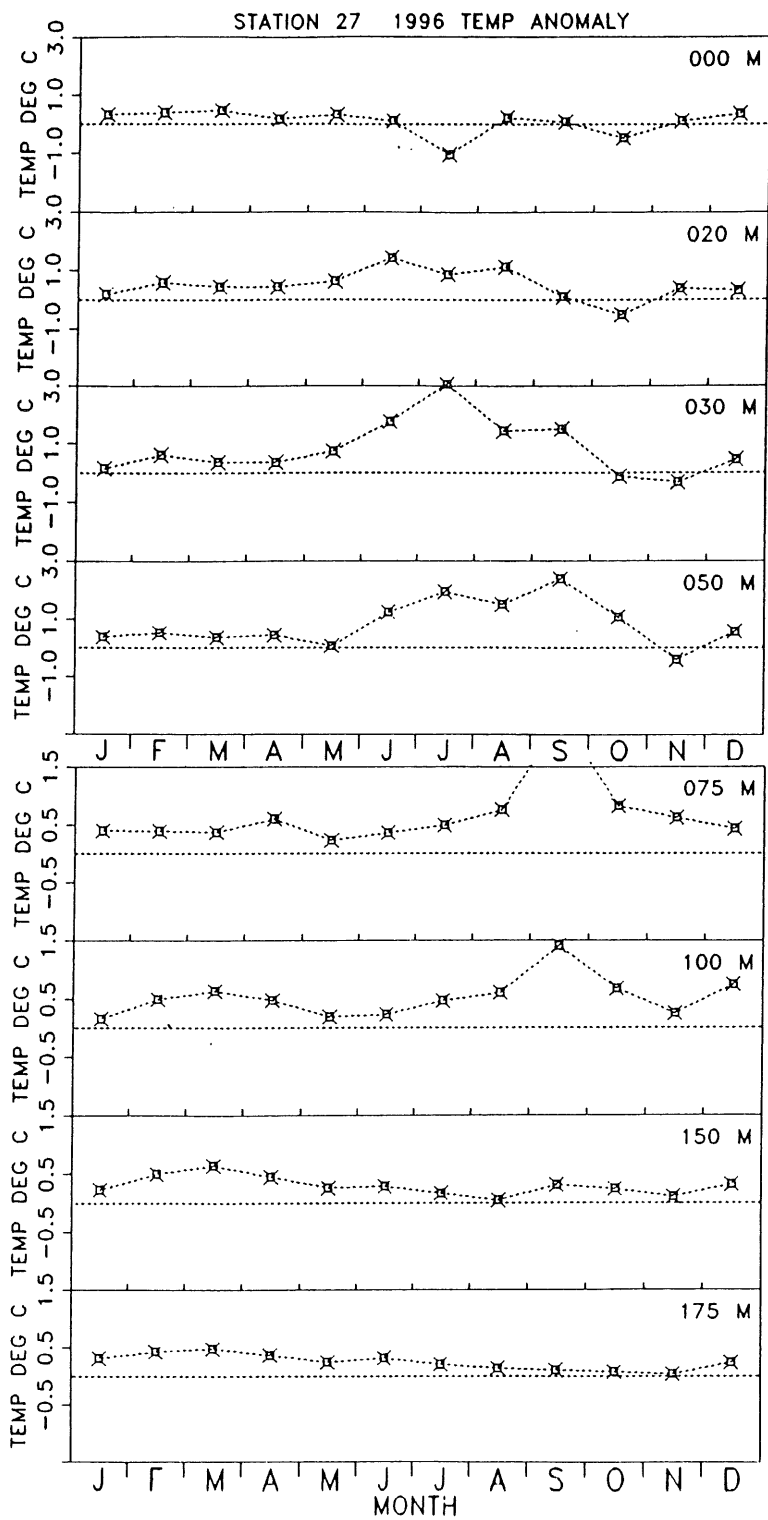
Fig. 10a Time series of the monthly temperature anomalies at Station 27 at standard depths during 1996.
