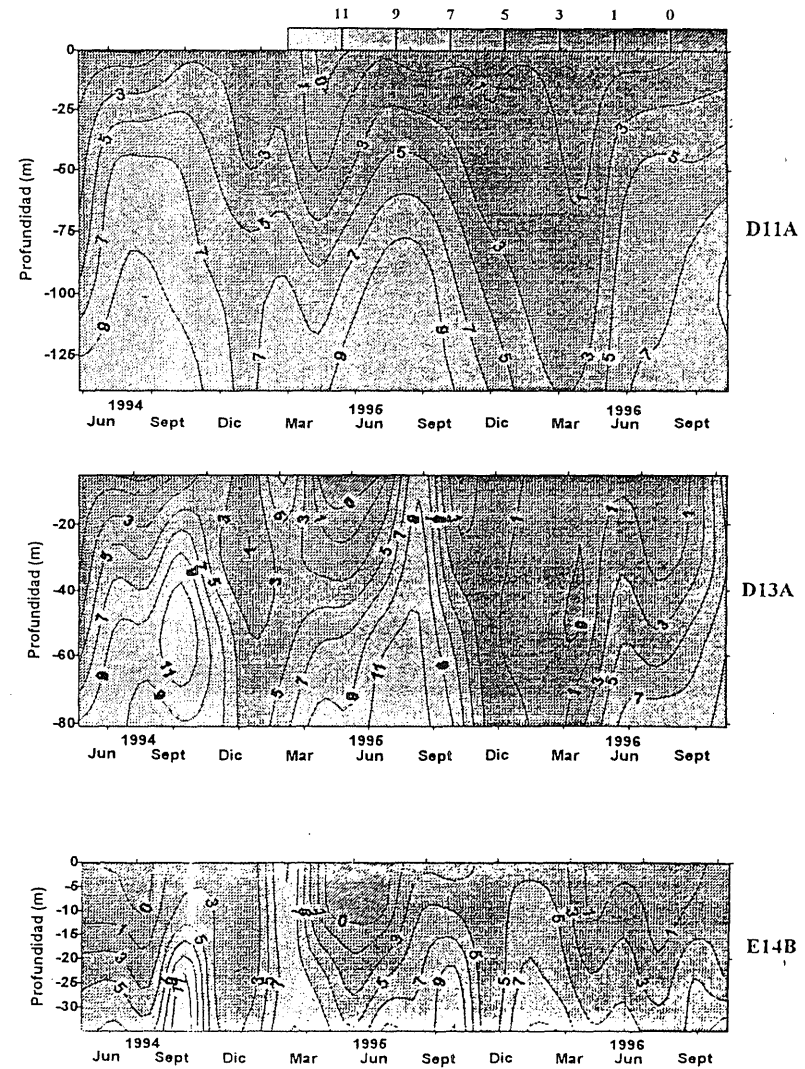
Figure 11. Nitrate distributions at stations 14b, 13a and 11a. (Vigo Section)
