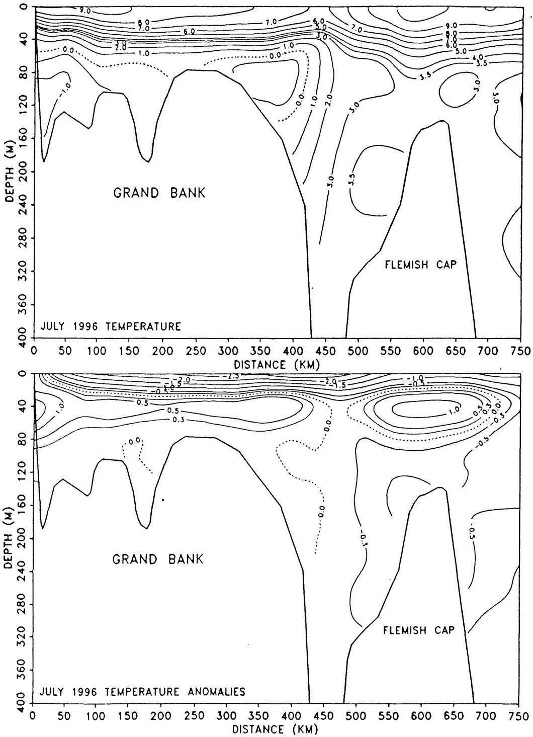
Fig. 9a The vertical distribution of temperature and temperature anomalies along the standard Flemish Cap transect for the summer (July) of 1996.
