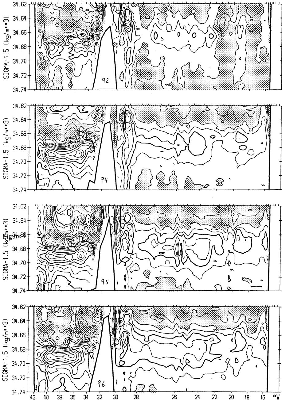
Fig. 2 a) Difference of Potential Temperatures against Sigma 1.5 along the WOCE A1E -Sections in 1992, 1994, 1995 and 1996 against 1991. Hatched: Warmer against 1991
