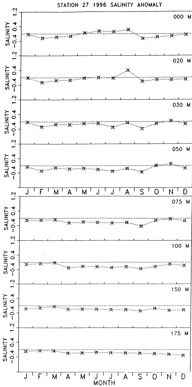
Fig. 10b Time series of the monthly anomalies at Station 27 at standard depths during 1996.
