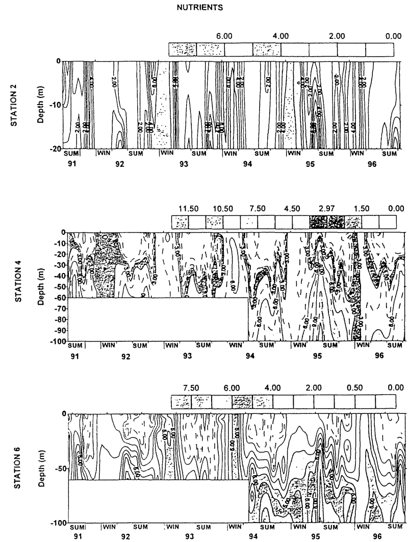
Figure 6: Nitrate distributions at stations 2, 4 and 6 (Santander Section).
