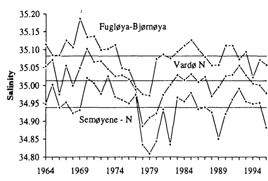
Fig. 2. Mean temperature and salinity between 50 and 200 m depth in the sections Fugløya-Bjørnøya, Vardø - N and Sem Islands - N. Observations from August/September, 1964 - 1996.
