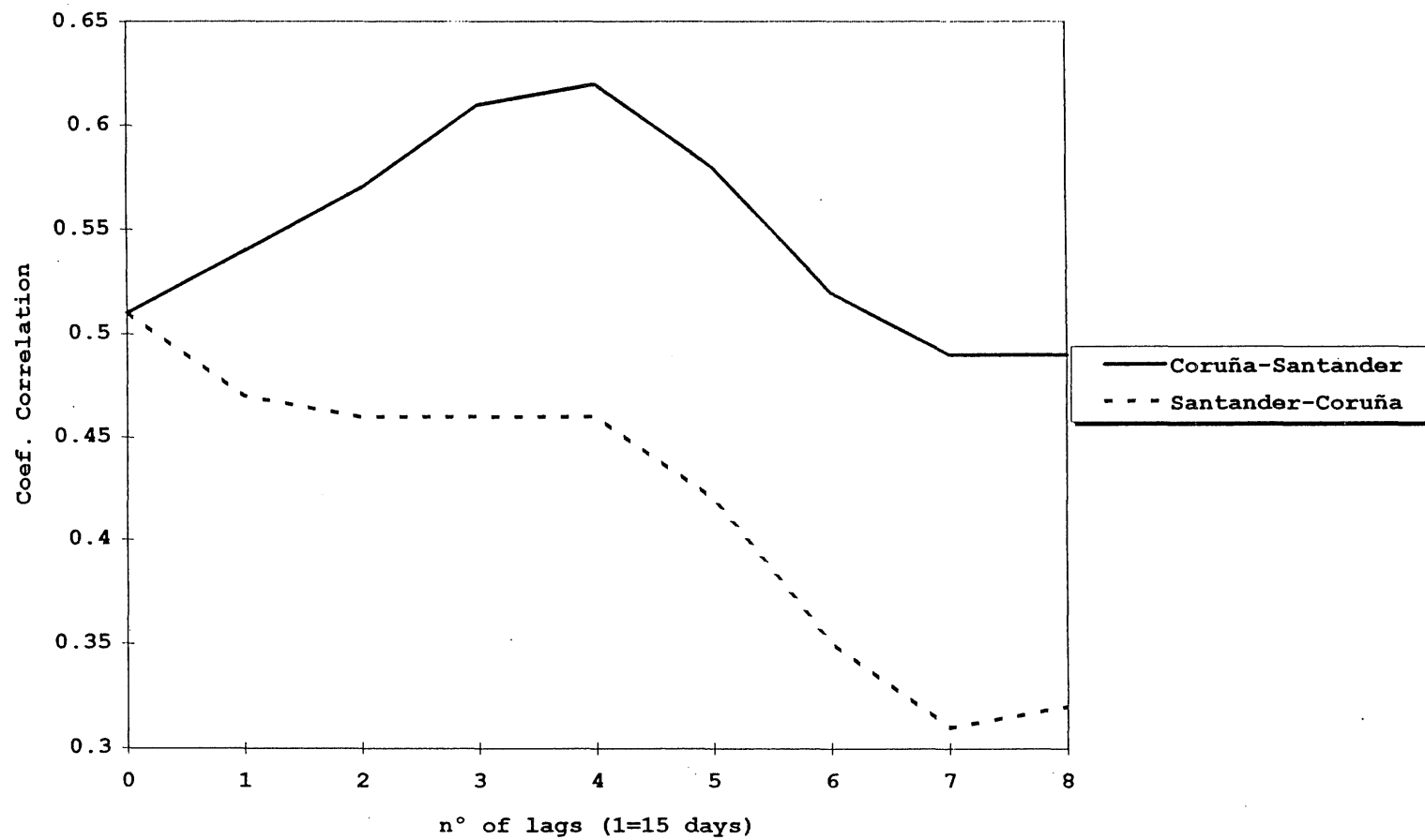
Figure 12. Correlation between salinity conditions at 70 m depth in La Coruña and Santander.
