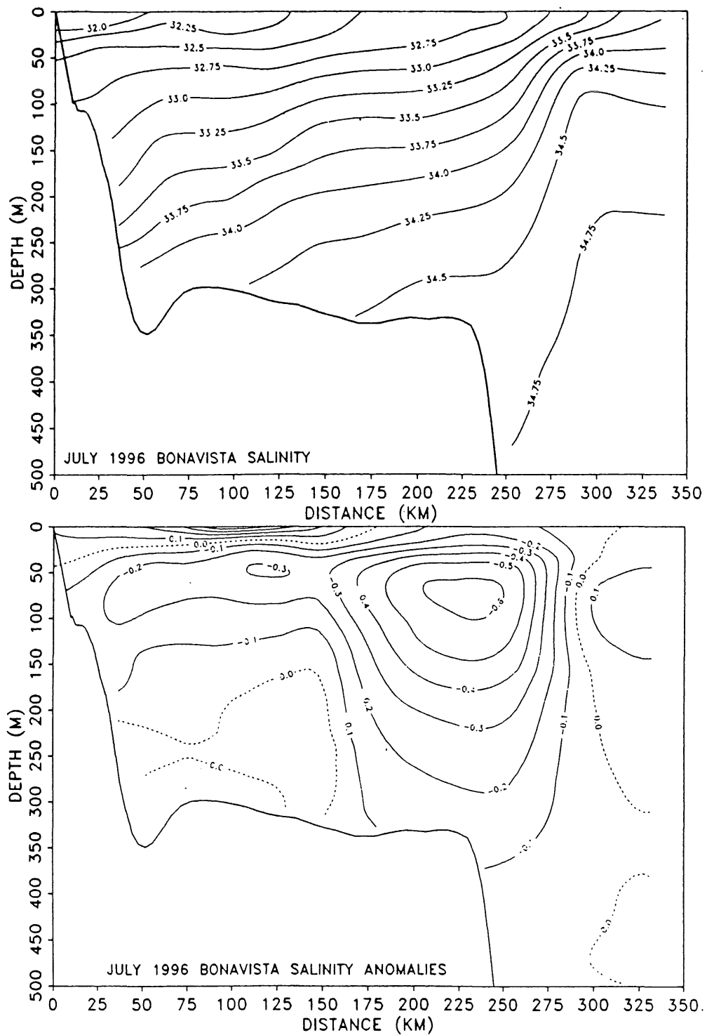
Fig. 8b The vertical distribution of salinity and salinity anomalies along the standard Bonavista transect for the summer (July) of 1996.
